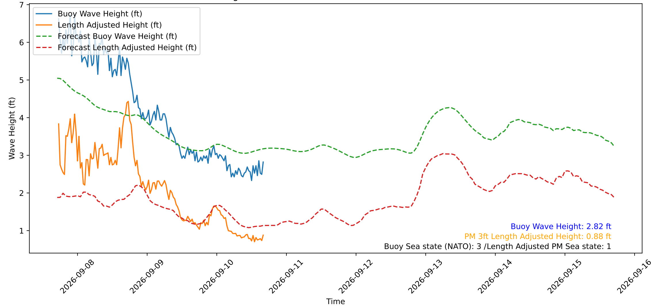
Wave Heights over Time for Red Beach at 2026-09-10 17:10:49
