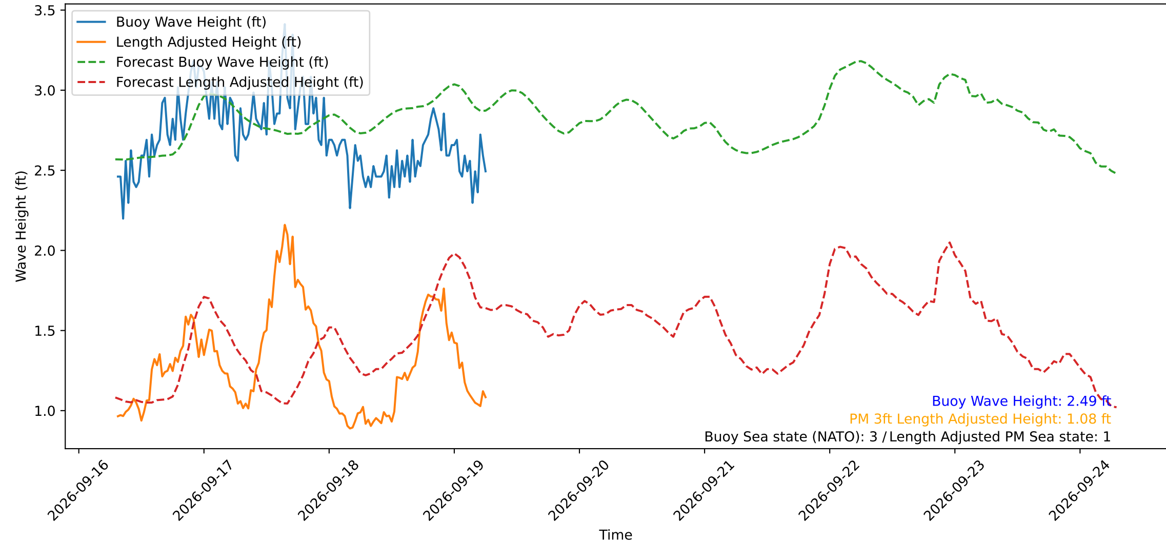
Wave Heights over Time for Red Beach at 2026-09-19 07:00:49
