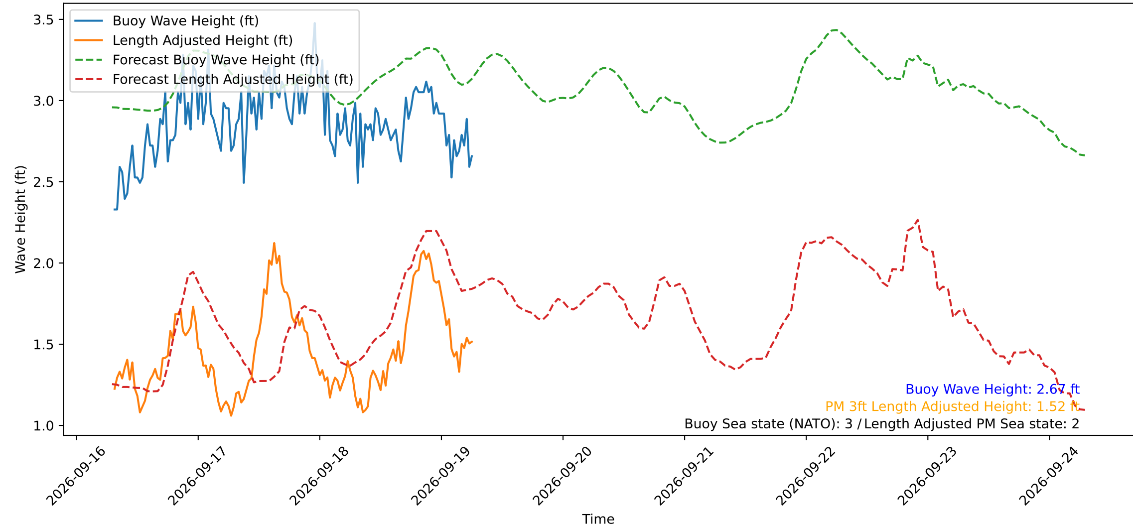
Wave Heights over Time for Green Beach at 2026-09-19 07:01:11
