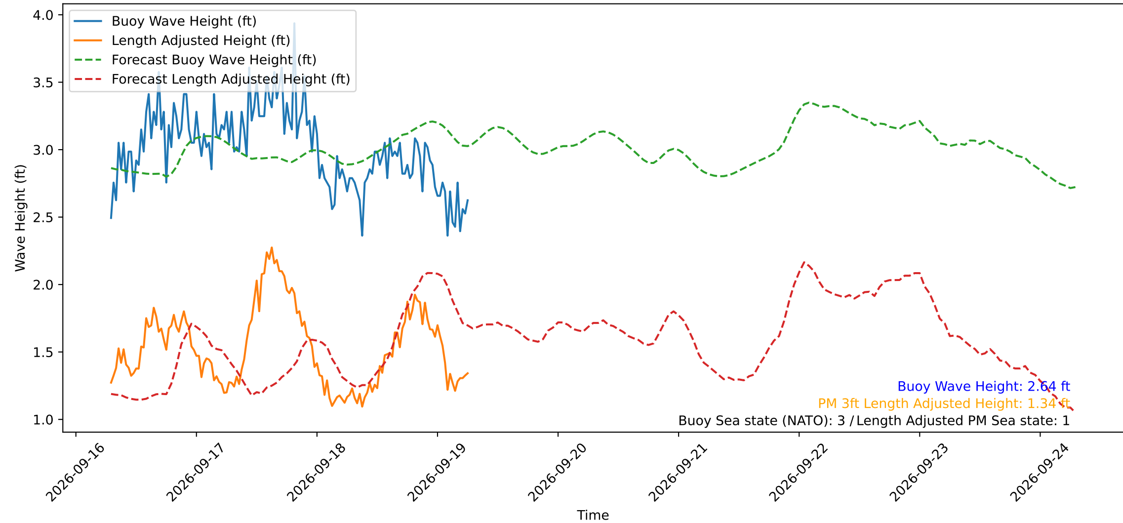
Wave Heights over Time for Oceanside Harbor at 2026-09-19 07:00:29
