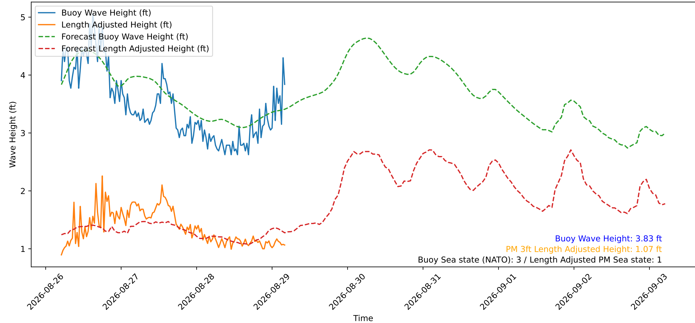
Wave Heights over Time for Red Beach at 2026-08-29 04:50:52
