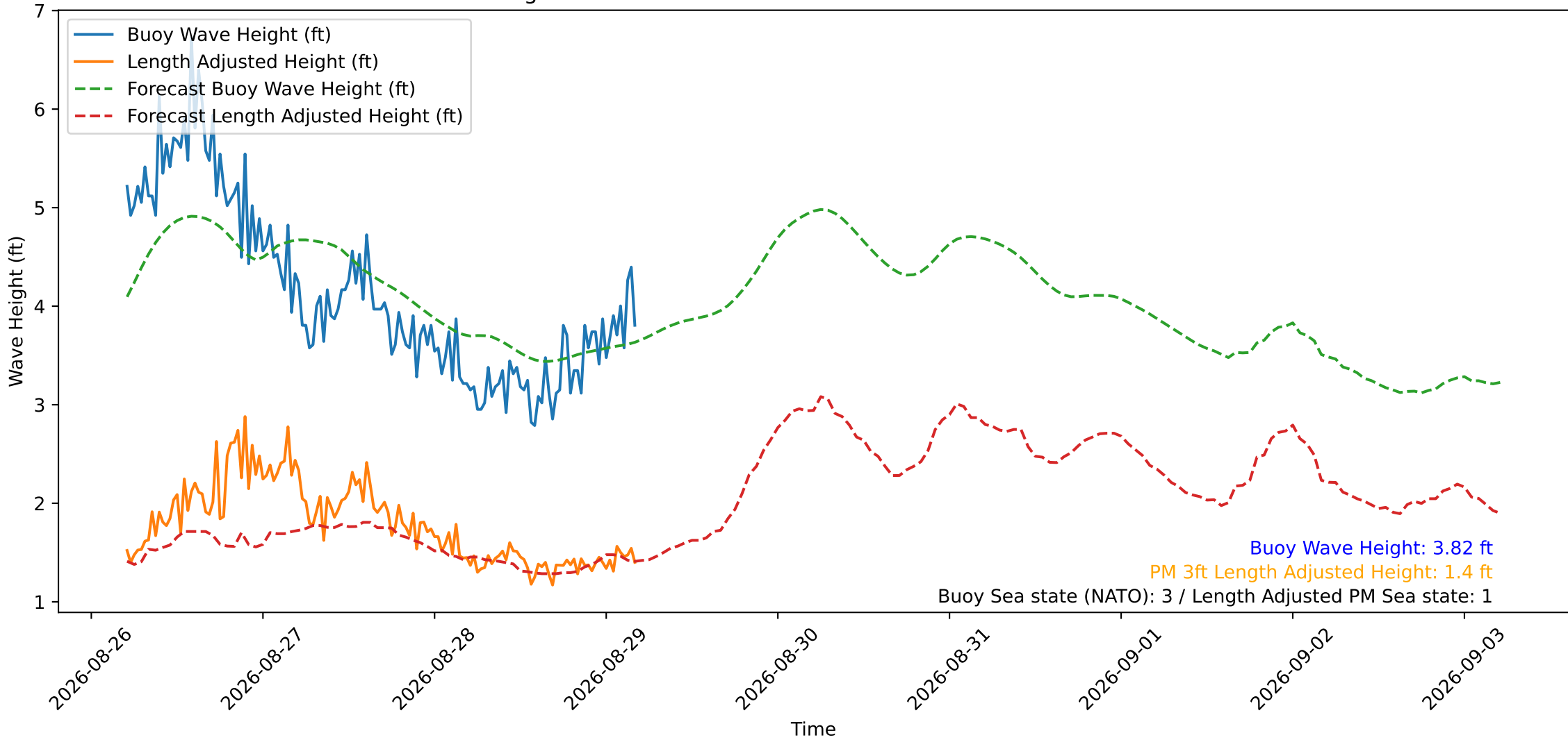
Wave Heights over Time for Oceanside Harbor at 2026-08-29 04:50:30
