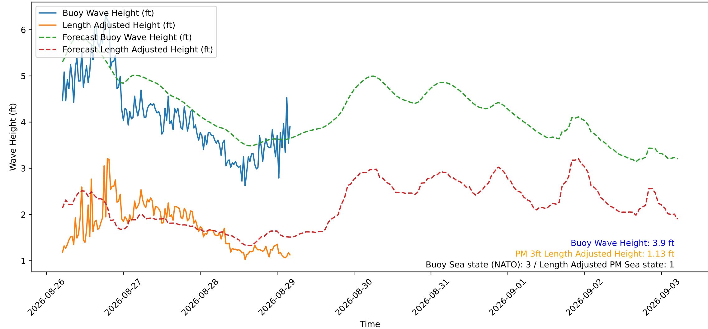
Wave Heights over Time for Green Beach at 2026-08-29 04:51:16
