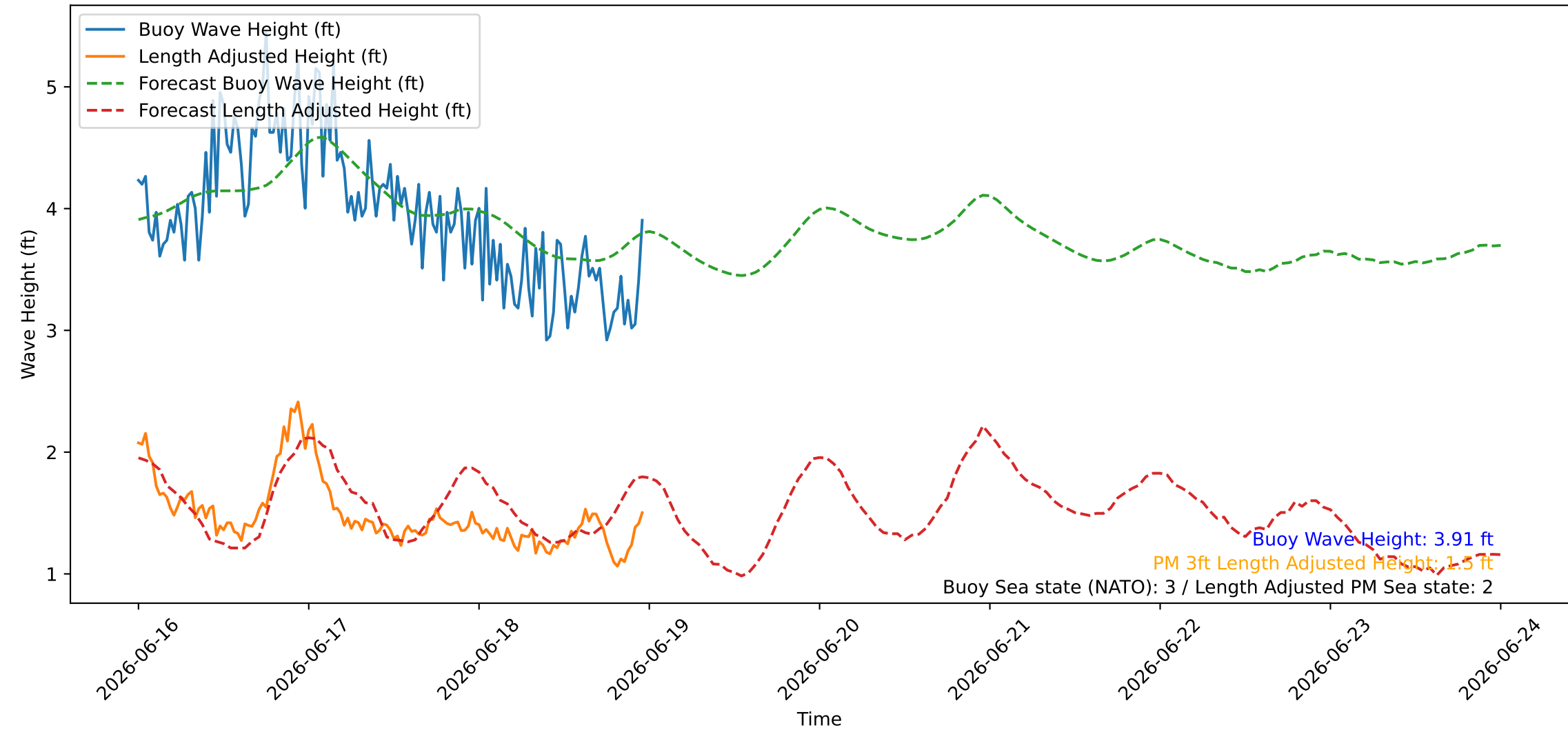
Wave Heights over Time for Oceanside Harbor at 2026-06-18 23:50:26
