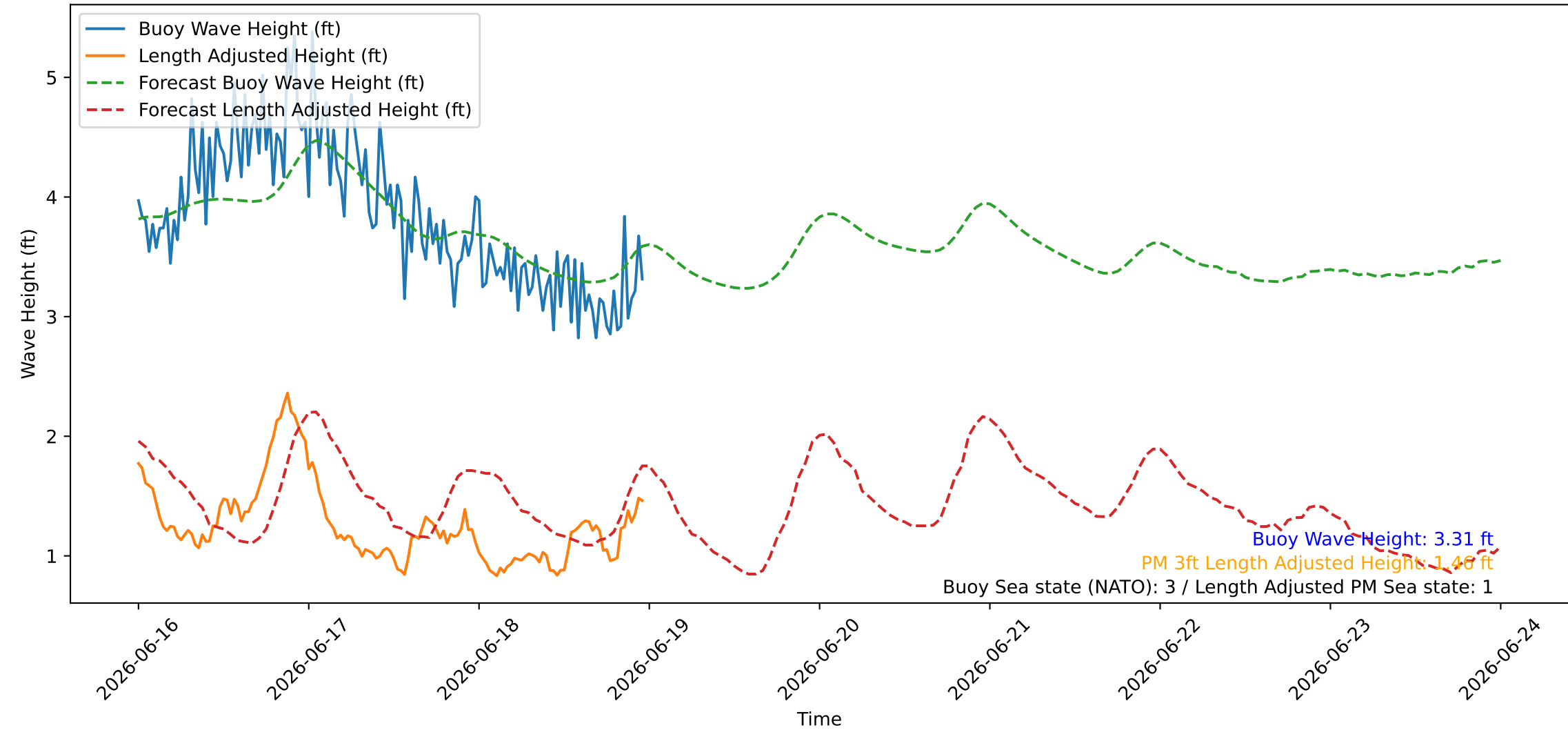
Wave Heights over Time for Red Beach at 2026-06-18 23:50:47
