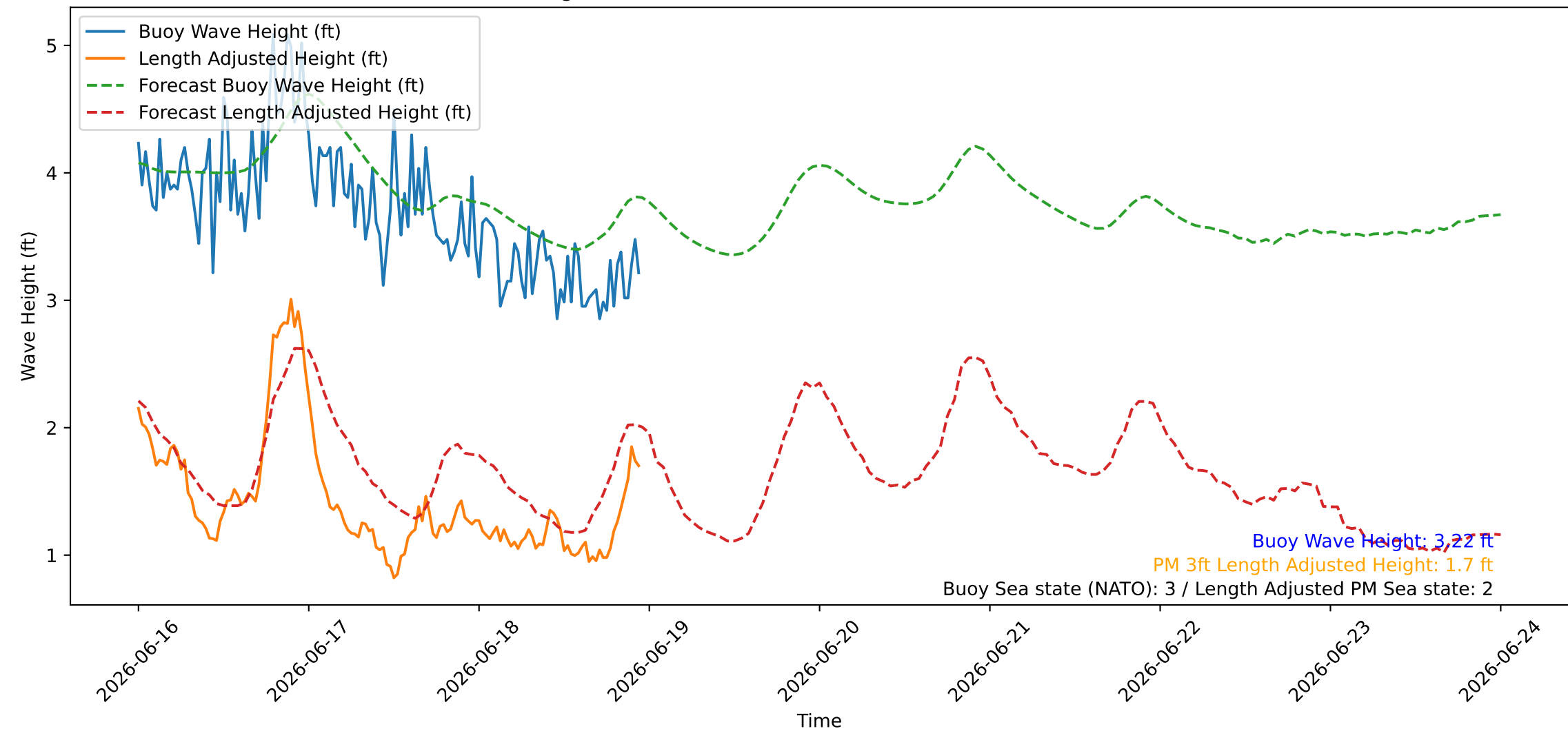
Wave Heights over Time for Green Beach at 2026-06-18 23:51:09
