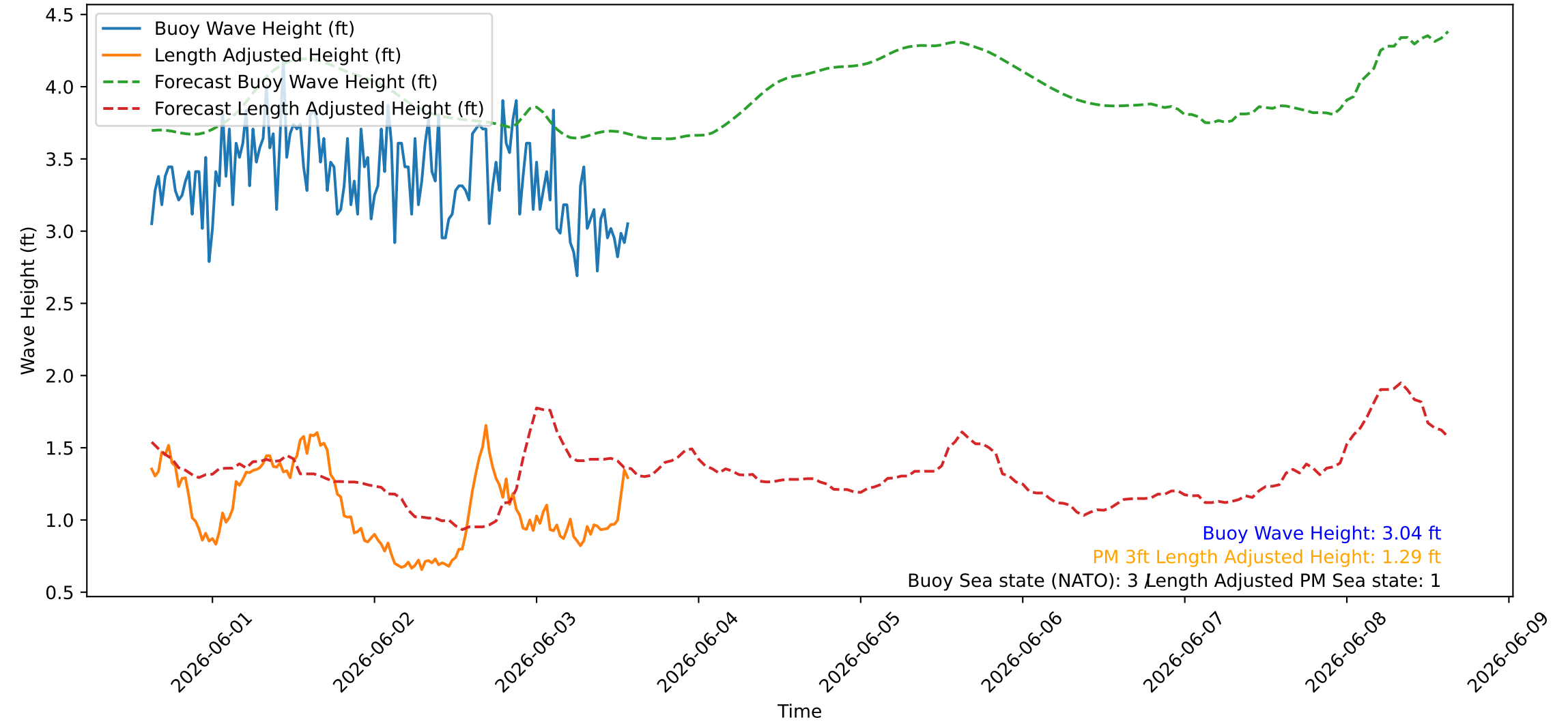
Wave Heights over Time for Red Beach at 2026-06-03 14:30:46
