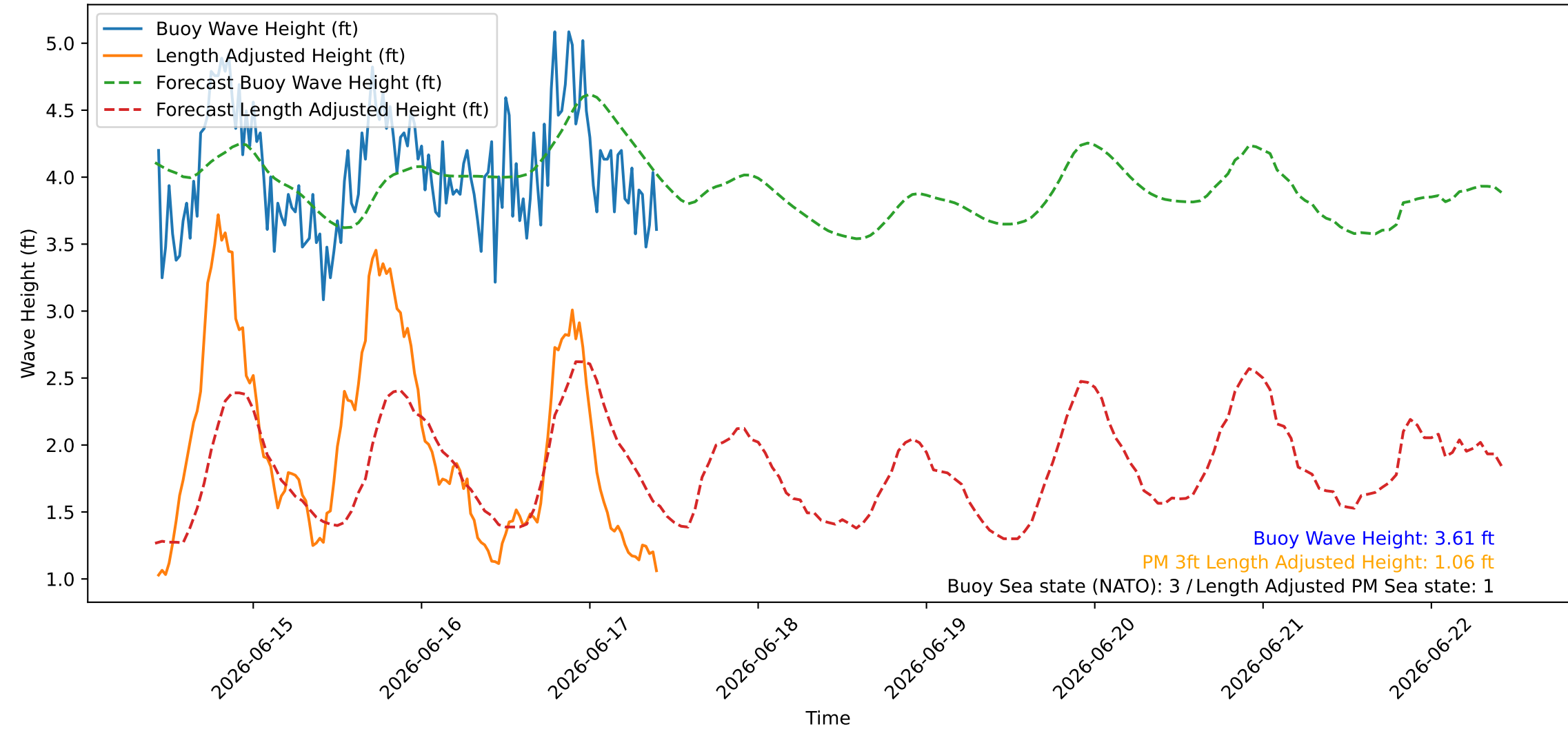
Wave Heights over Time for Green Beach at 2026-06-17 10:21:09
