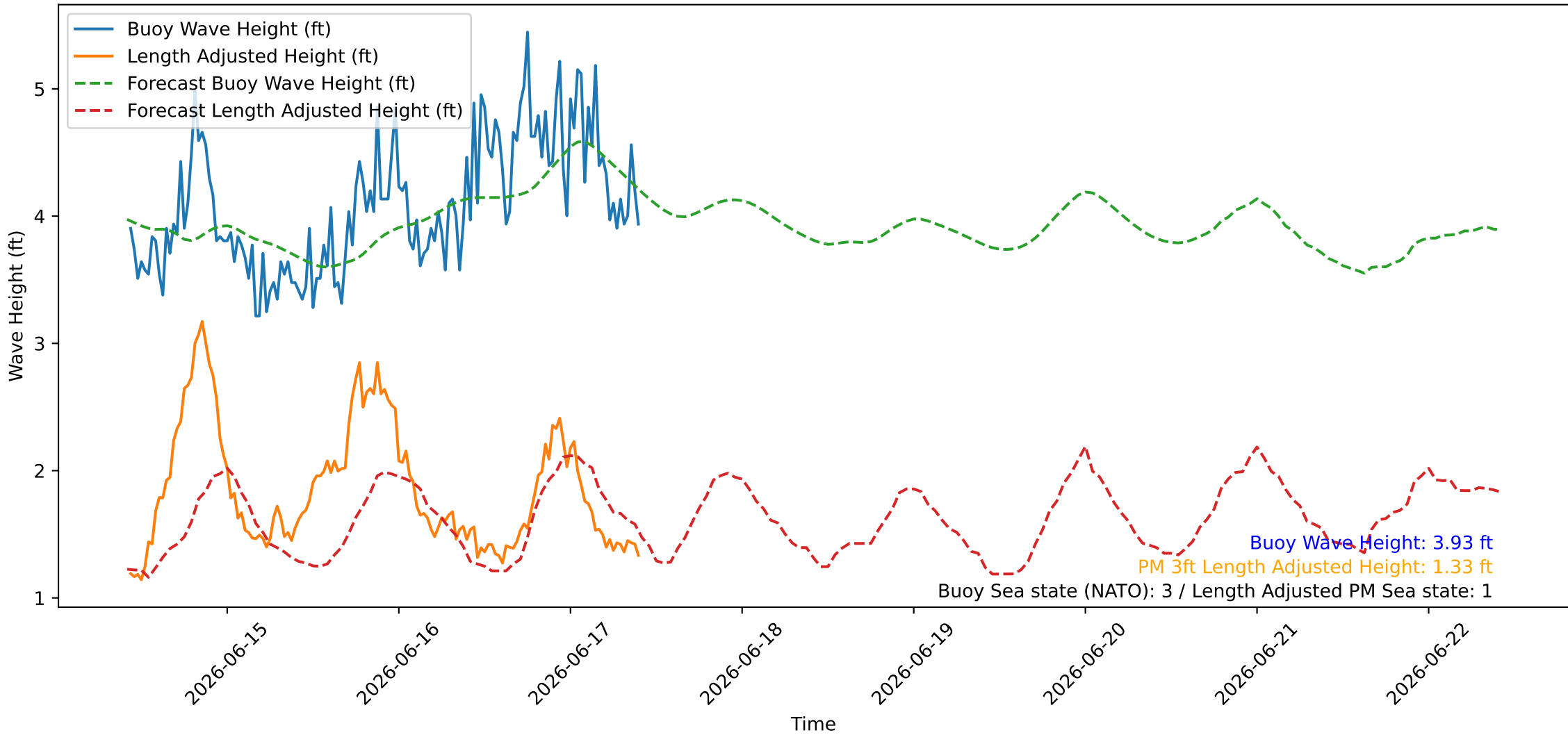
Wave Heights over Time for Oceanside Harbor at 2026-06-17 10:20:26
