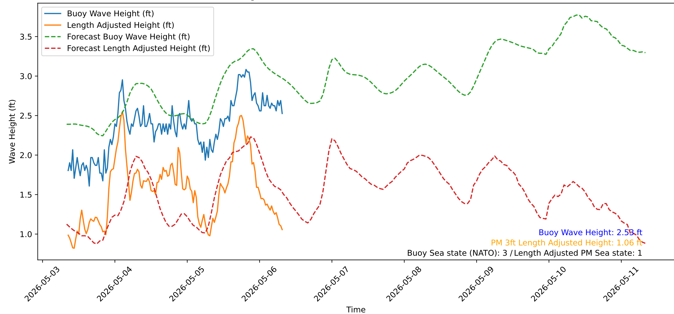
Wave Heights over Time for Red Beach at 2026-05-06 08:20:51
