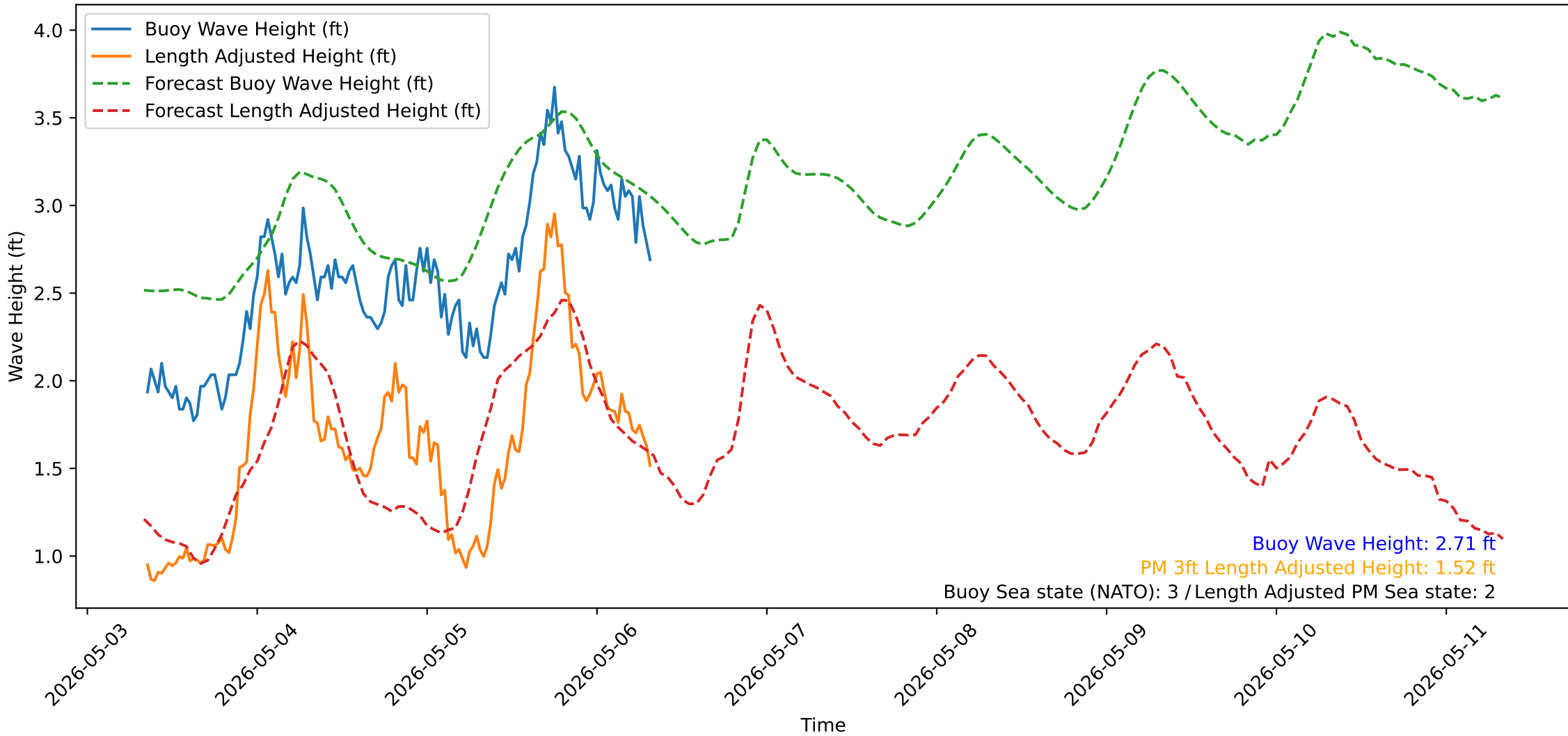
Wave Heights over Time for Green Beach at 2026-05-06 08:21:13
