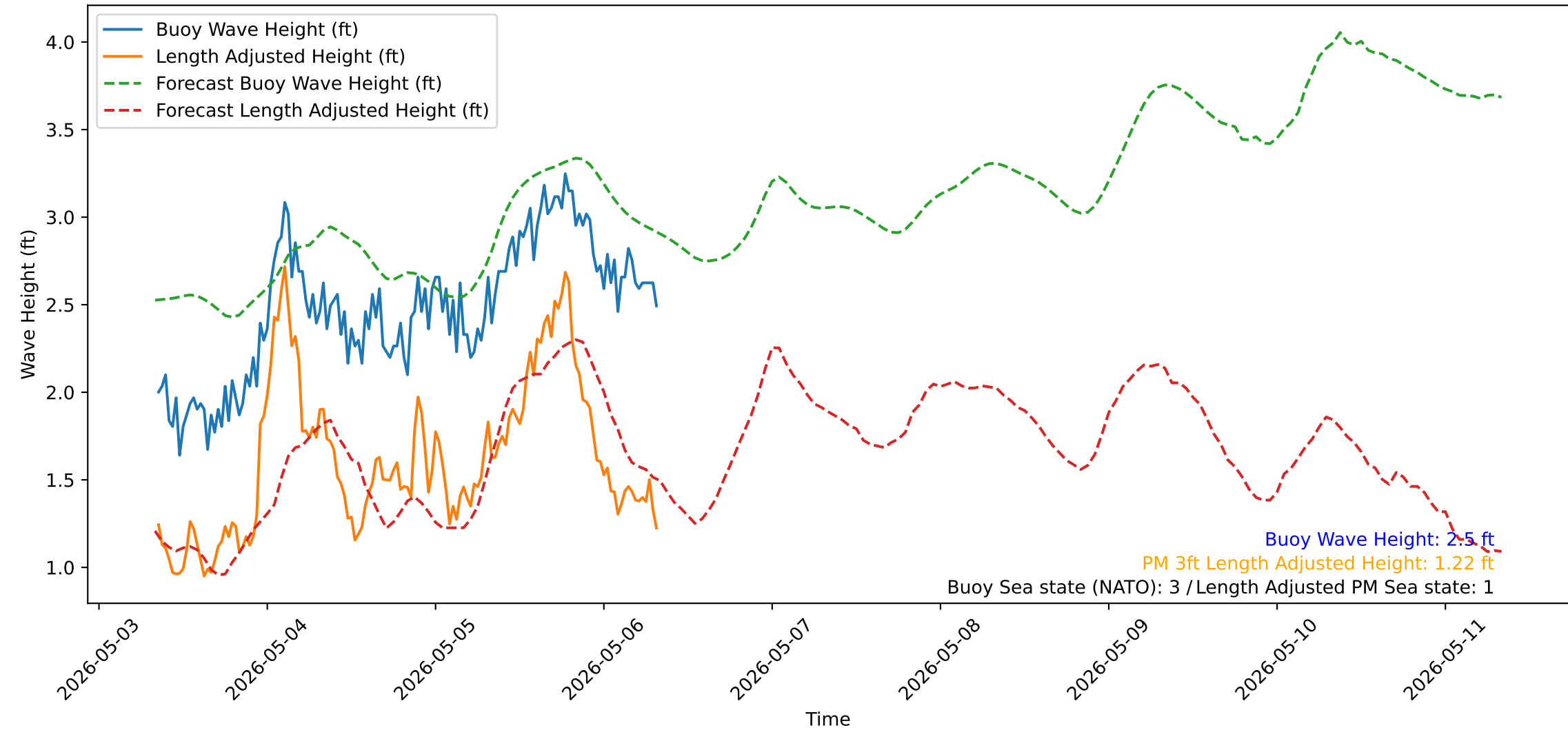
Wave Heights over Time for Oceanside Harbor at 2026-05-06 08:20:31
