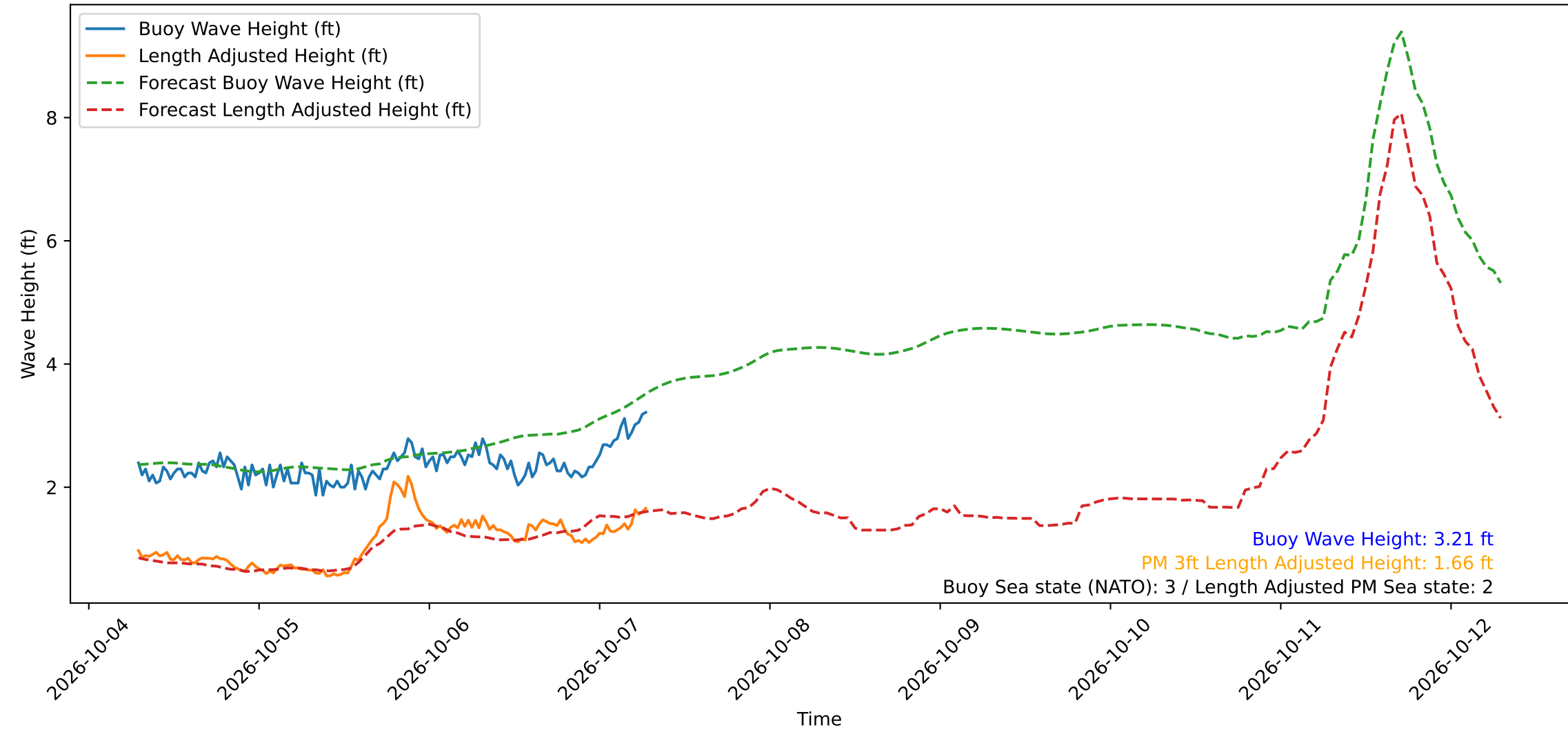
Wave Heights over Time for Oceanside Harbor at 2026-10-07 07:10:30
