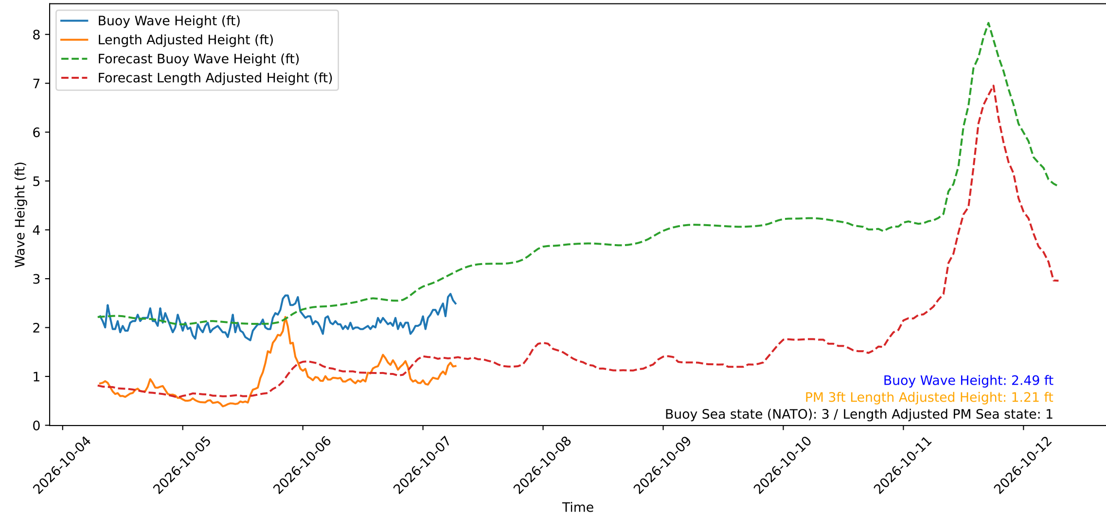
Wave Heights over Time for Red Beach at 2026-10-07 07:10:50
