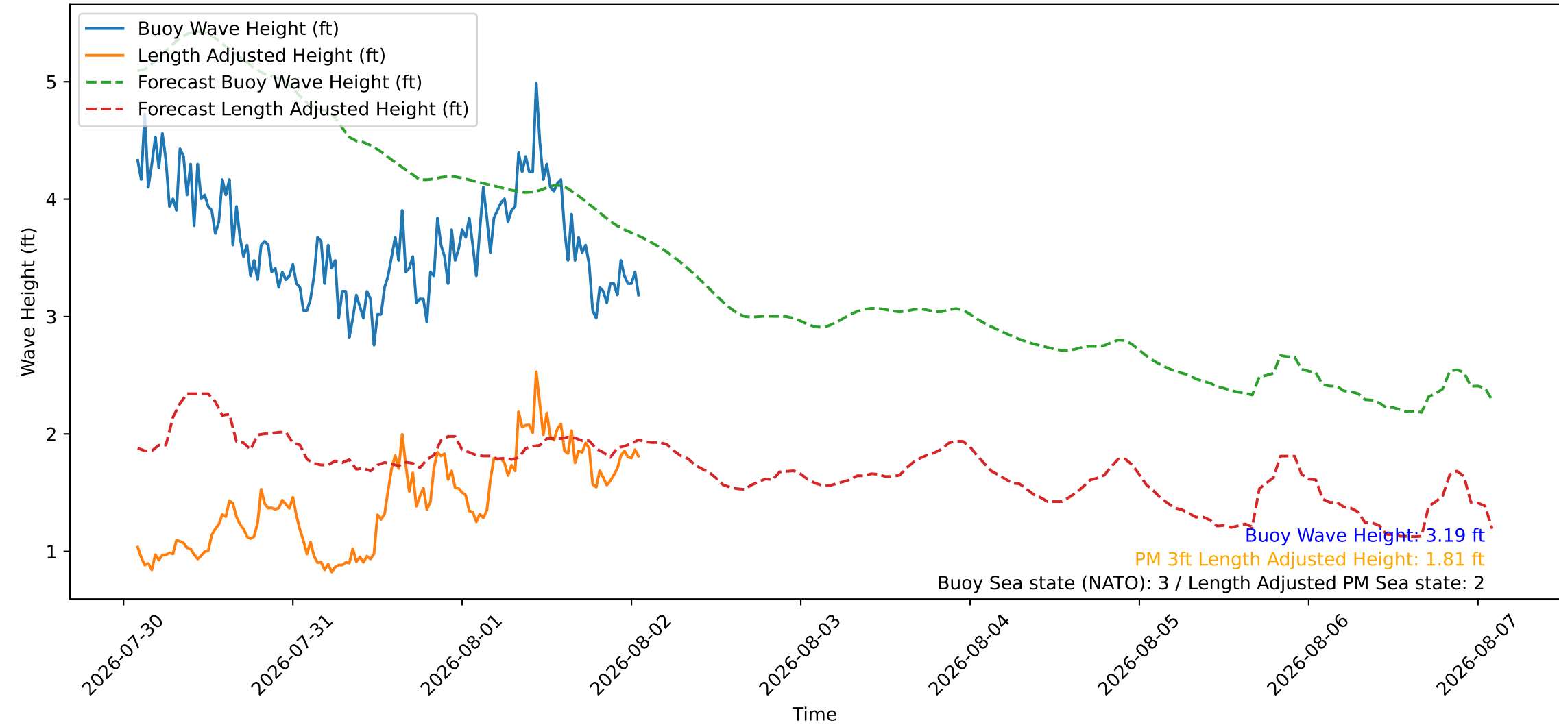
Wave Heights over Time for Green Beach at 2026-08-02 02:01:09
