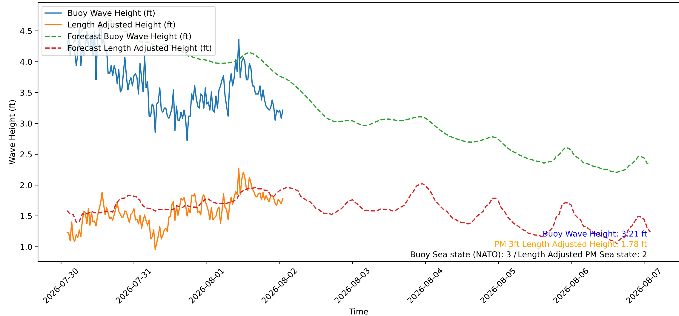
Wave Heights over Time for Oceanside Harbor at 2026-08-02 02:00:27
