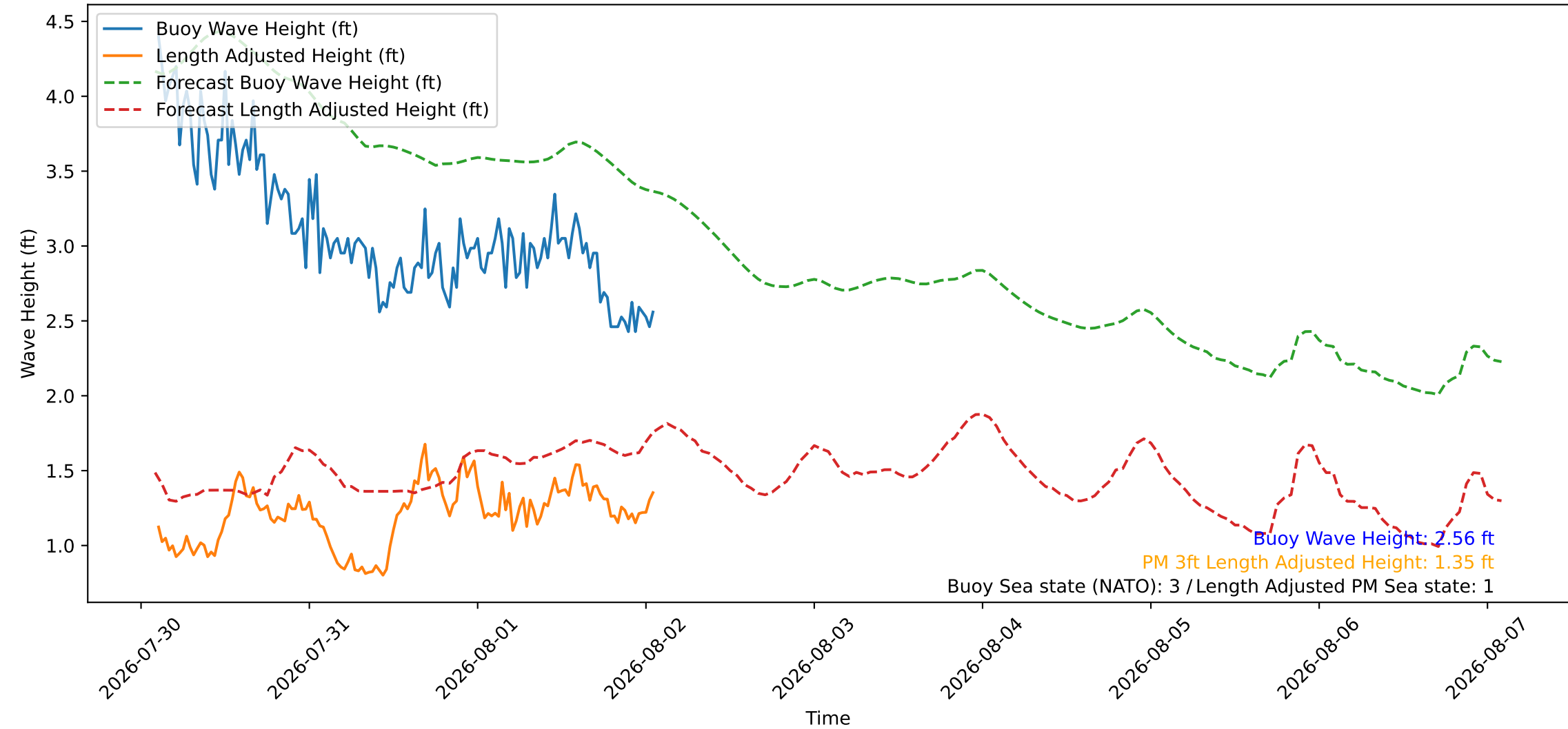
Wave Heights over Time for Red Beach at 2026-08-02 02:00:46
