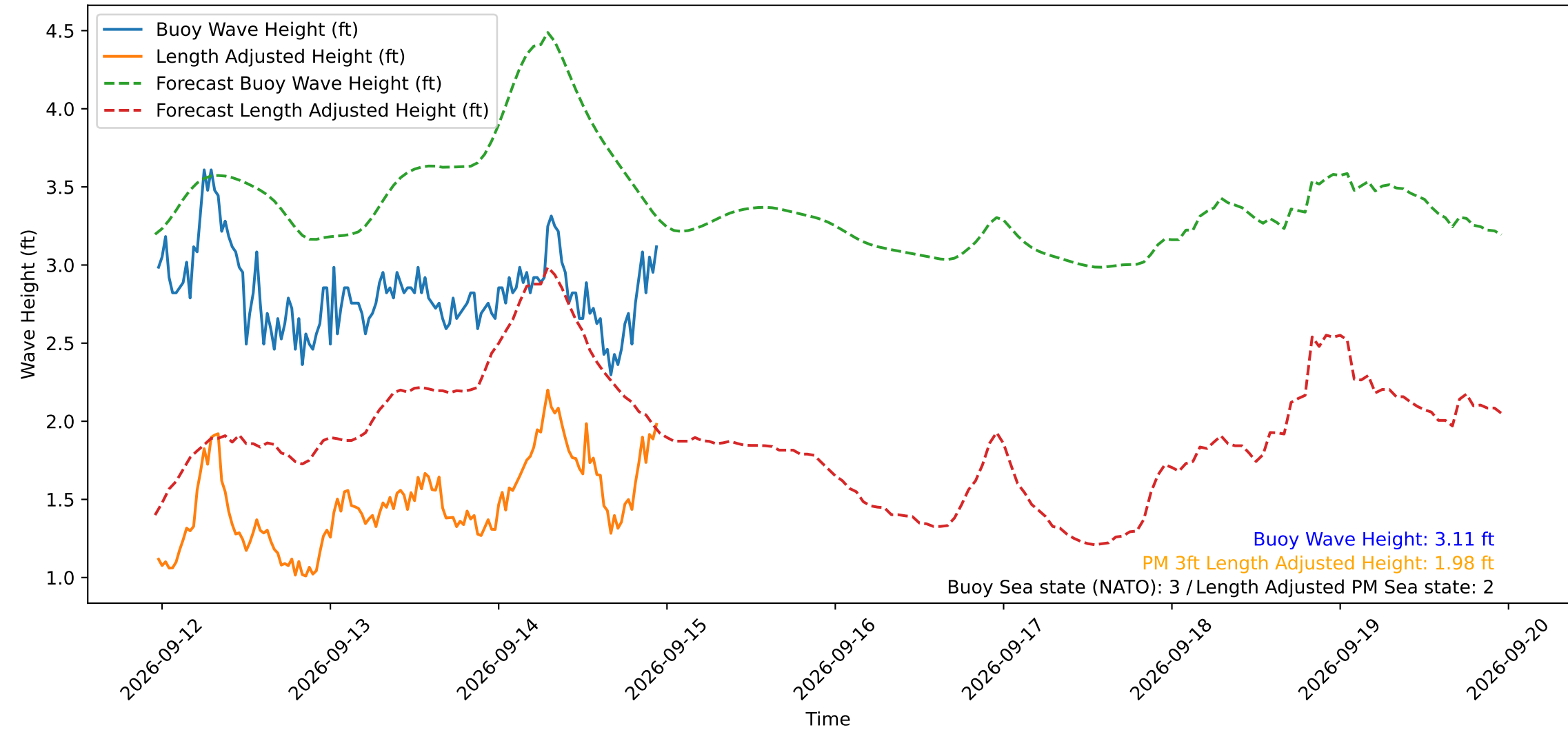
Wave Heights over Time for Green Beach at 2026-09-14 23:11:11
