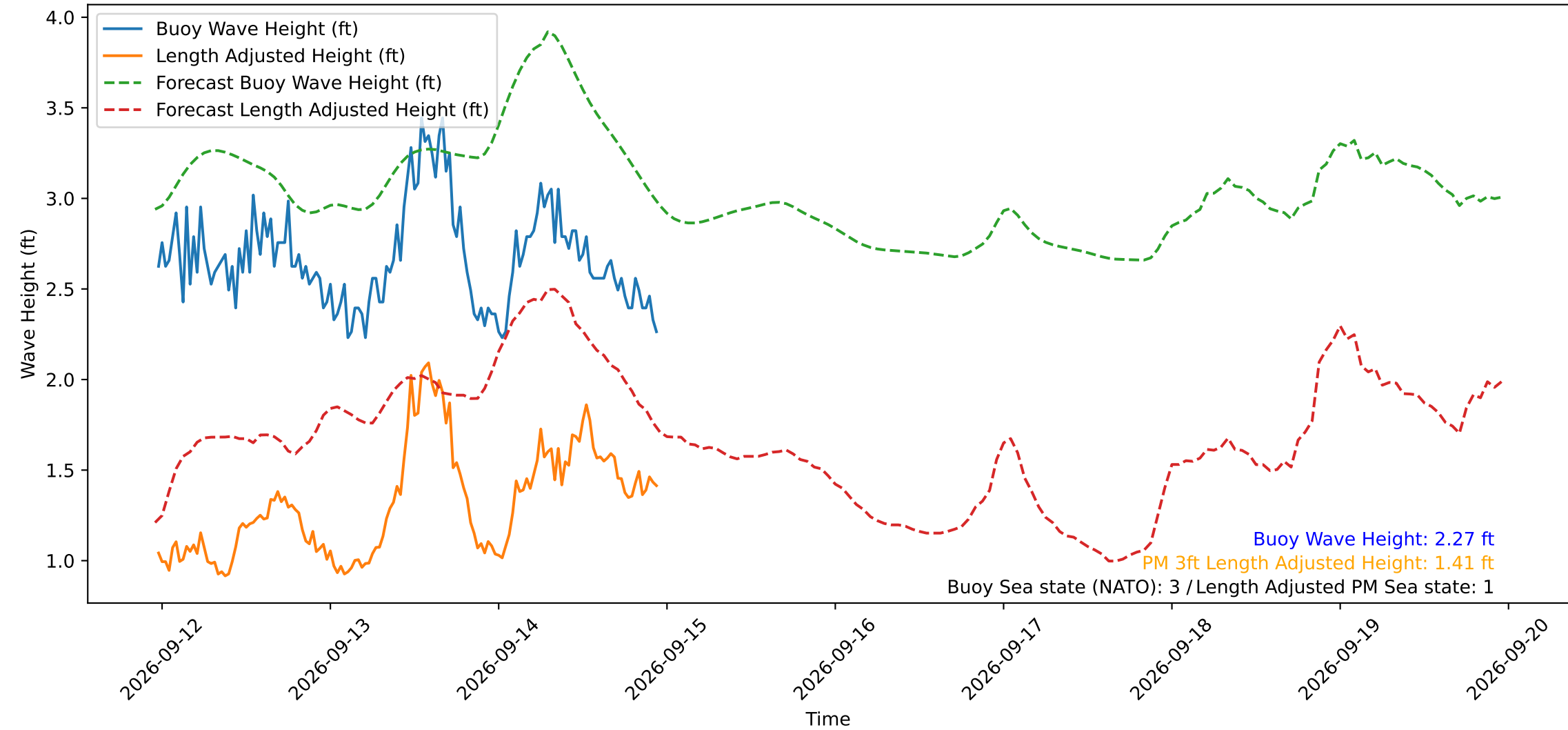
Wave Heights over Time for Red Beach at 2026-09-14 23:10:49
