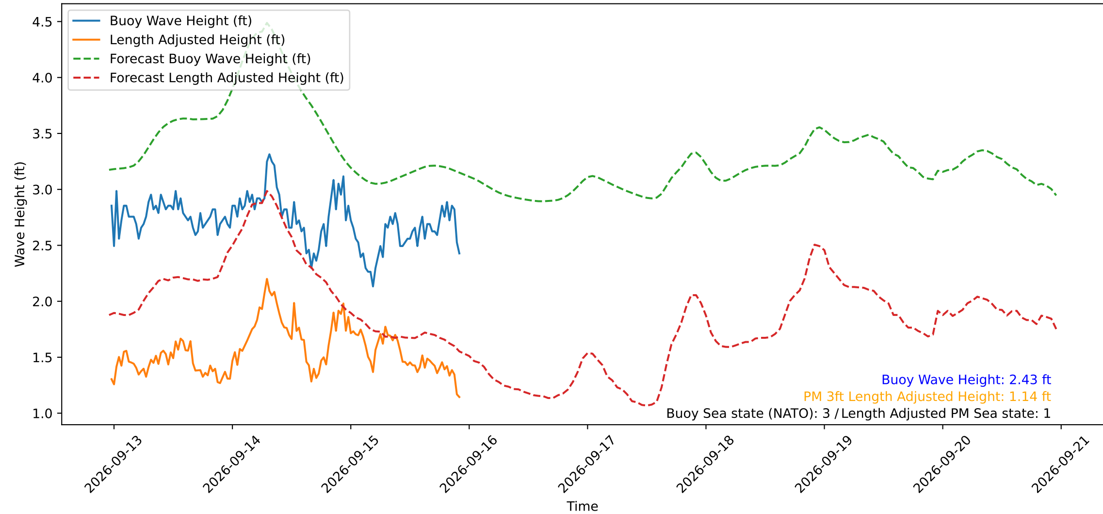
Wave Heights over Time for Green Beach at 2026-09-15 23:01:11
