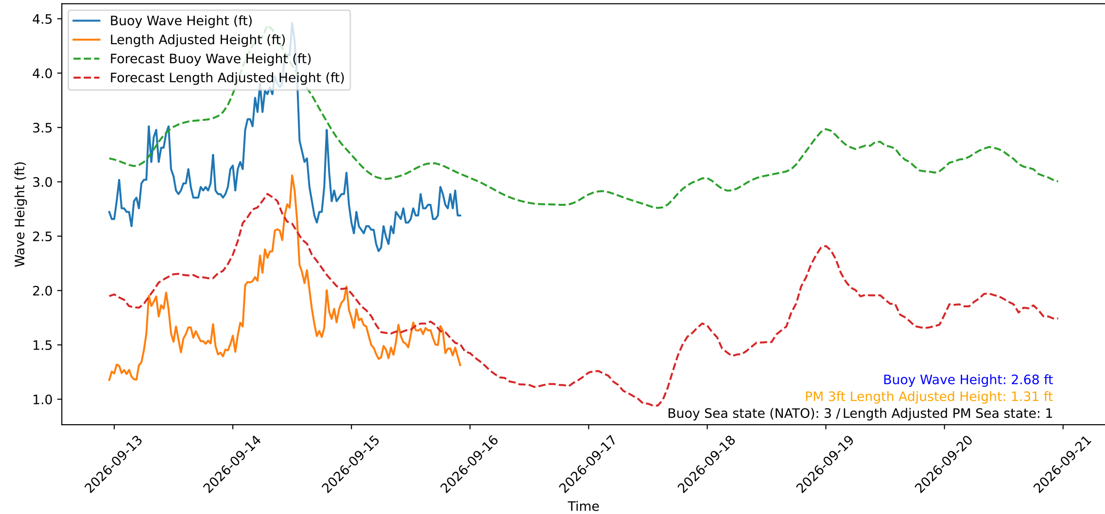
Wave Heights over Time for Oceanside Harbor at 2026-09-15 23:00:29
