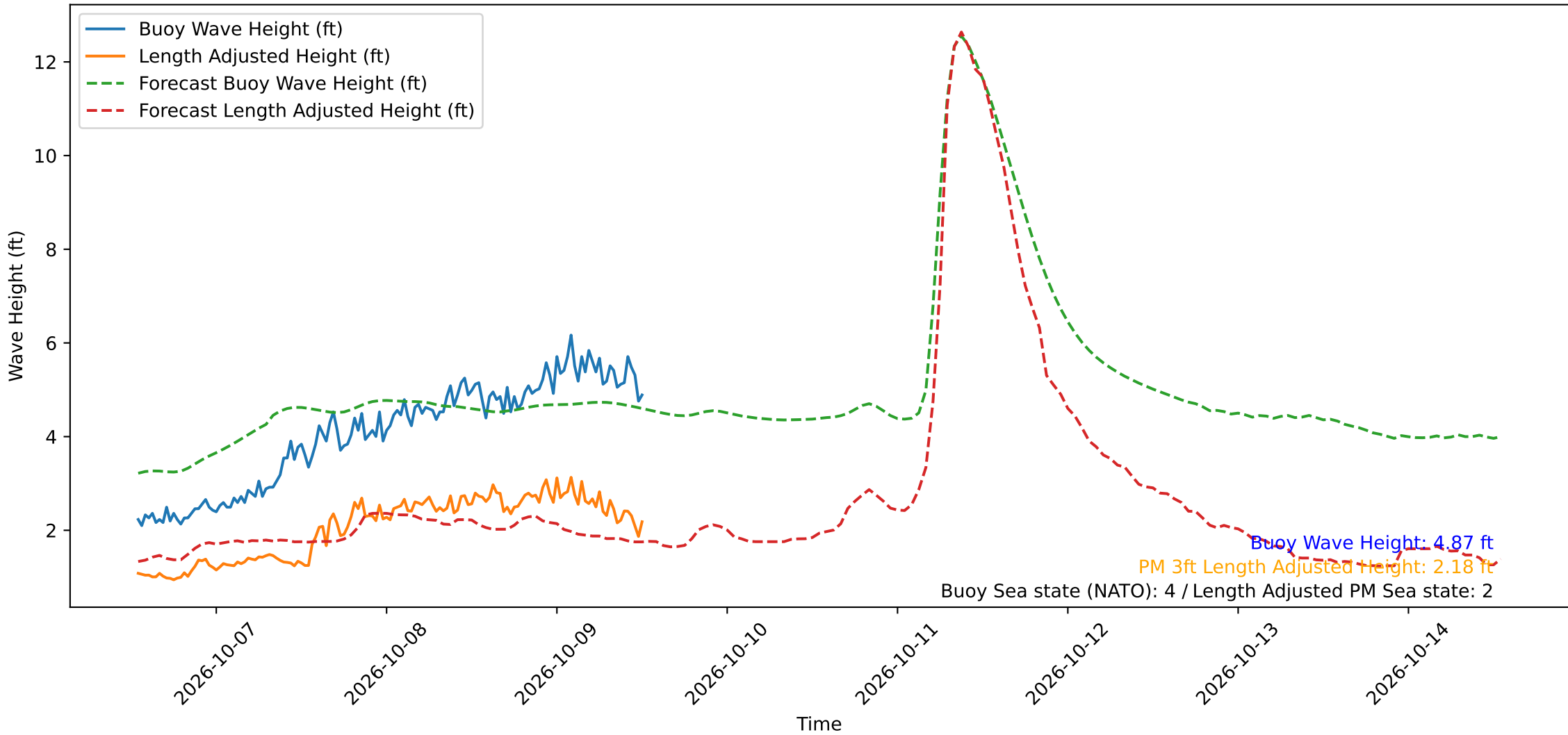
Wave Heights over Time for Green Beach at 2026-10-09 12:51:14
