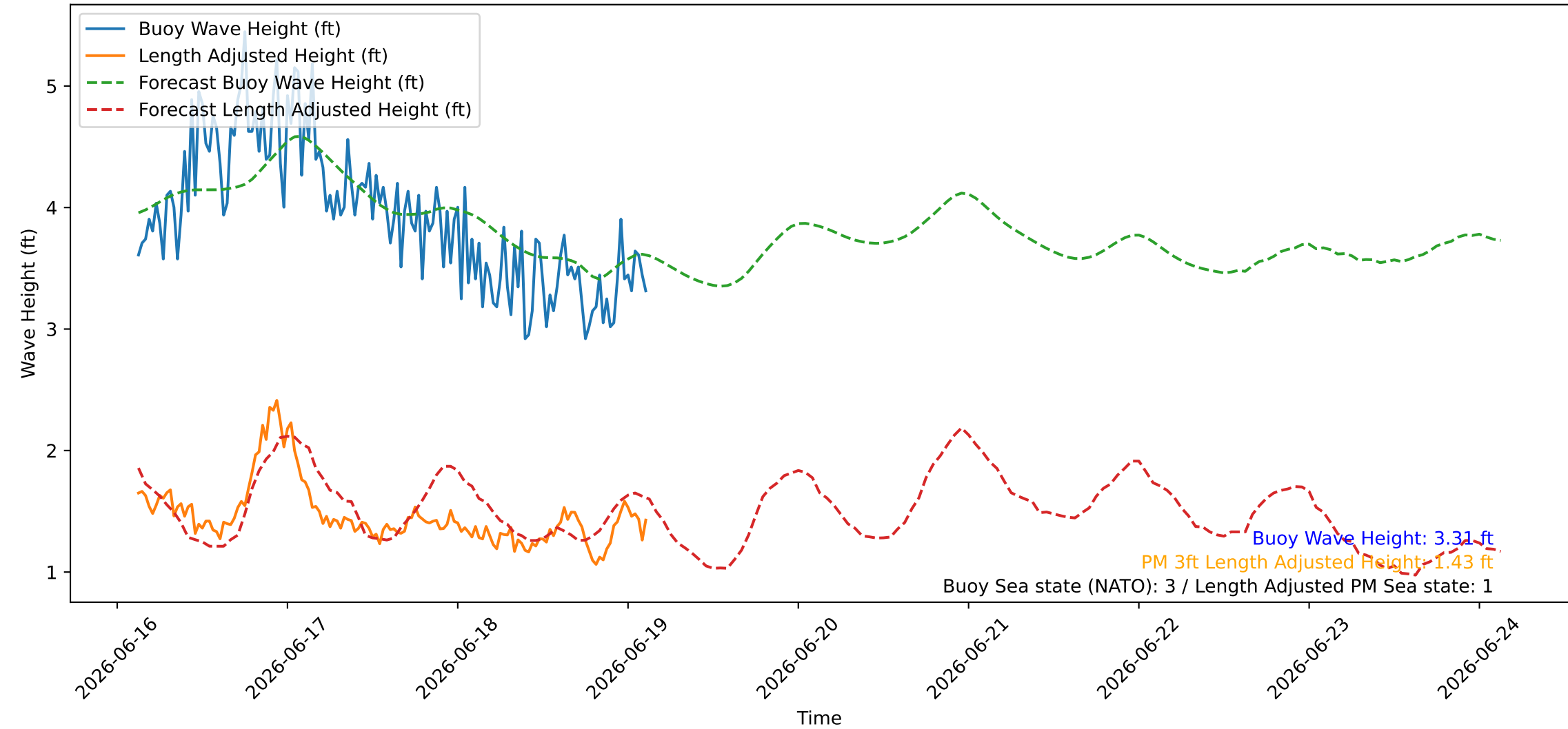
Wave Heights over Time for Oceanside Harbor at 2026-06-19 03:10:26
