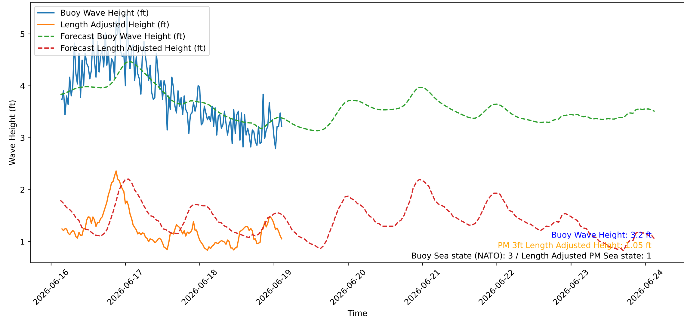
Wave Heights over Time for Red Beach at 2026-06-19 03:10:45
