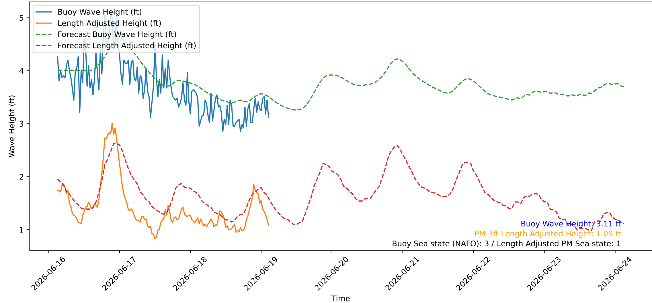
Wave Heights over Time for Green Beach at 2026-06-19 03:11:08
