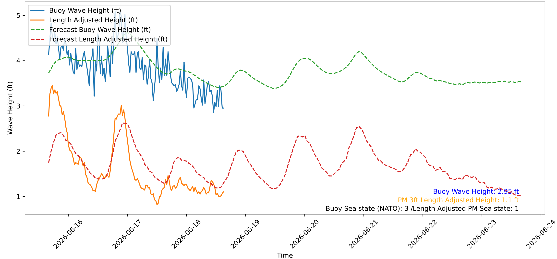
Wave Heights over Time for Green Beach at 2026-06-18 15:51:10
