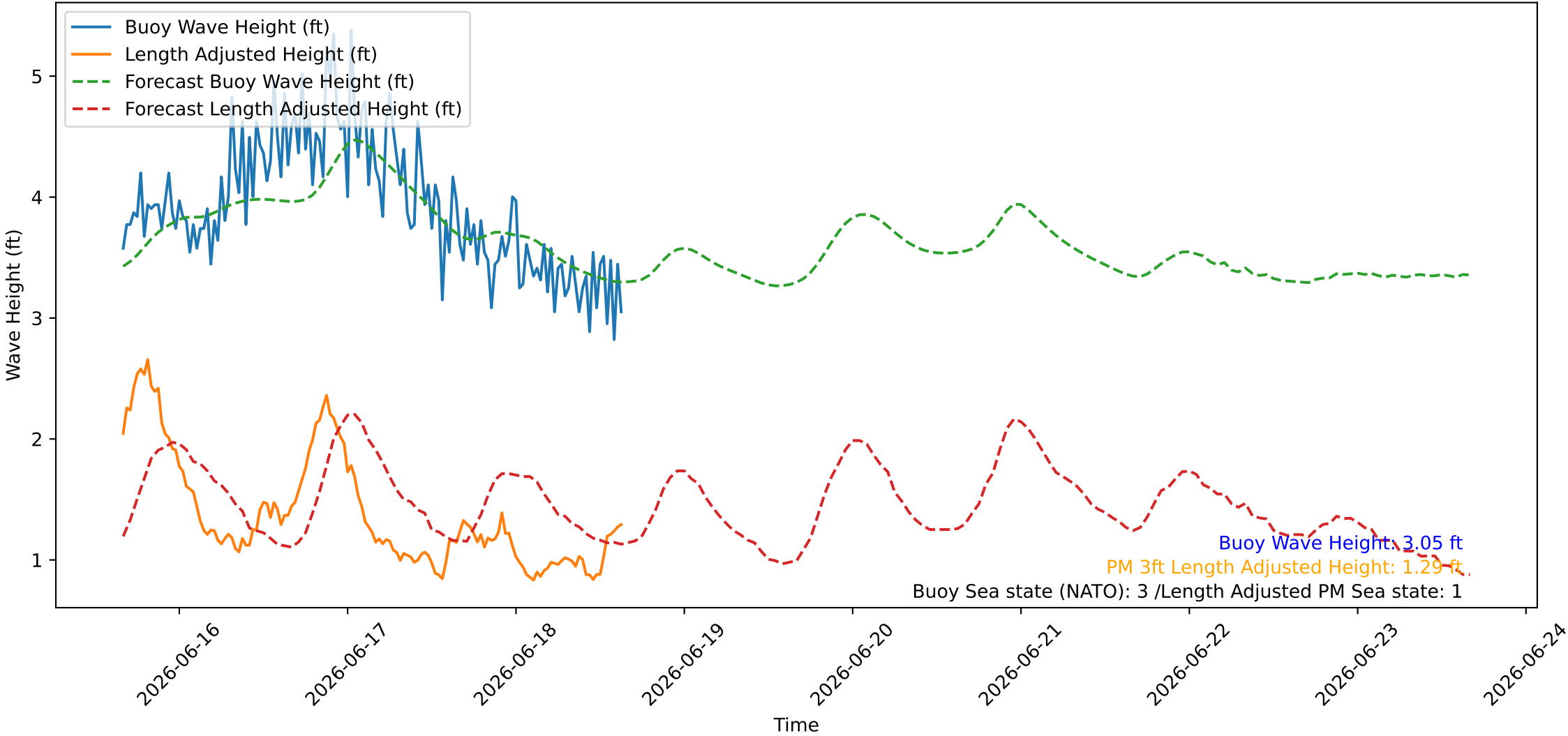
Wave Heights over Time for Red Beach at 2026-06-18 15:50:47
