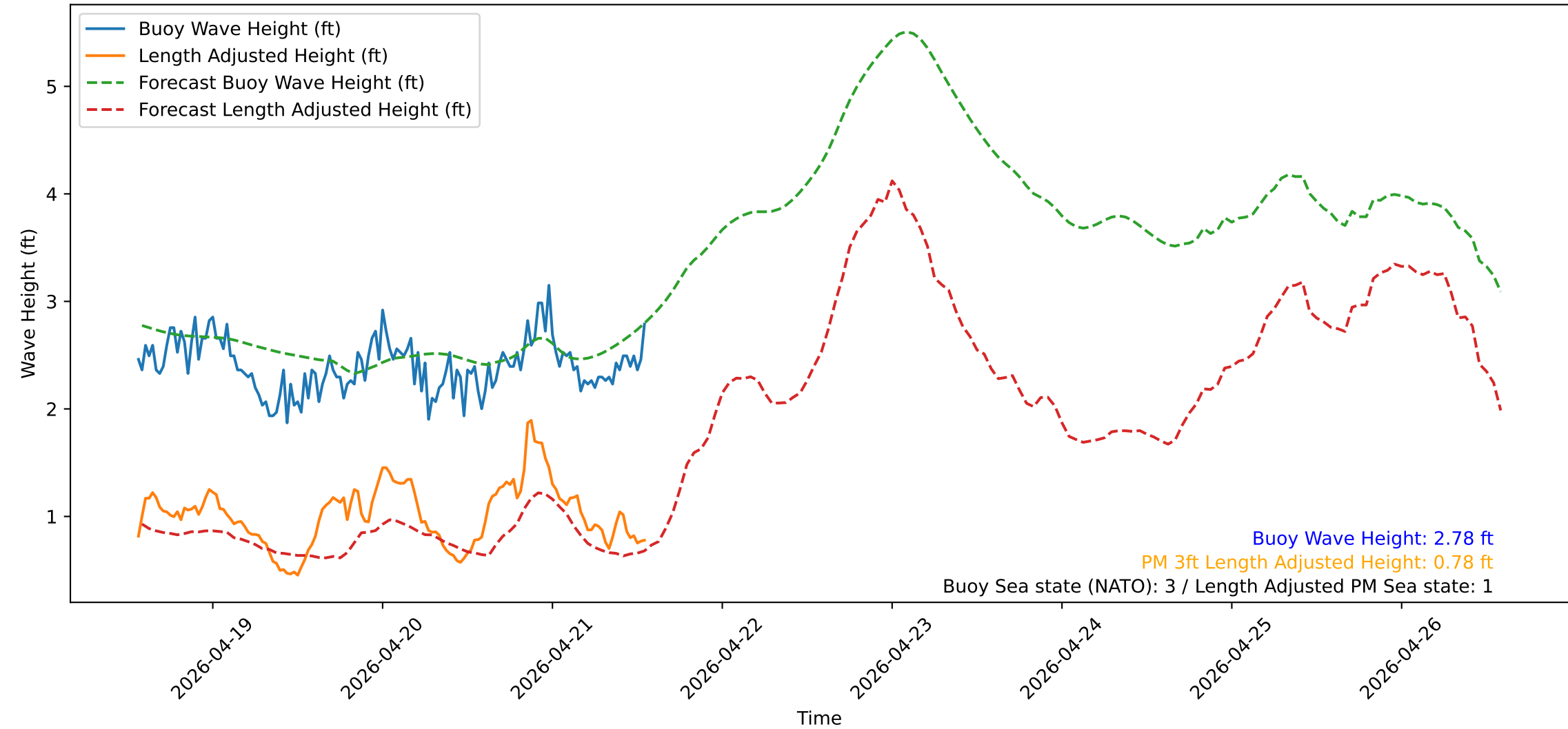
Wave Heights over Time for Green Beach at 2026-04-21 13:41:13
