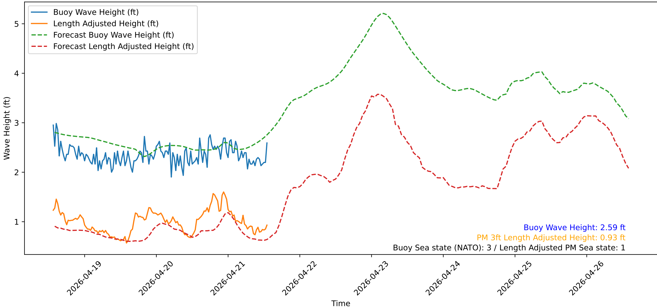
Wave Heights over Time for Oceanside Harbor at 2026-04-21 13:40:31
