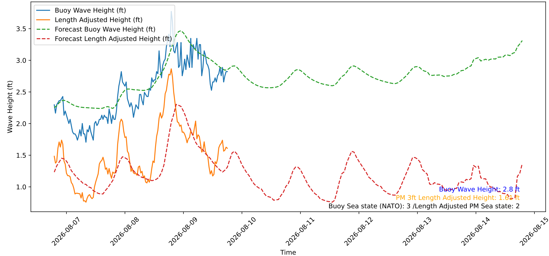
Wave Heights over Time for Green Beach at 2026-08-09 18:51:10
