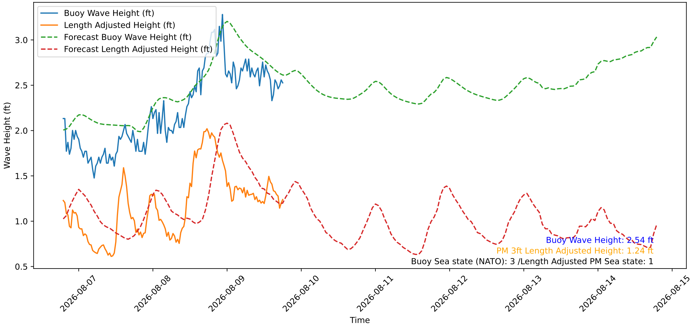
Wave Heights over Time for Red Beach at 2026-08-09 18:50:48
