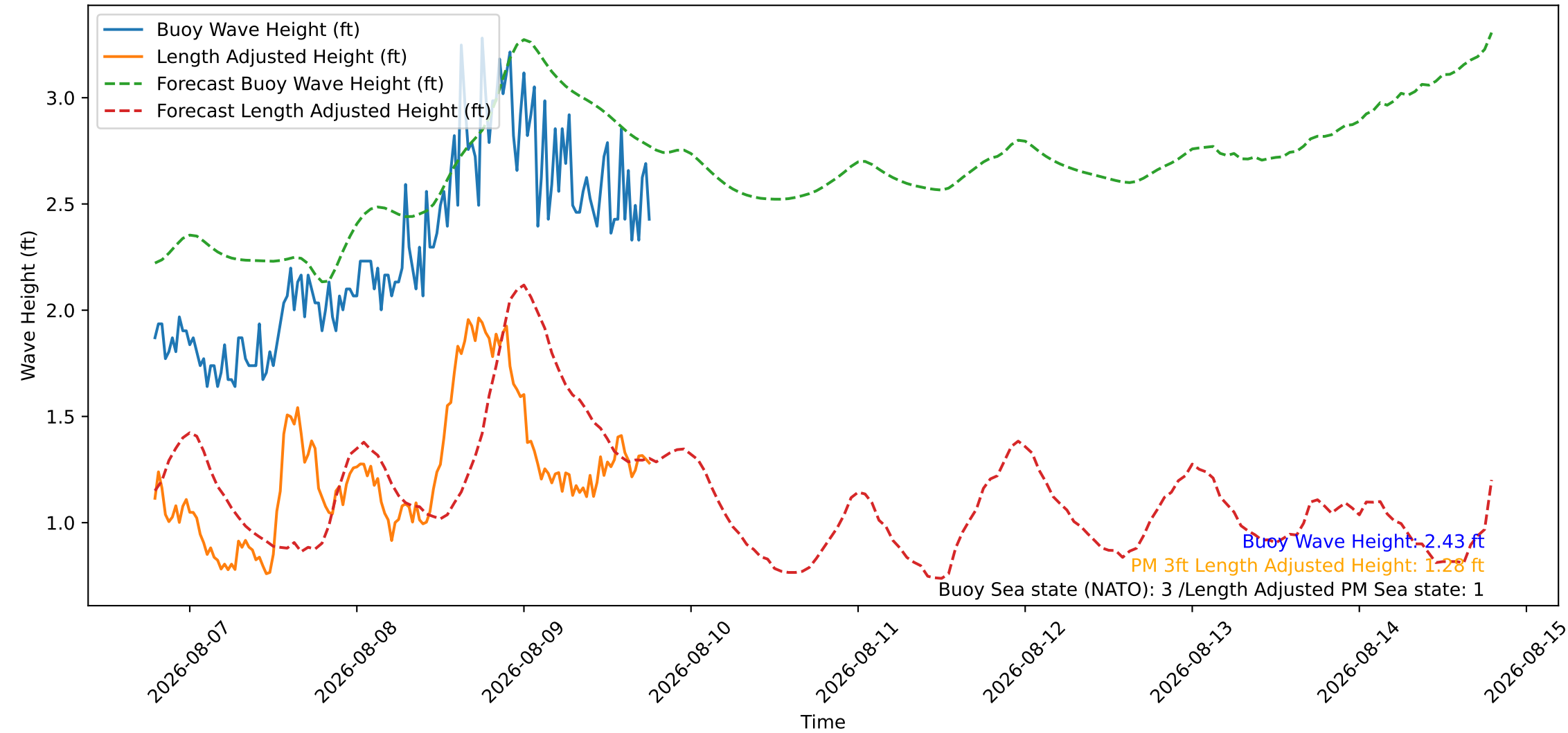
Wave Heights over Time for Oceanside Harbor at 2026-08-09 18:50:27
