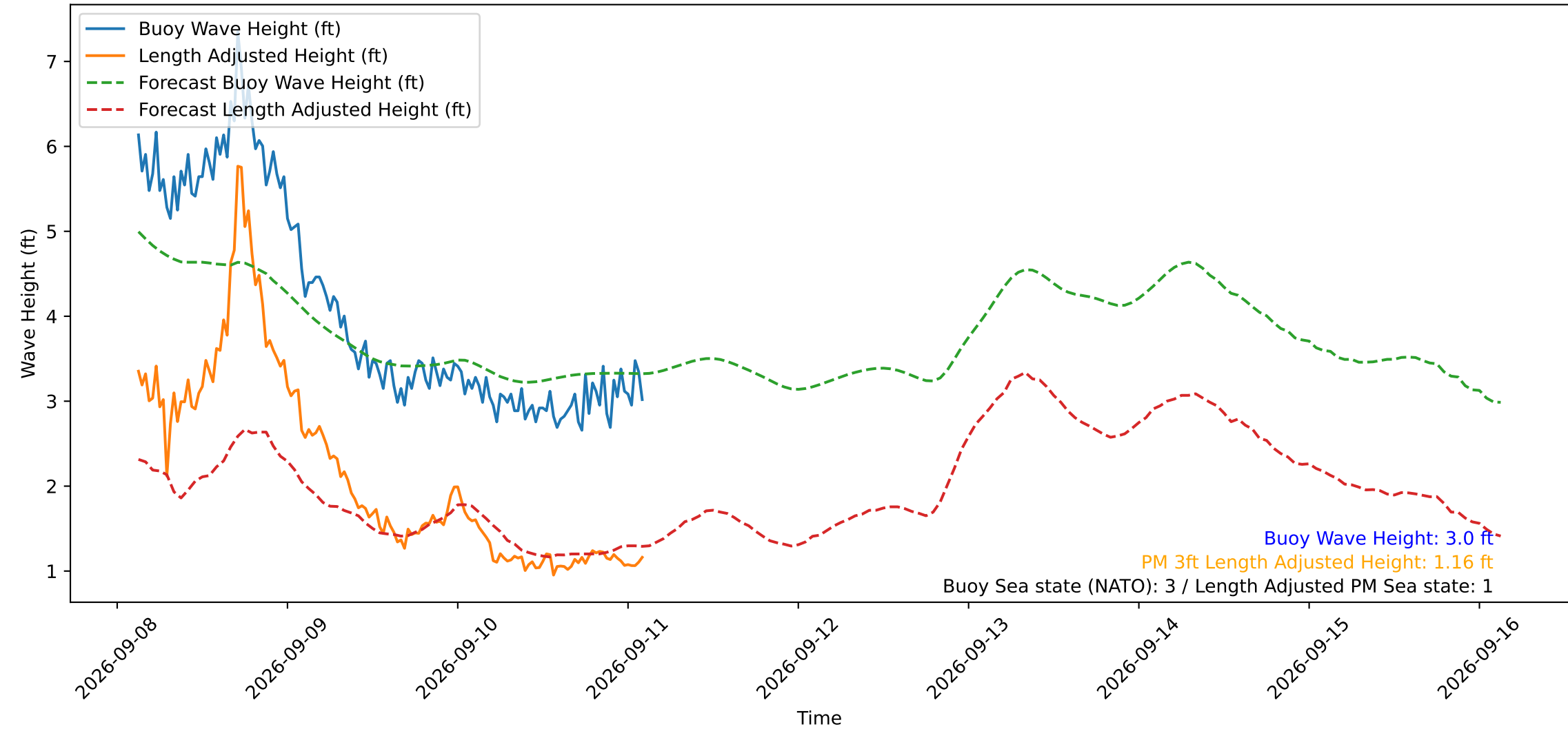
Wave Heights over Time for Oceanside Harbor at 2026-09-11 03:00:29
