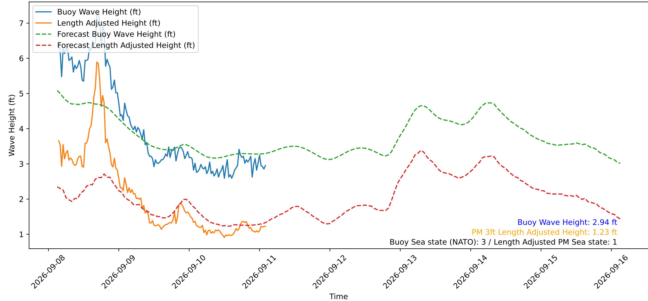
Wave Heights over Time for Green Beach at 2026-09-11 03:01:11
