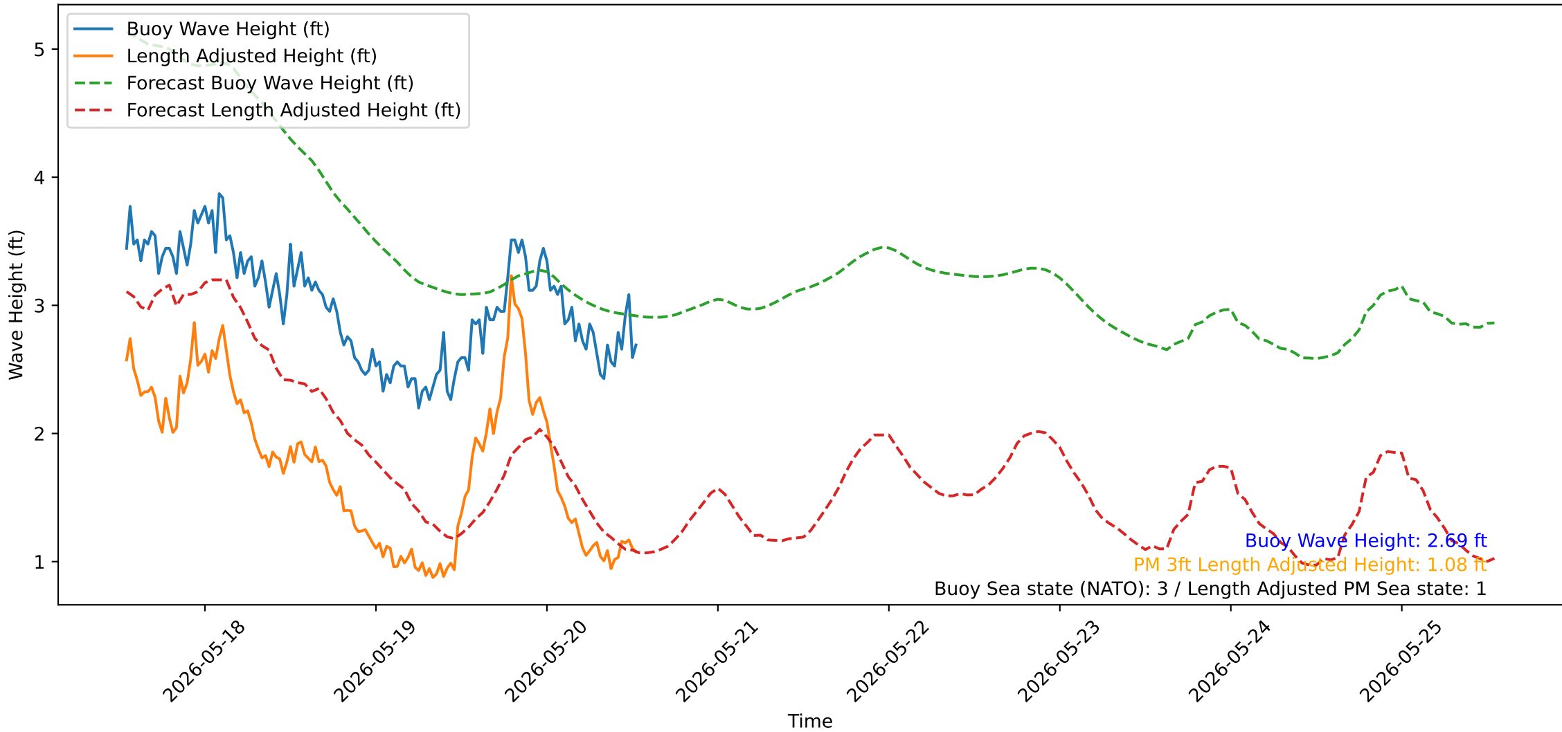
Wave Heights over Time for Oceanside Harbor at 2026-05-20 13:10:32
