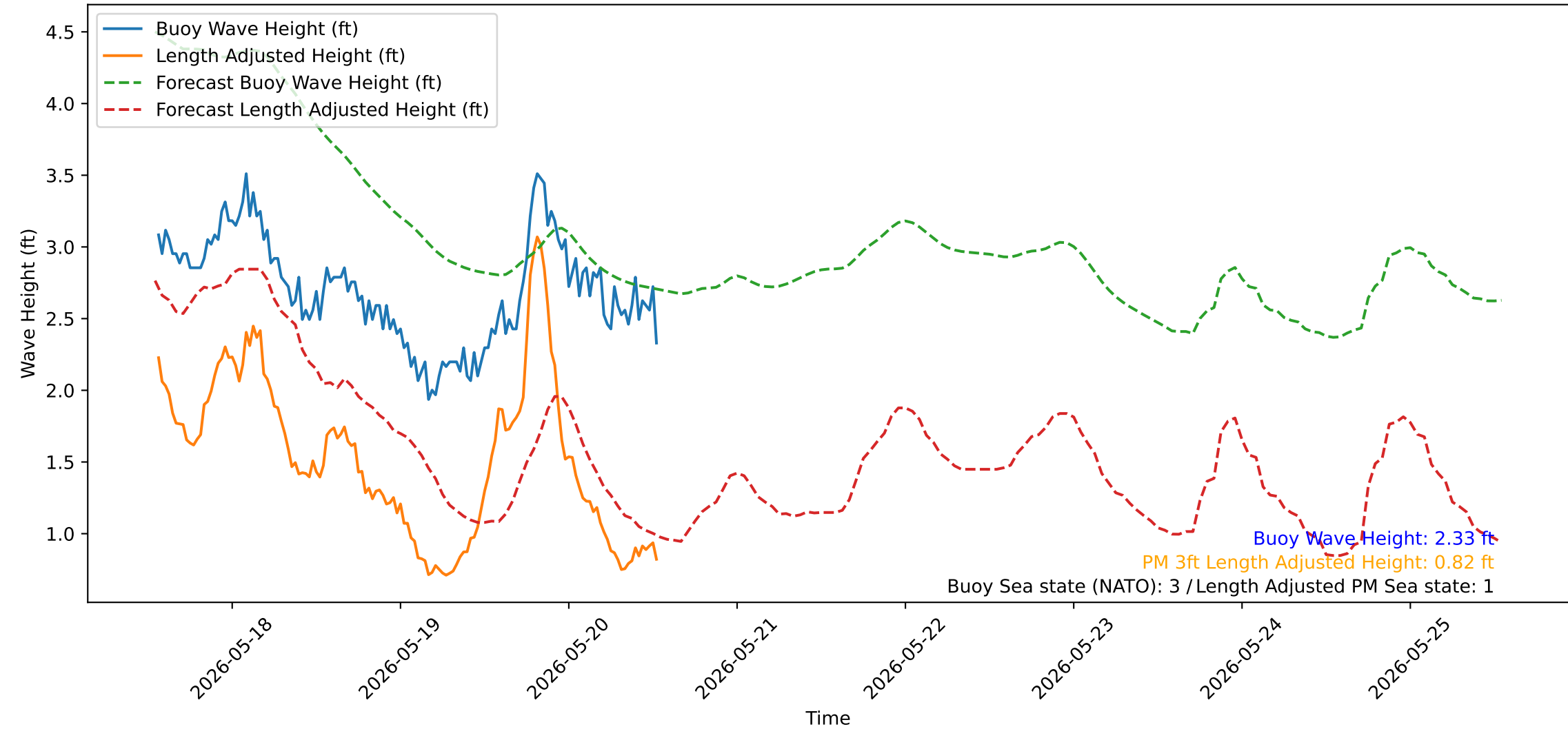
Wave Heights over Time for Red Beach at 2026-05-20 13:10:51
