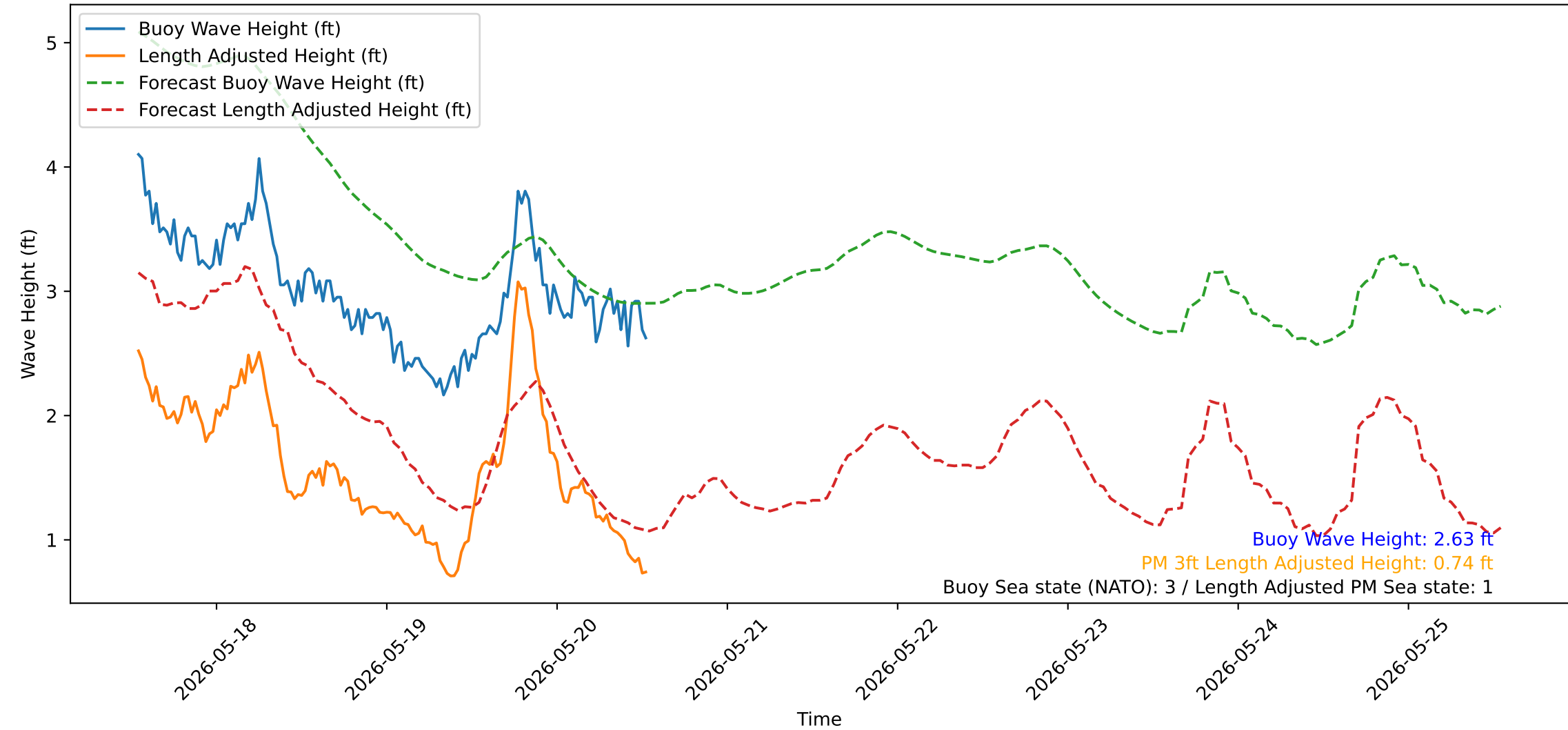
Wave Heights over Time for Green Beach at 2026-05-20 13:11:14
