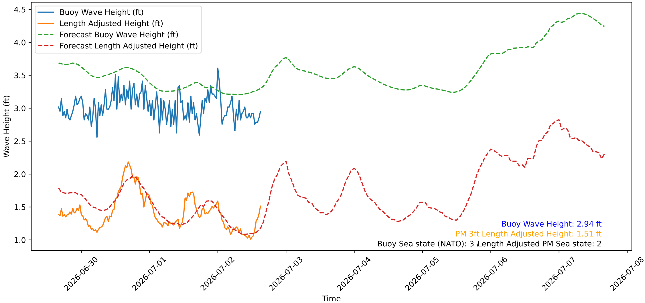
Wave Heights over Time for Oceanside Harbor at 2026-07-02 16:00:26
