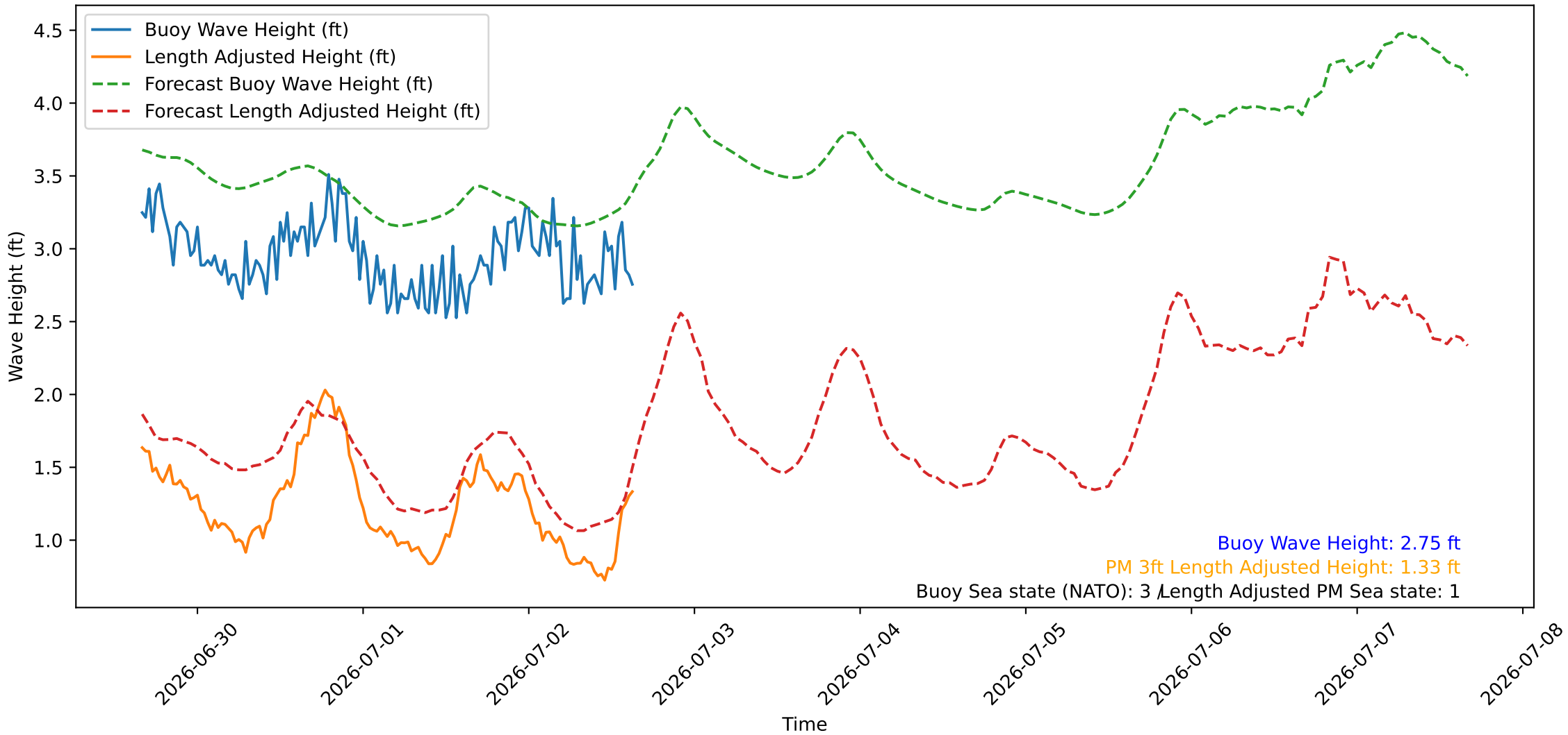
Wave Heights over Time for Green Beach at 2026-07-02 16:01:07
