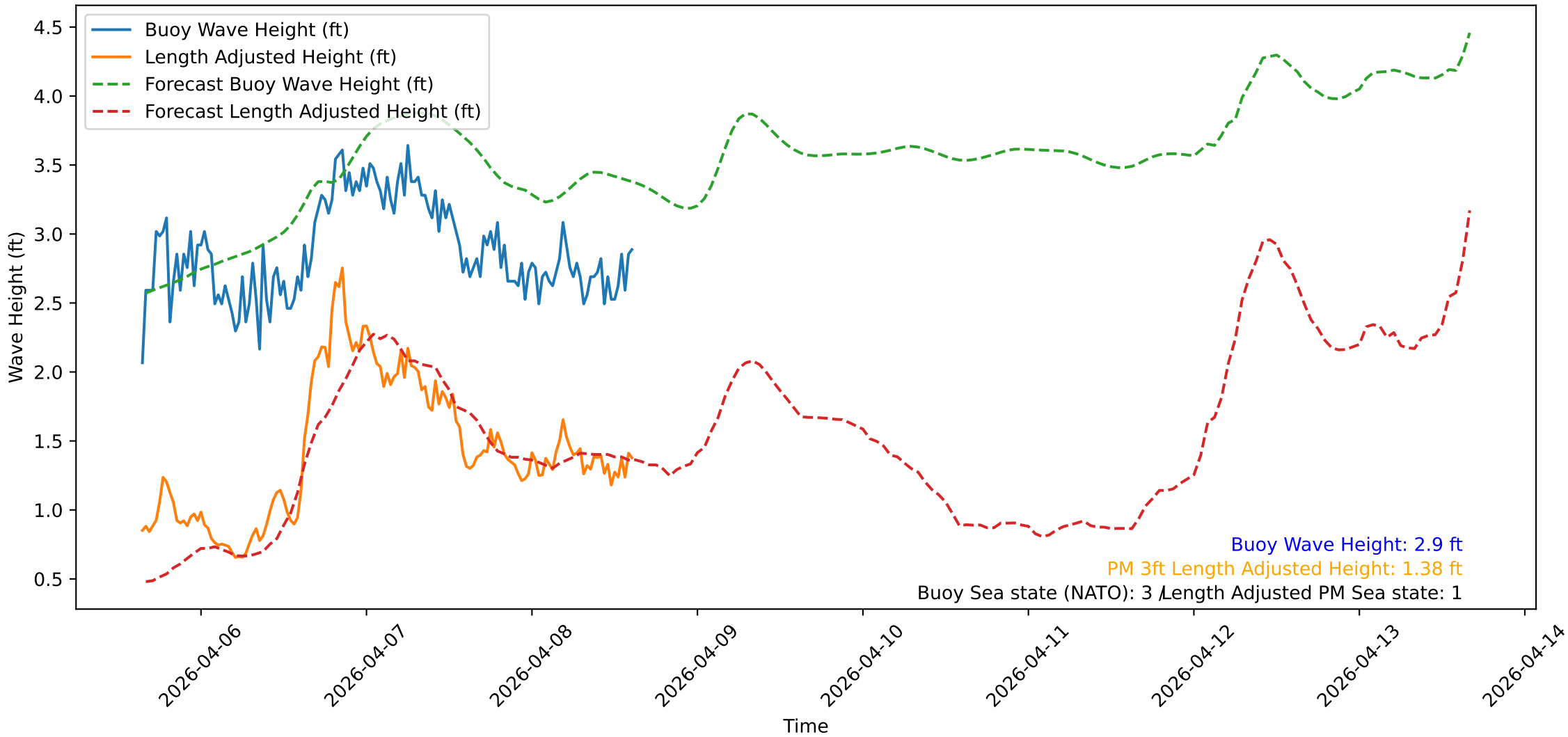
Wave Heights over Time for Oceanside Harbor at 2026-04-08 15:30:32
