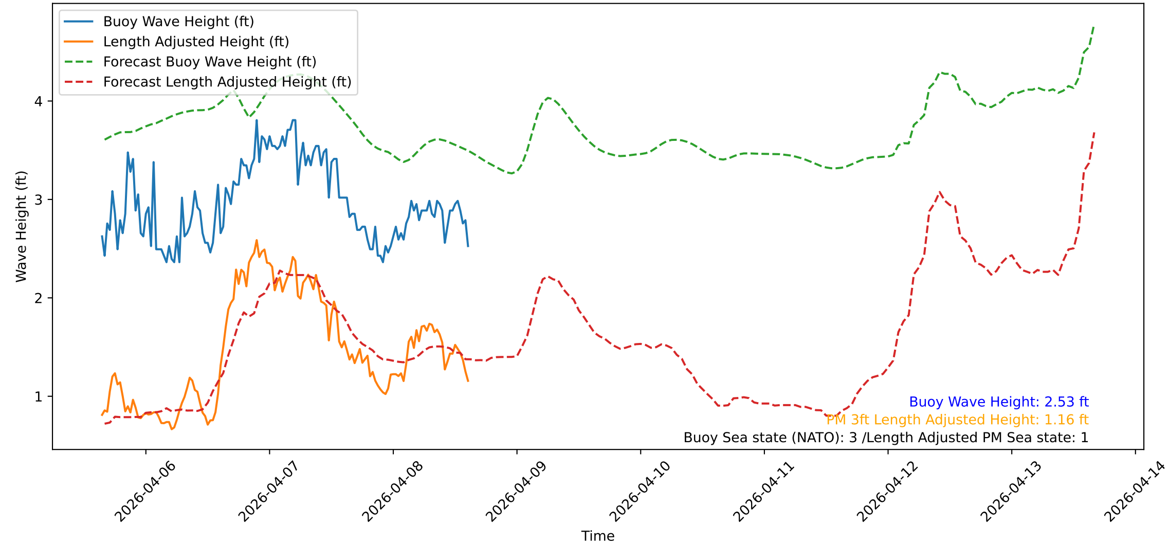
Wave Heights over Time for Green Beach at 2026-04-08 15:31:10
