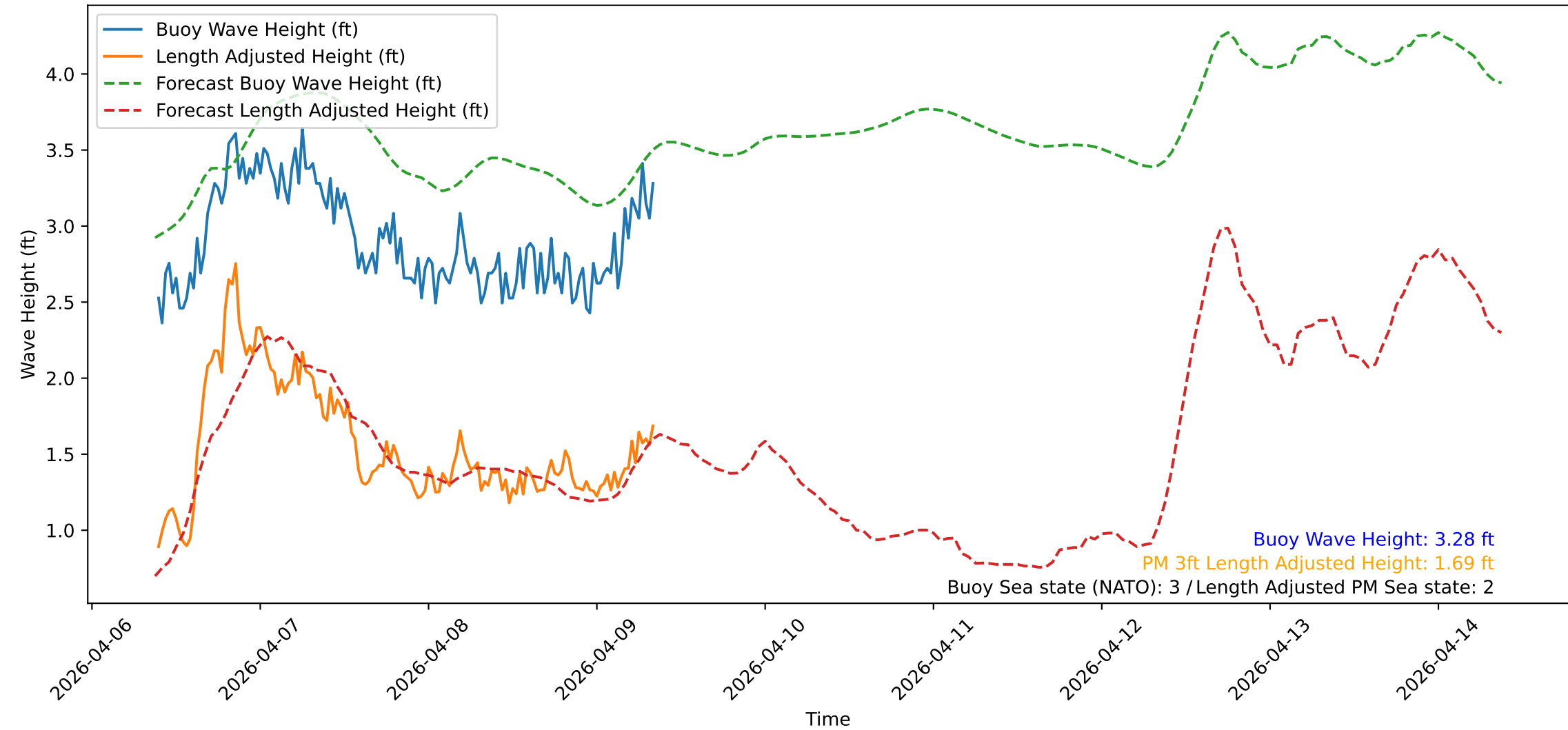
Wave Heights over Time for Oceanside Harbor at 2026-04-09 09:20:32
