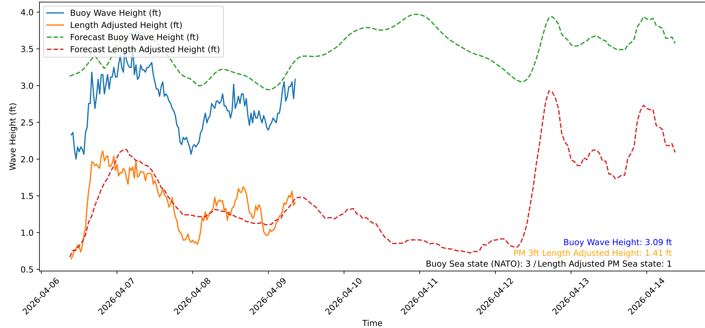
Wave Heights over Time for Red Beach at 2026-04-09 09:20:48
