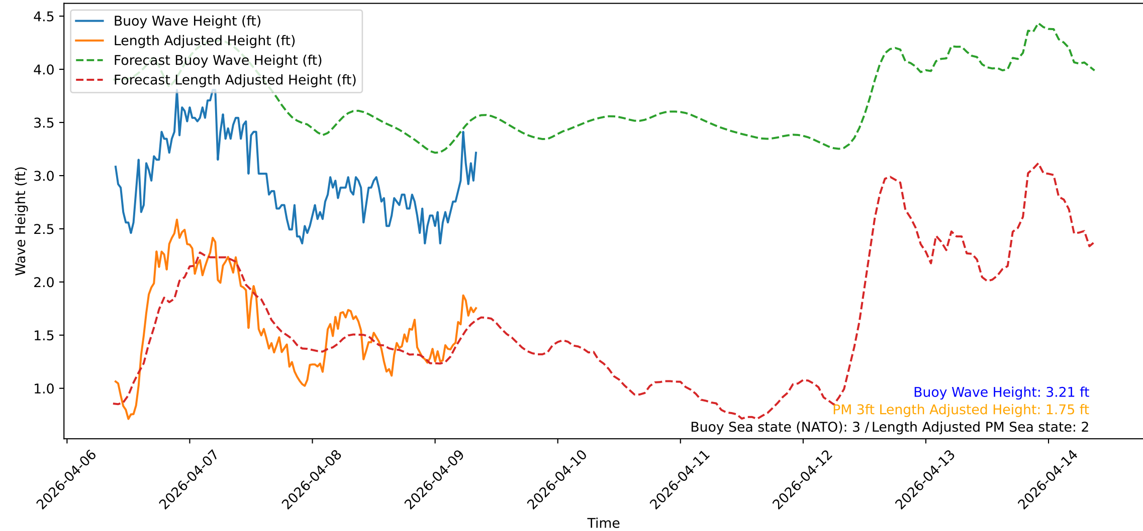
Wave Heights over Time for Green Beach at 2026-04-09 09:21:10
