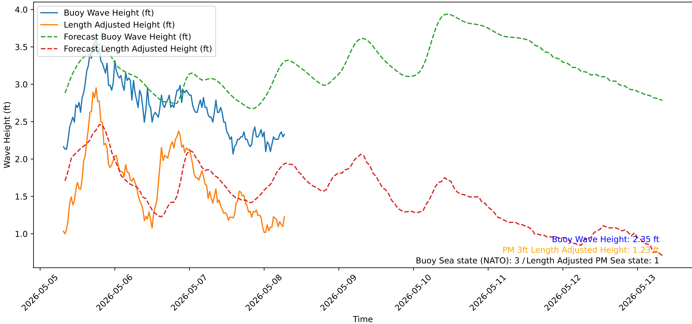
Wave Heights over Time for Green Beach at 2026-05-08 07:31:13
