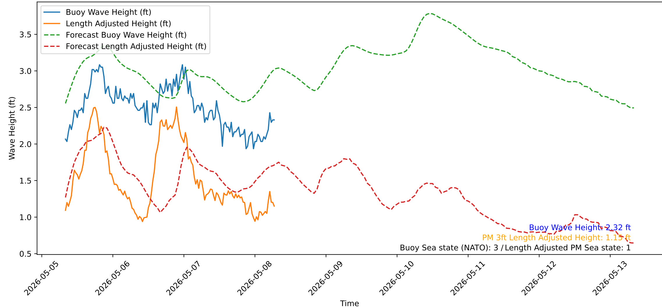
Wave Heights over Time for Red Beach at 2026-05-08 07:30:51
