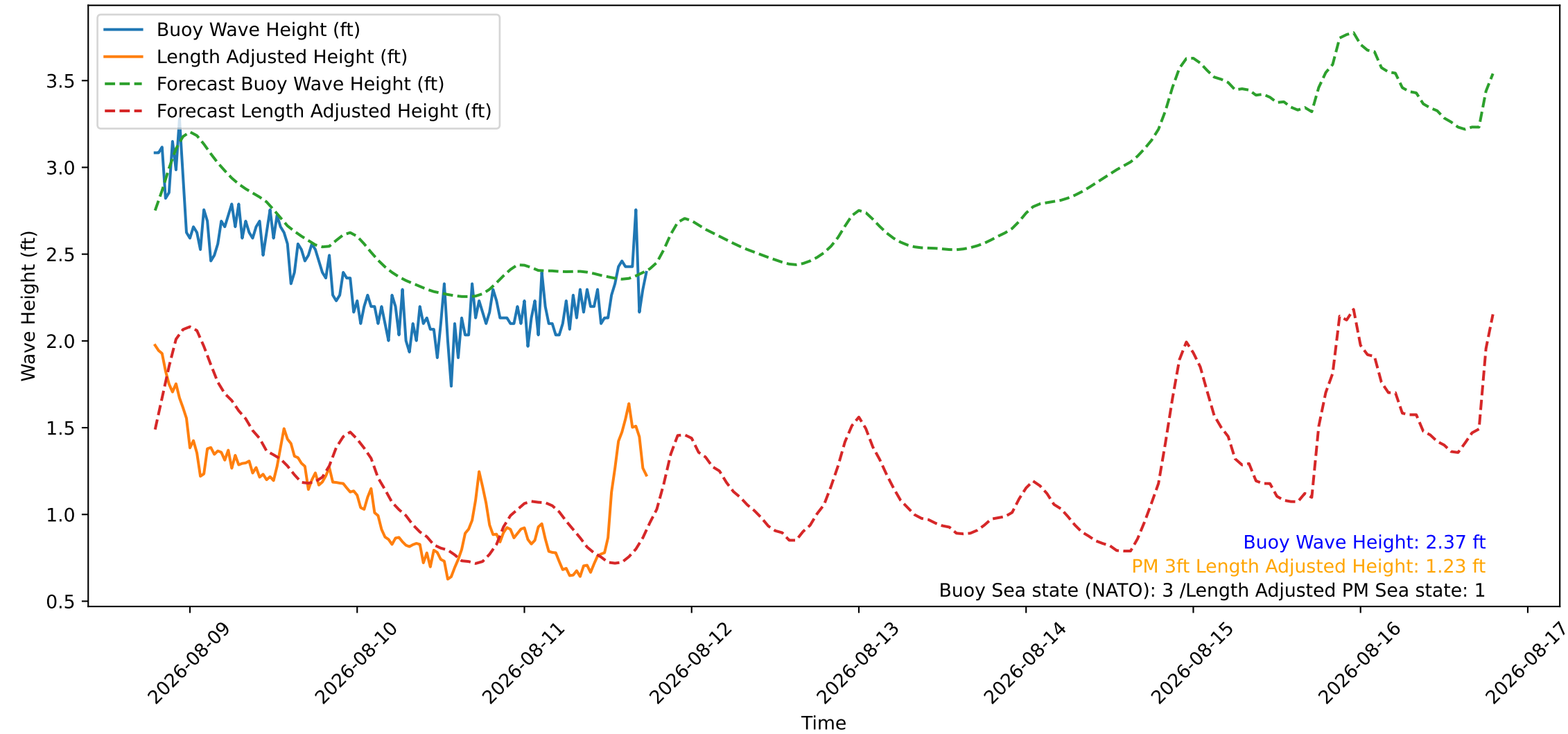
Wave Heights over Time for Red Beach at 2026-08-11 18:40:46
