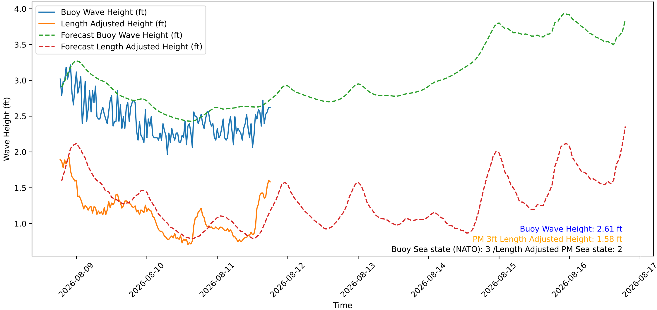
Wave Heights over Time for Oceanside Harbor at 2026-08-11 18:40:26
