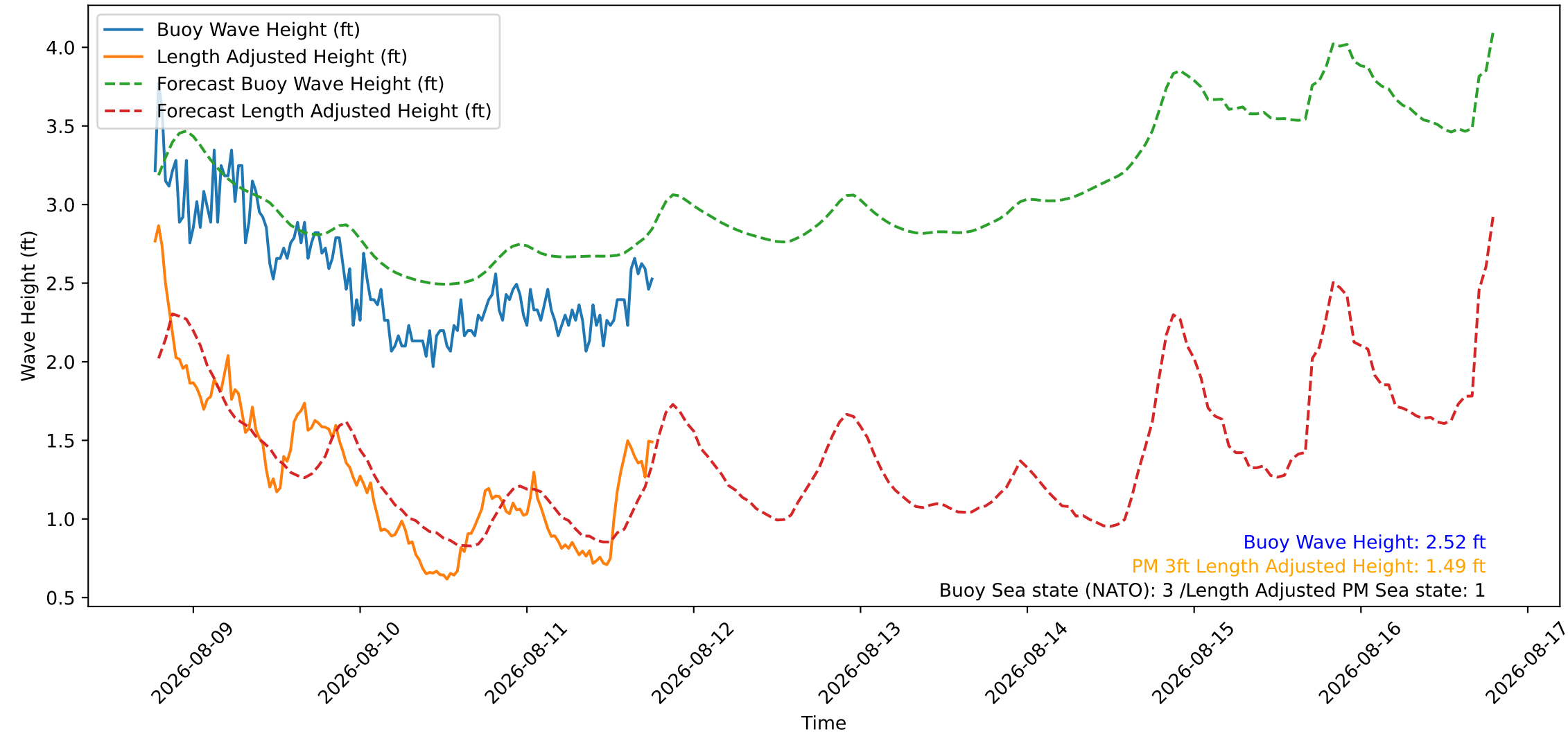
Wave Heights over Time for Green Beach at 2026-08-11 18:41:09
