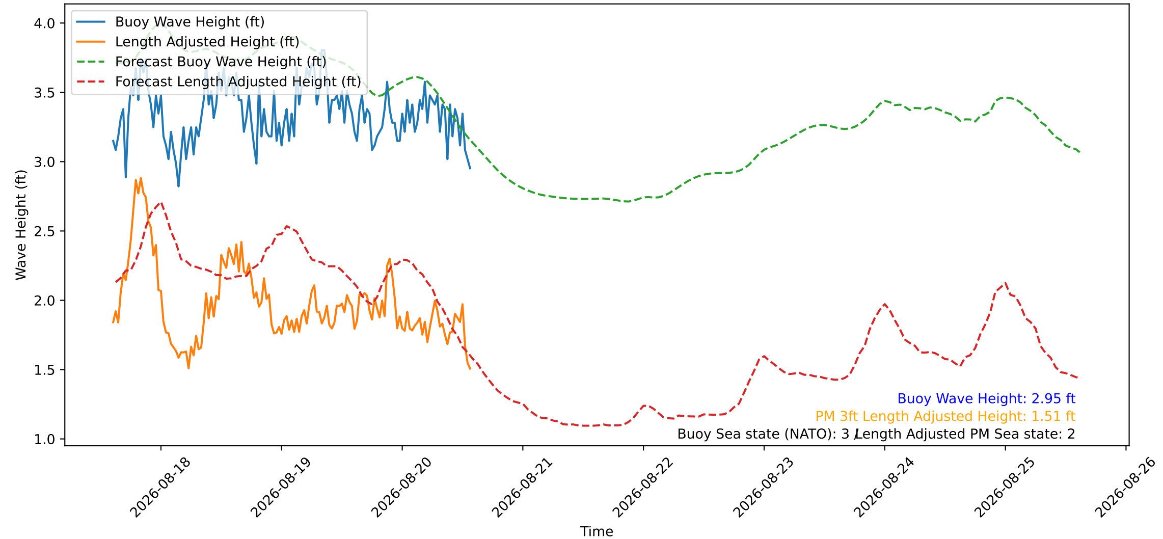
Wave Heights over Time for Oceanside Harbor at 2026-08-20 14:30:27
