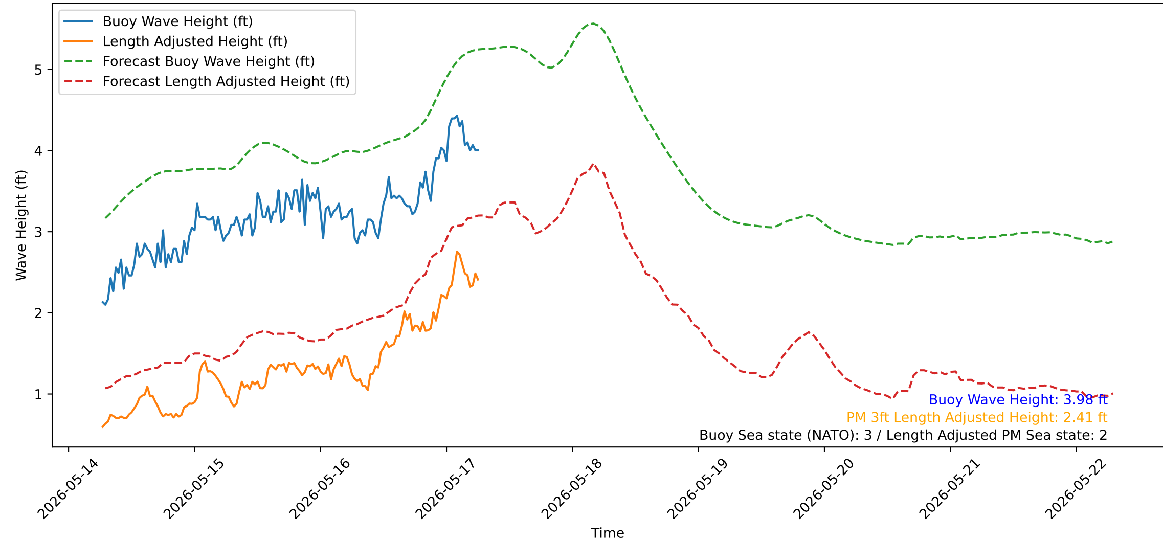
Wave Heights over Time for Green Beach at 2026-05-17 06:41:14
