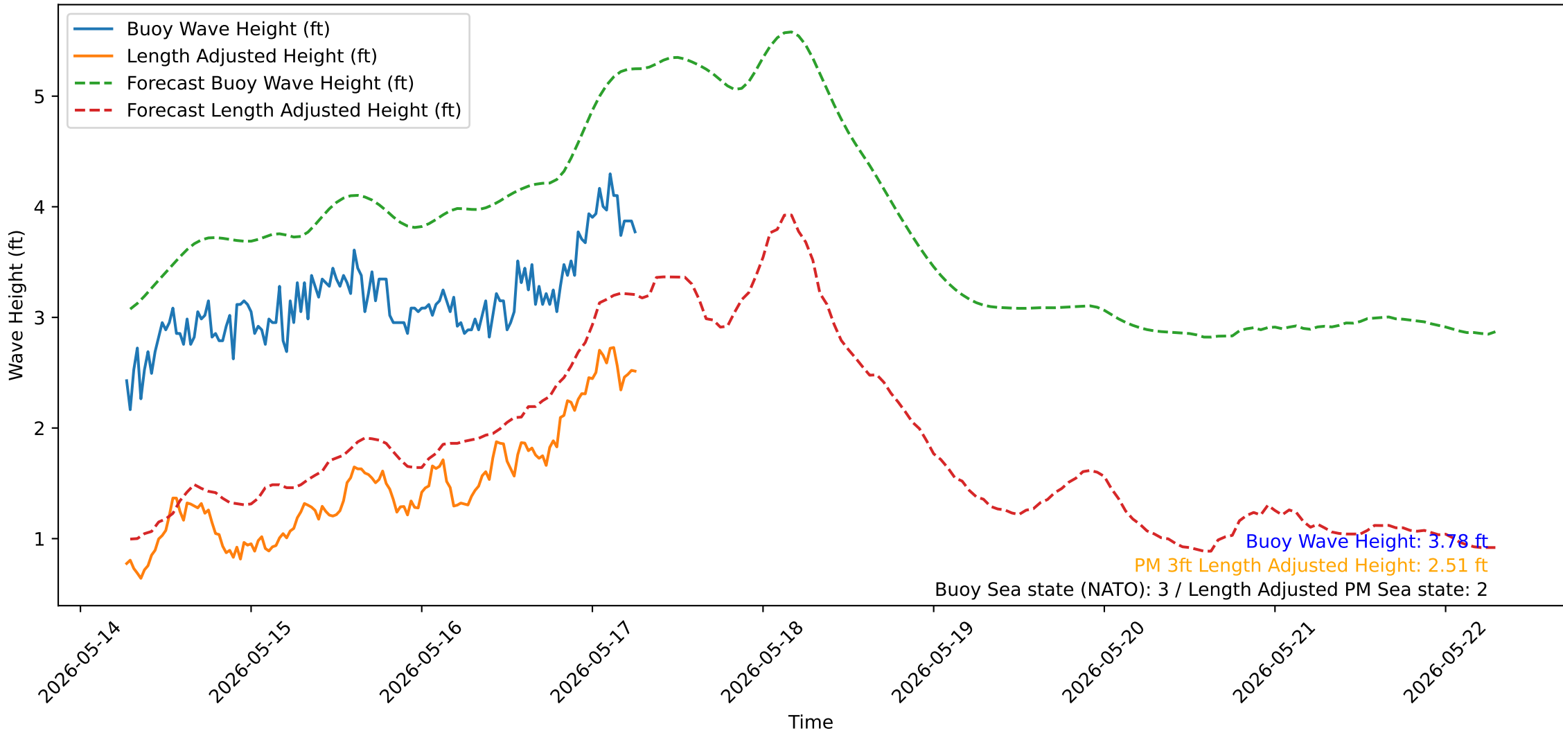
Wave Heights over Time for Oceanside Harbor at 2026-05-17 06:40:31
