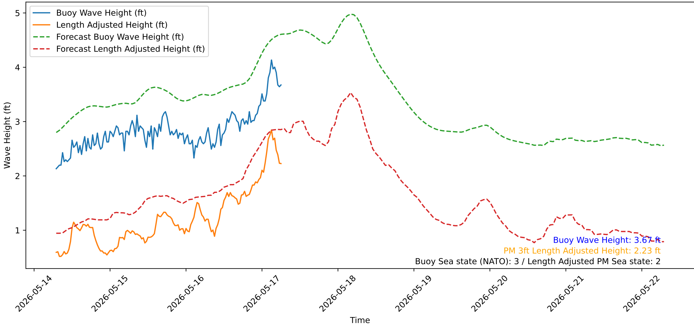
Wave Heights over Time for Red Beach at 2026-05-17 06:40:51
