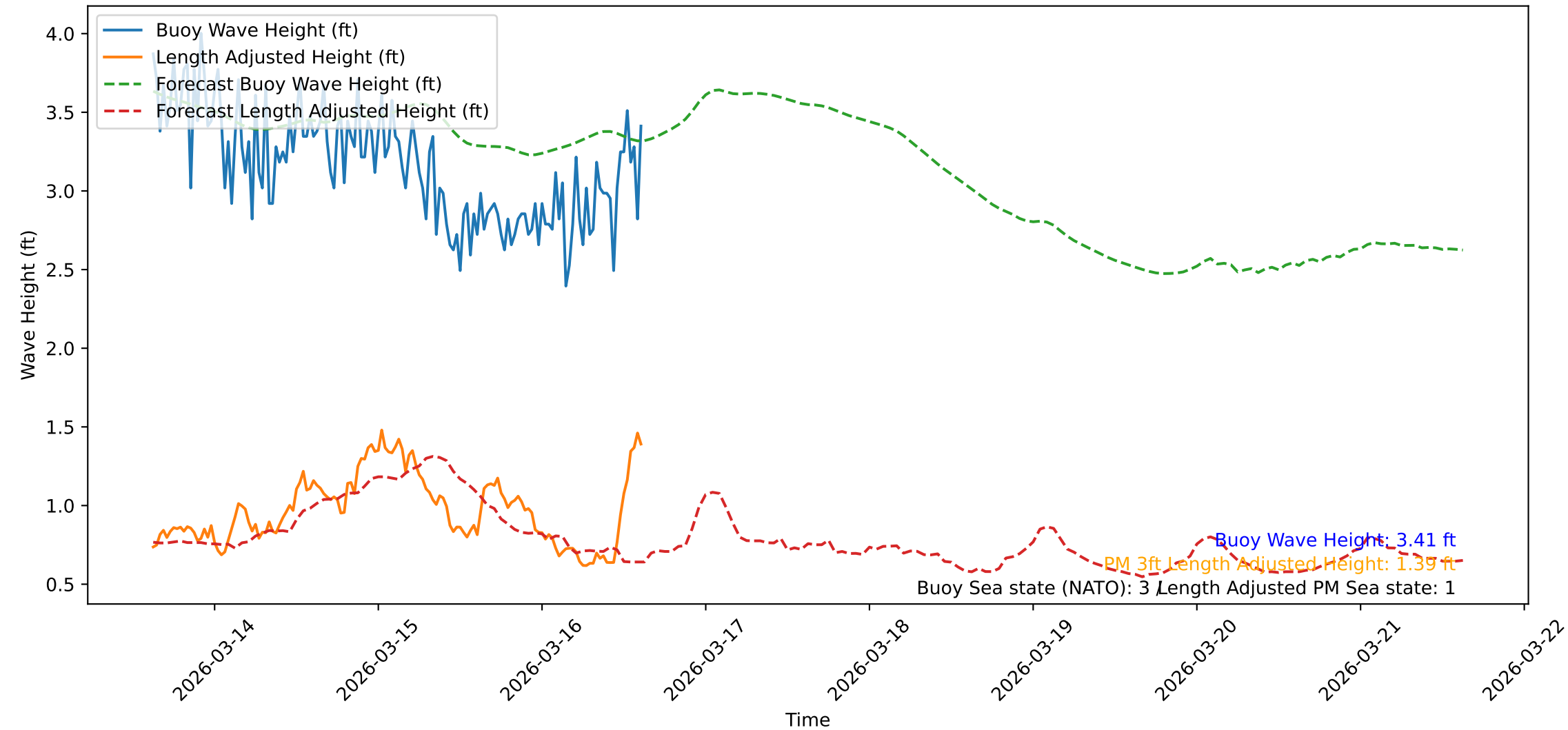
Wave Heights over Time for Oceanside Harbor at 2026-03-16 15:00:47
