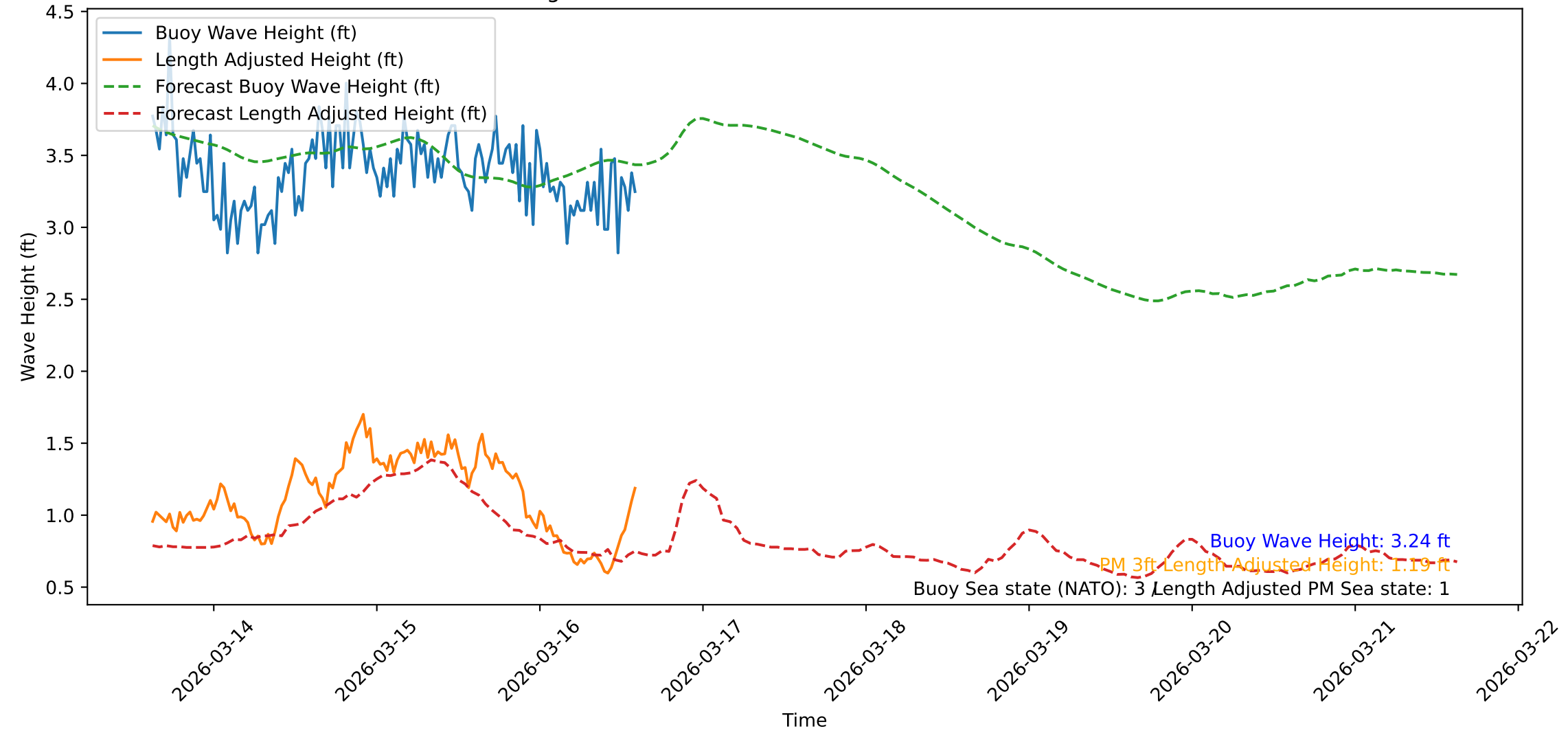
Wave Heights over Time for Green Beach at 2026-03-16 15:01:57
