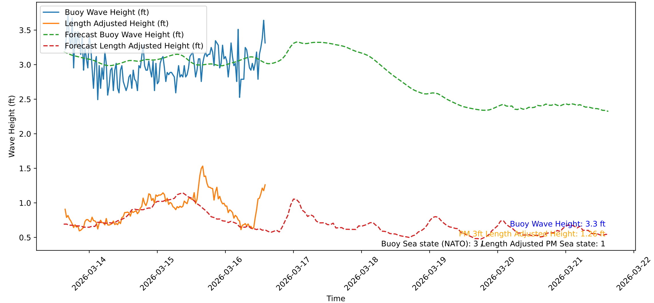
Wave Heights over Time for Red Beach at 2026-03-16 15:01:11
