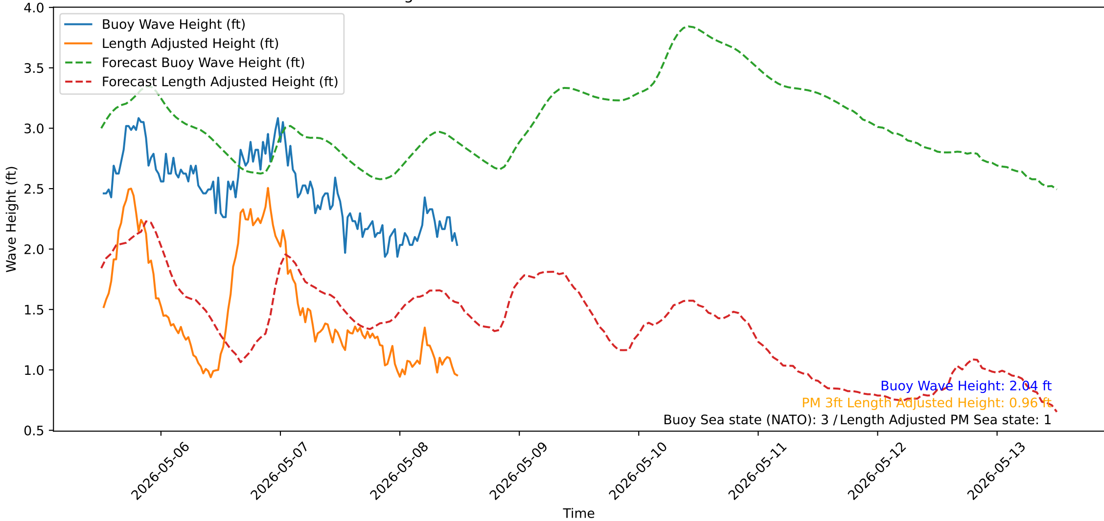
Wave Heights over Time for Red Beach at 2026-05-08 12:20:53
