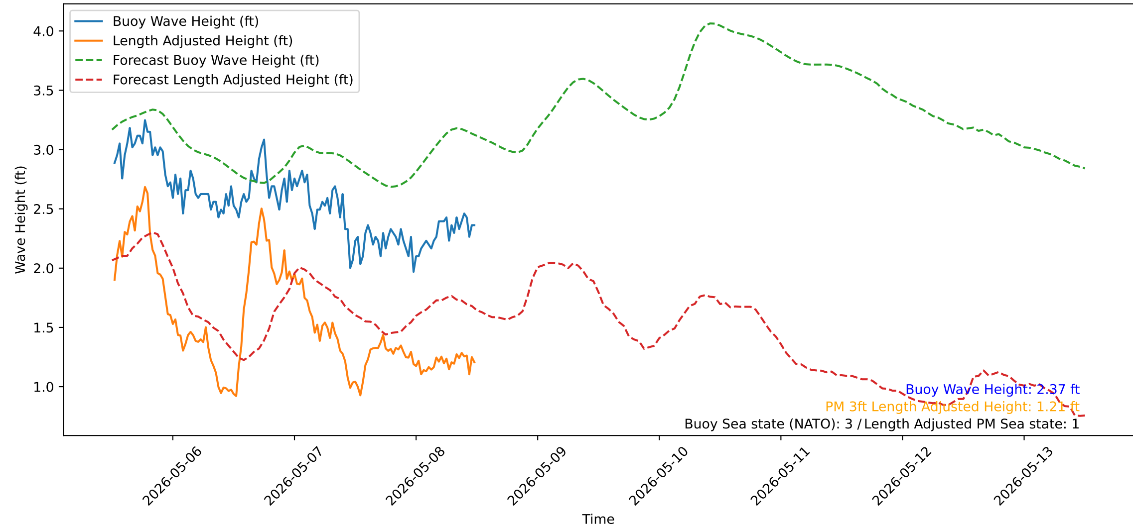
Wave Heights over Time for Oceanside Harbor at 2026-05-08 12:20:32
