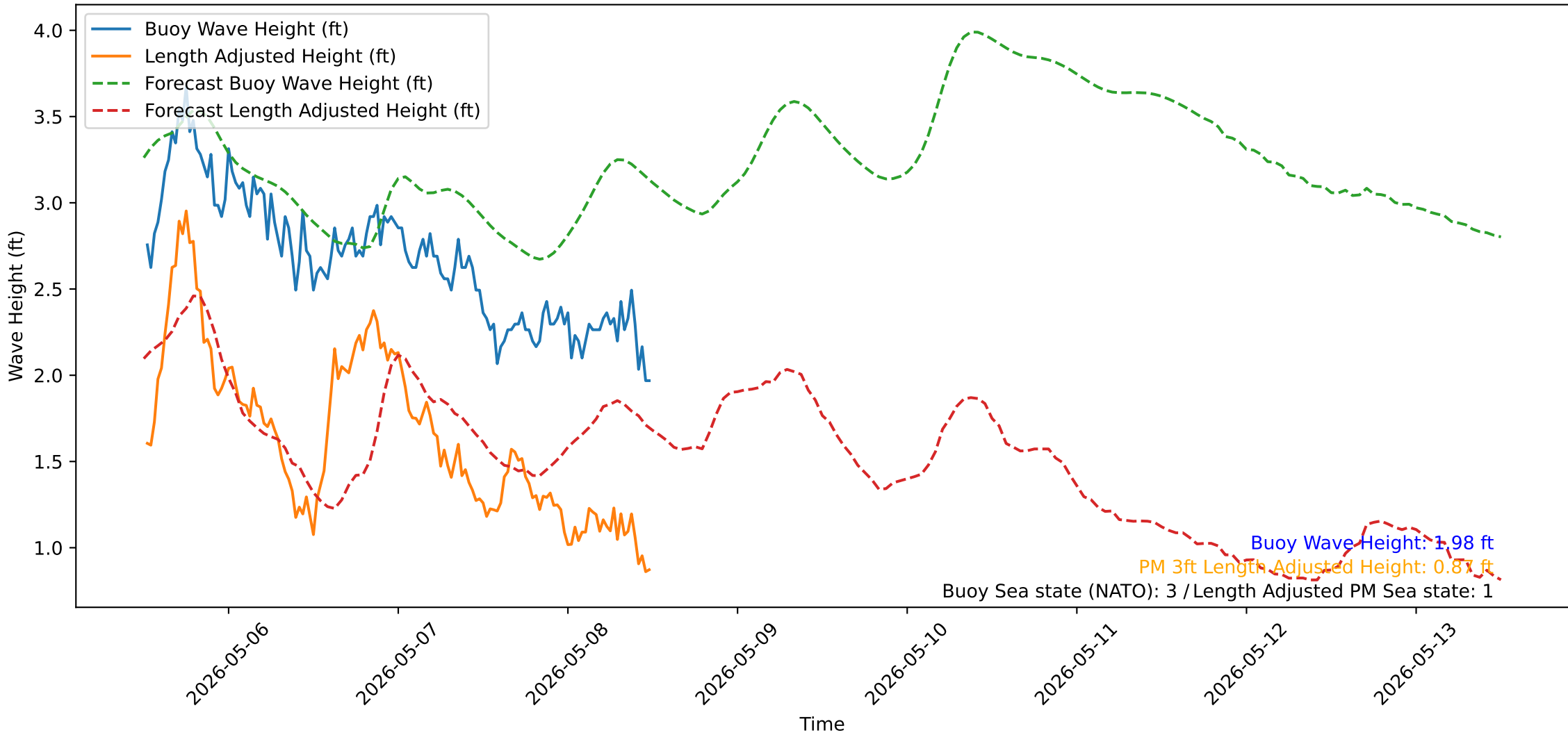
Wave Heights over Time for Green Beach at 2026-05-08 12:21:15
