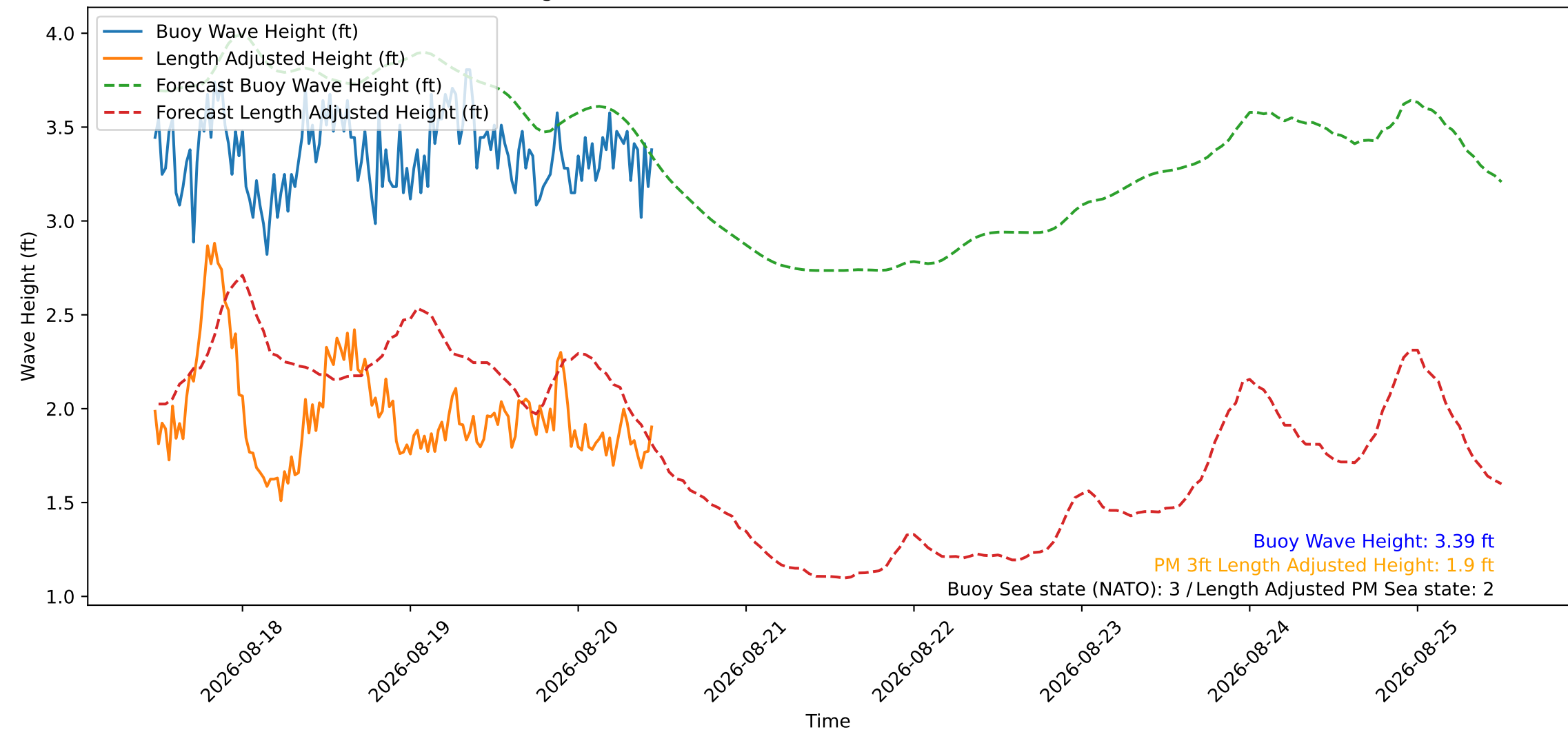
Wave Heights over Time for Oceanside Harbor at 2026-08-20 11:30:27
