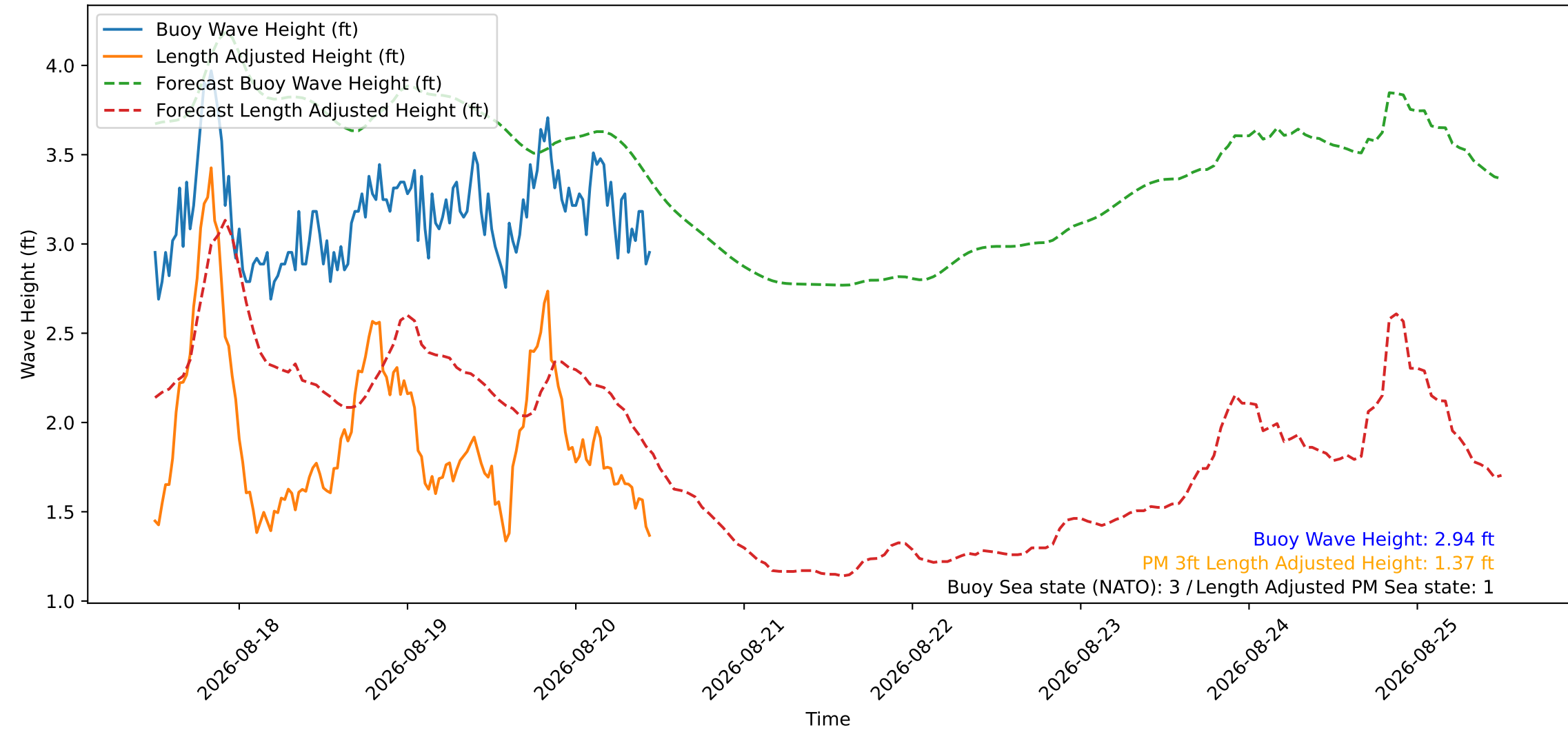
Wave Heights over Time for Green Beach at 2026-08-20 11:31:09
