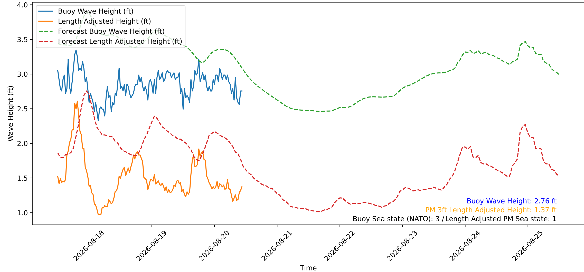
Wave Heights over Time for Red Beach at 2026-08-20 11:30:47
