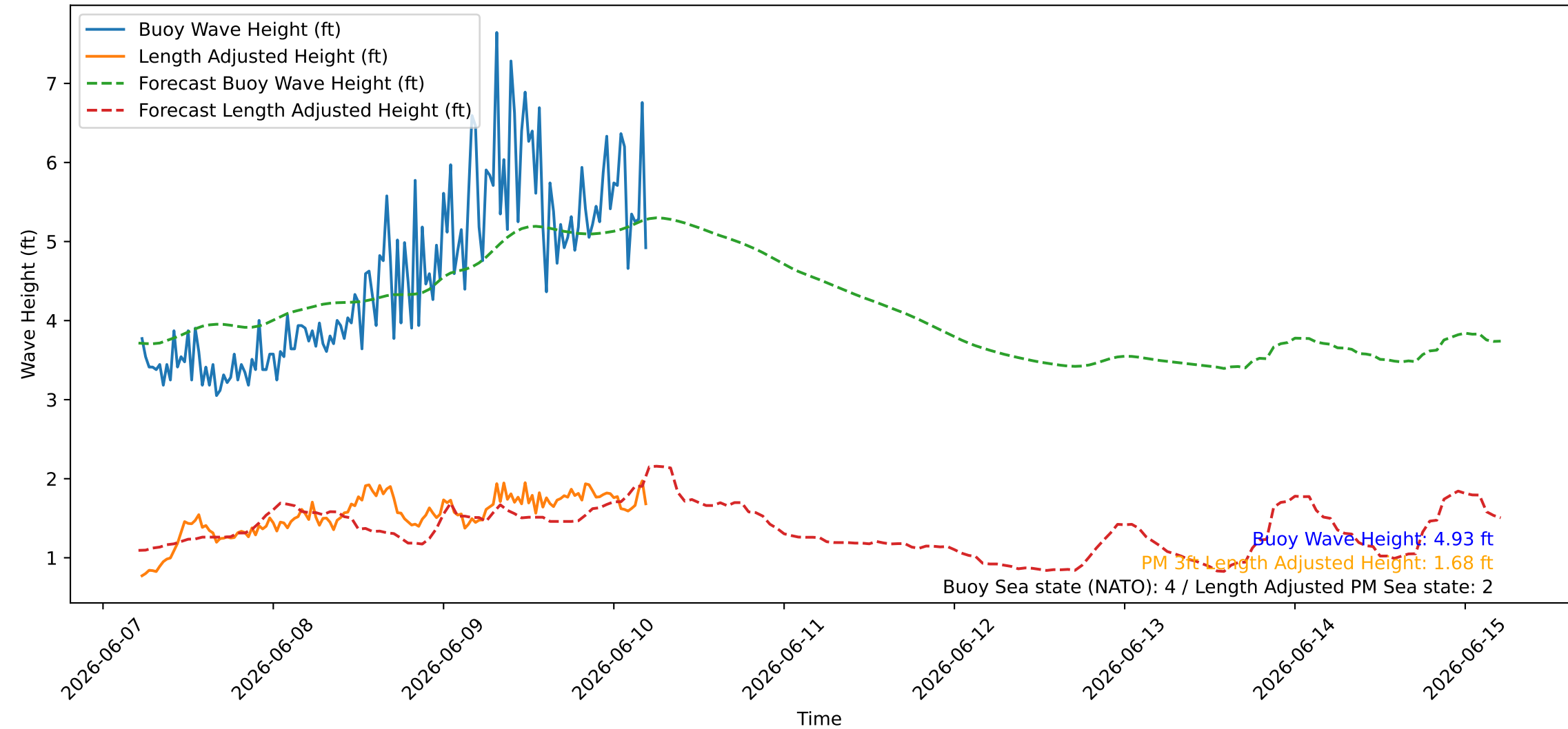
Wave Heights over Time for Red Beach at 2026-06-10 05:10:46
