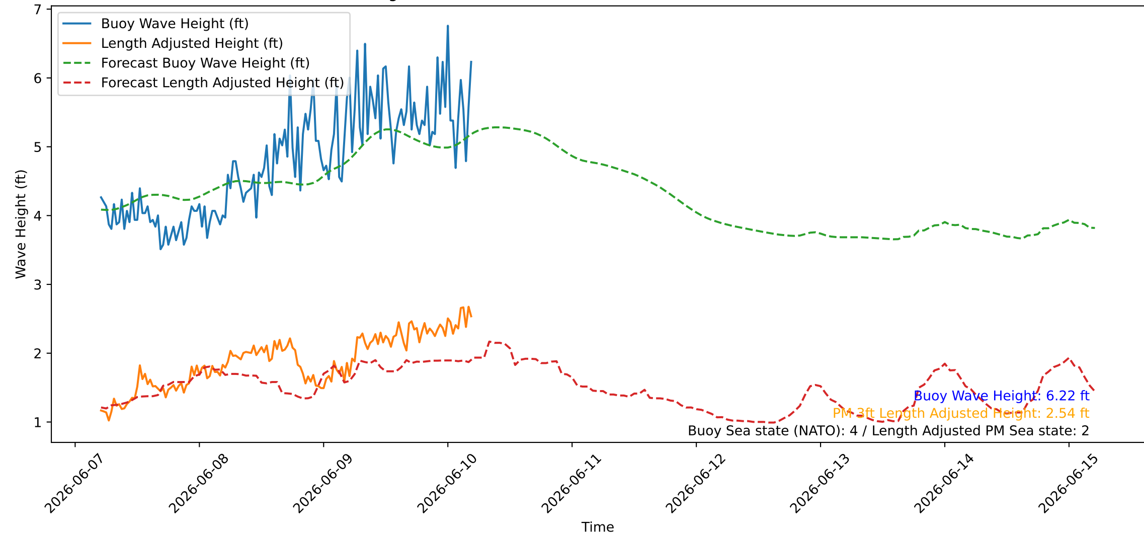
Wave Heights over Time for Oceanside Harbor at 2026-06-10 05:10:26
