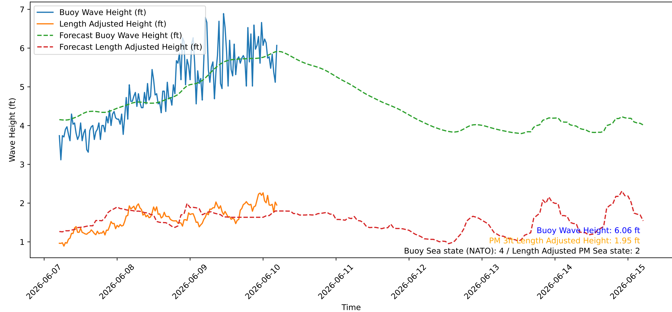
Wave Heights over Time for Green Beach at 2026-06-10 05:11:10
