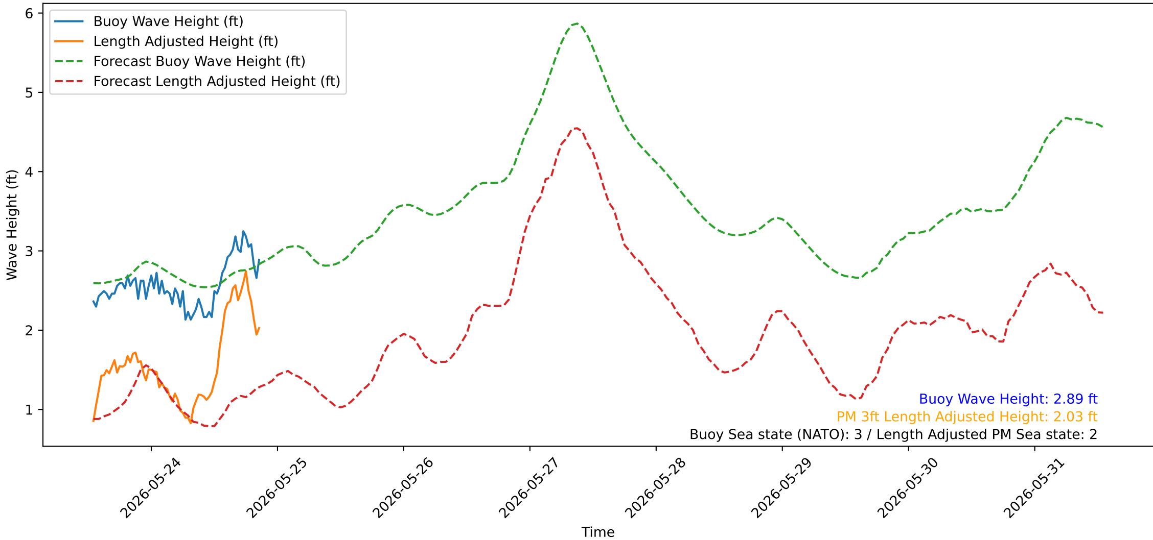
Wave Heights over Time for Oceanside Harbor at 2026-05-26 13:10:28
