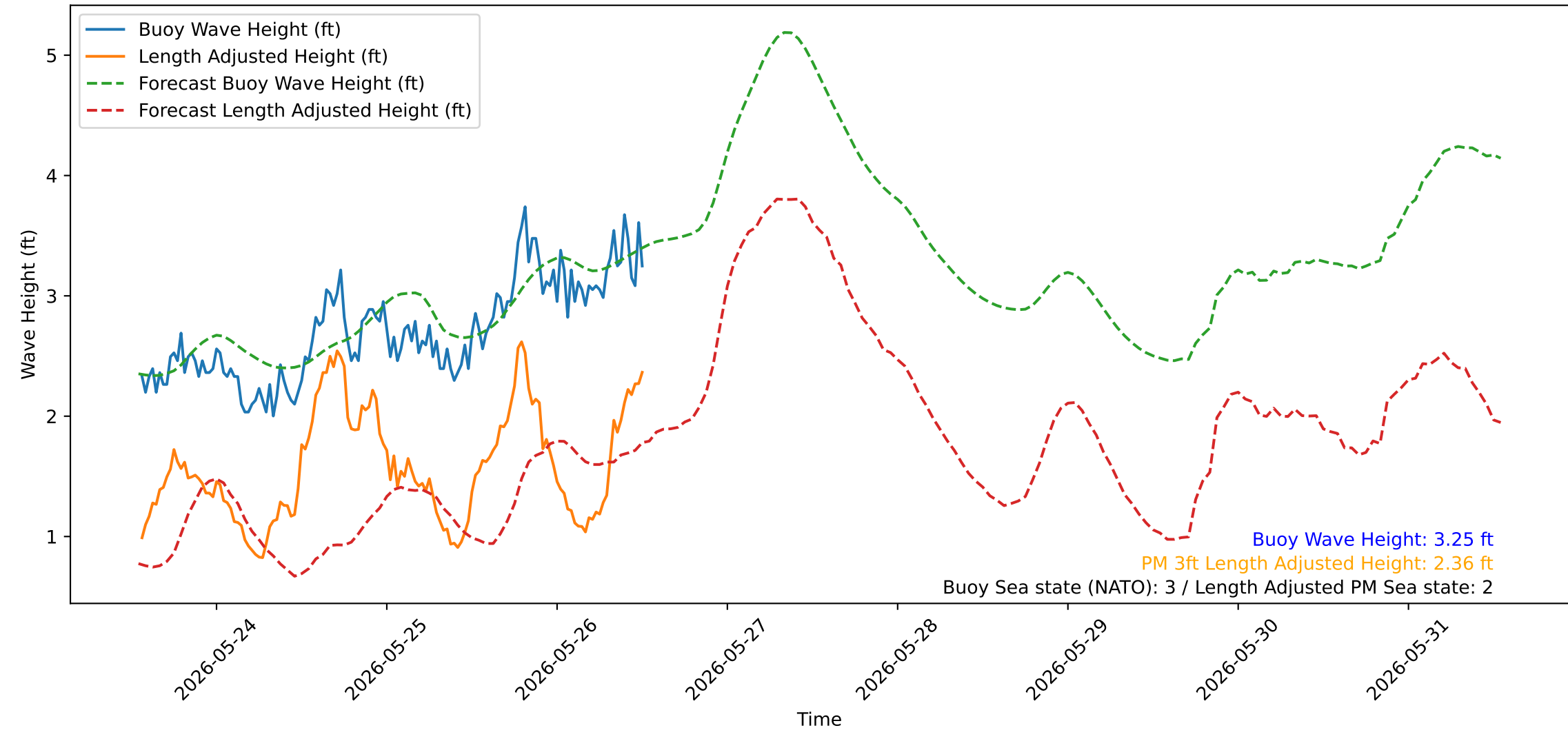
Wave Heights over Time for Red Beach at 2026-05-26 13:10:47
