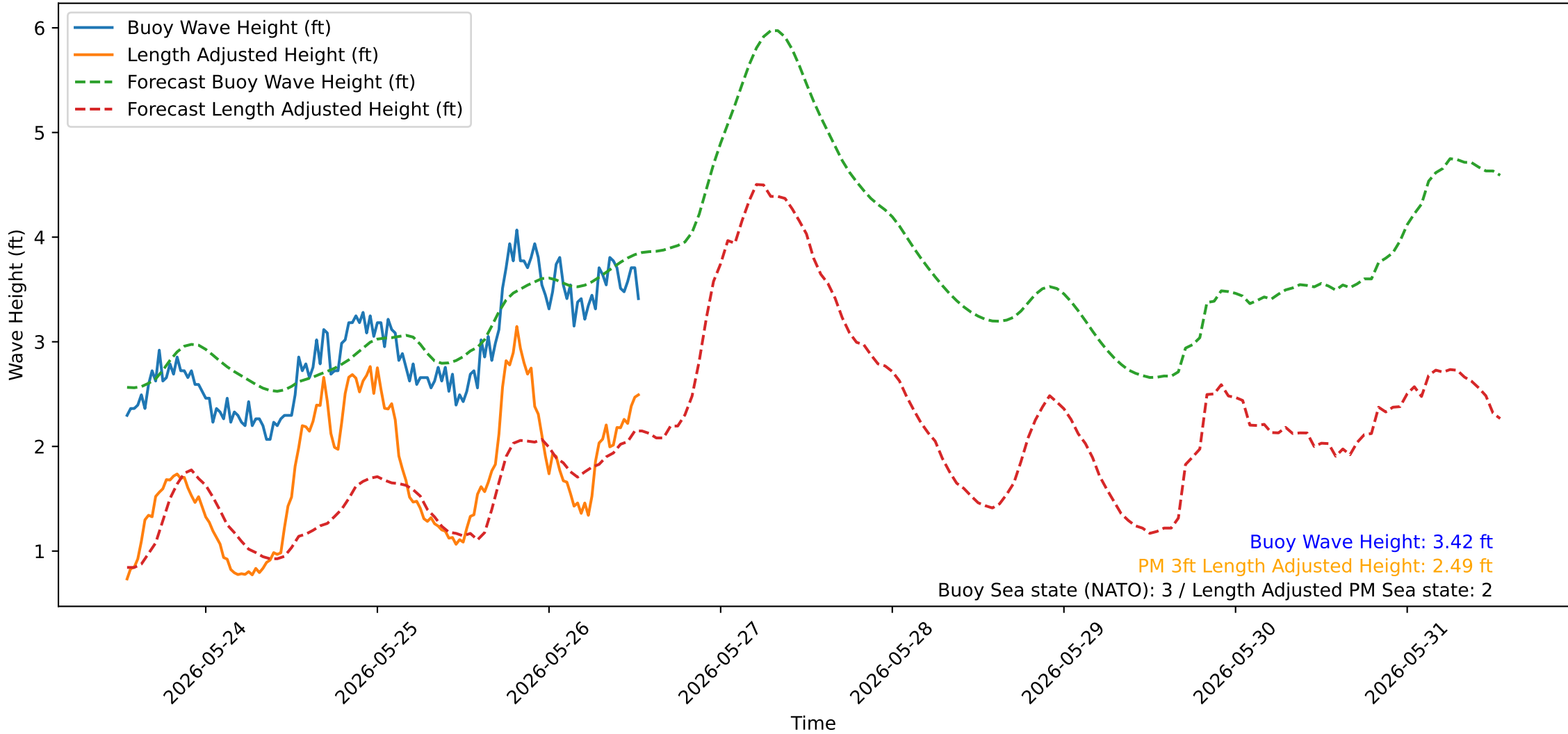
Wave Heights over Time for Green Beach at 2026-05-26 13:11:10
