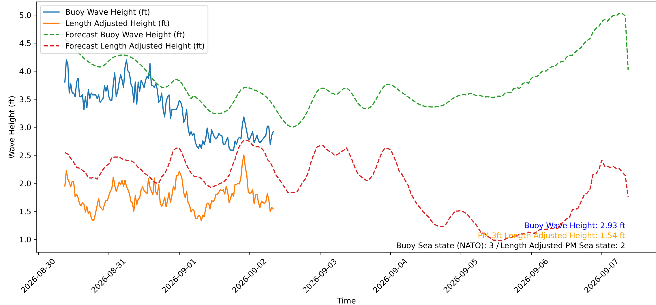
Wave Heights over Time for Red Beach at 2026-09-02 08:50:51
