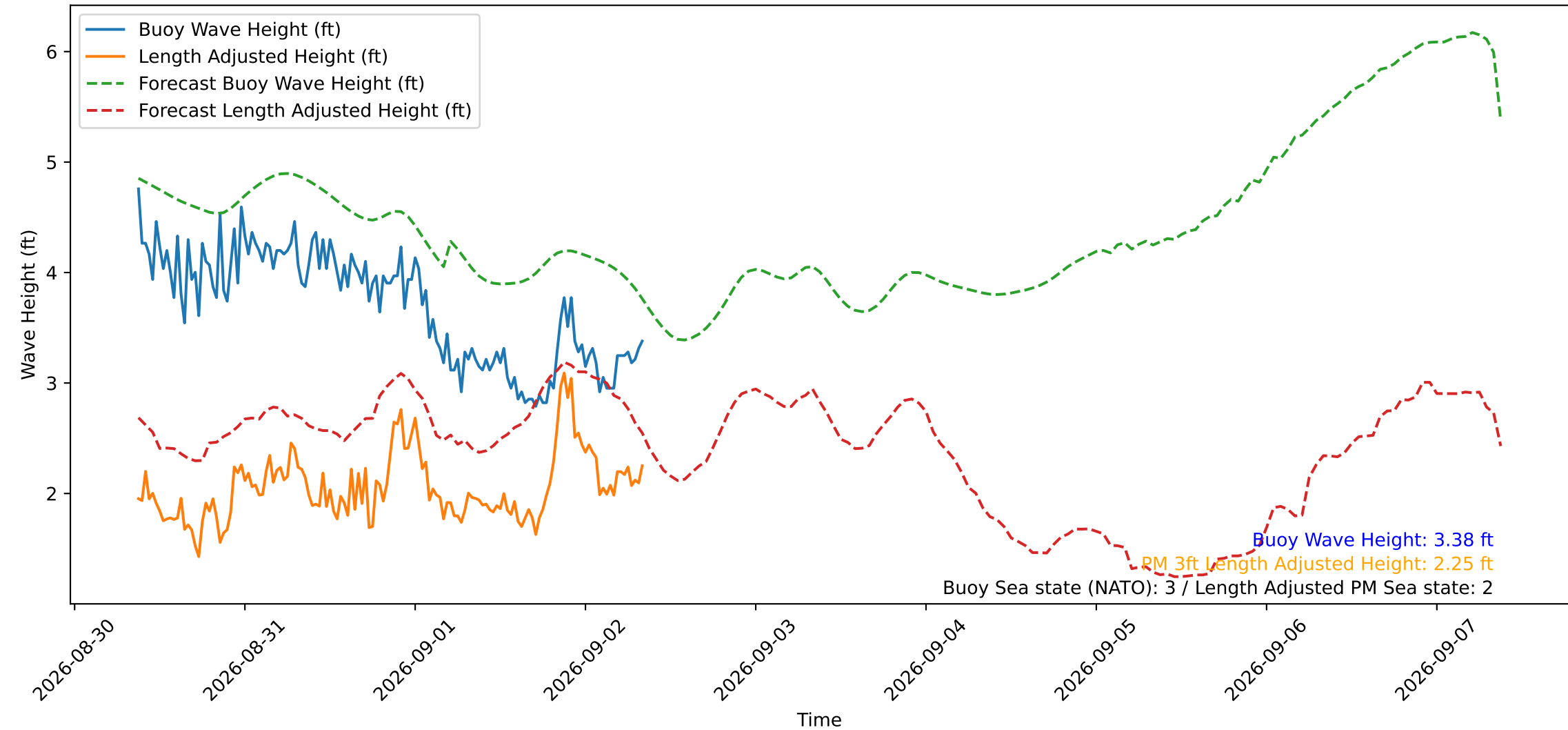
Wave Heights over Time for Green Beach at 2026-09-02 08:51:15
