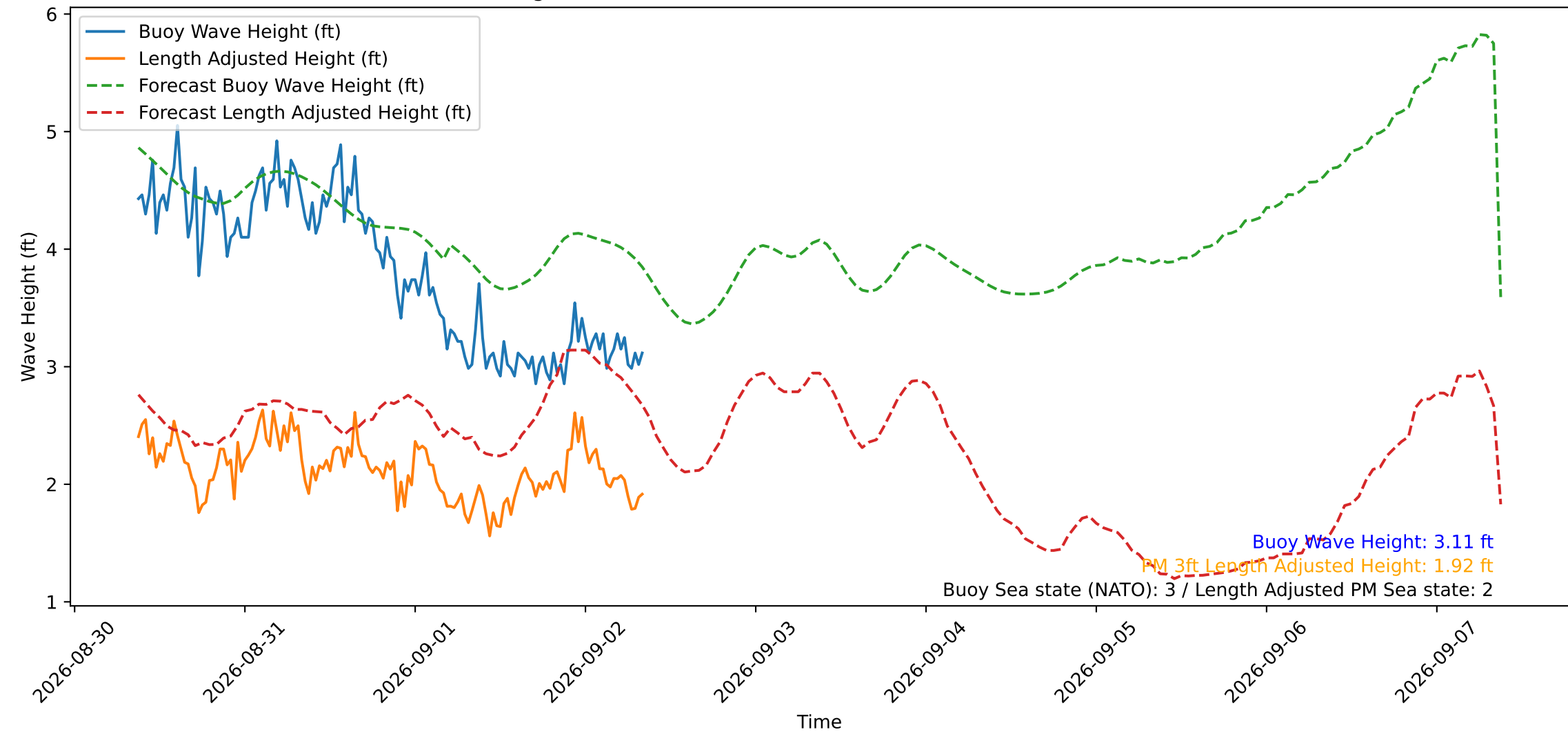
Wave Heights over Time for Oceanside Harbor at 2026-09-02 08:50:29
