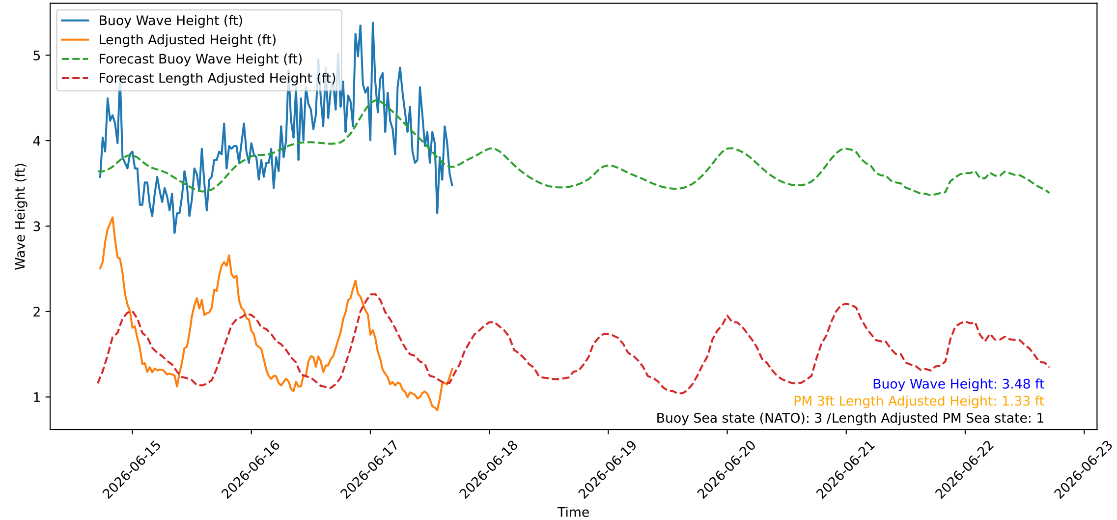
Wave Heights over Time for Red Beach at 2026-06-17 17:10:45
