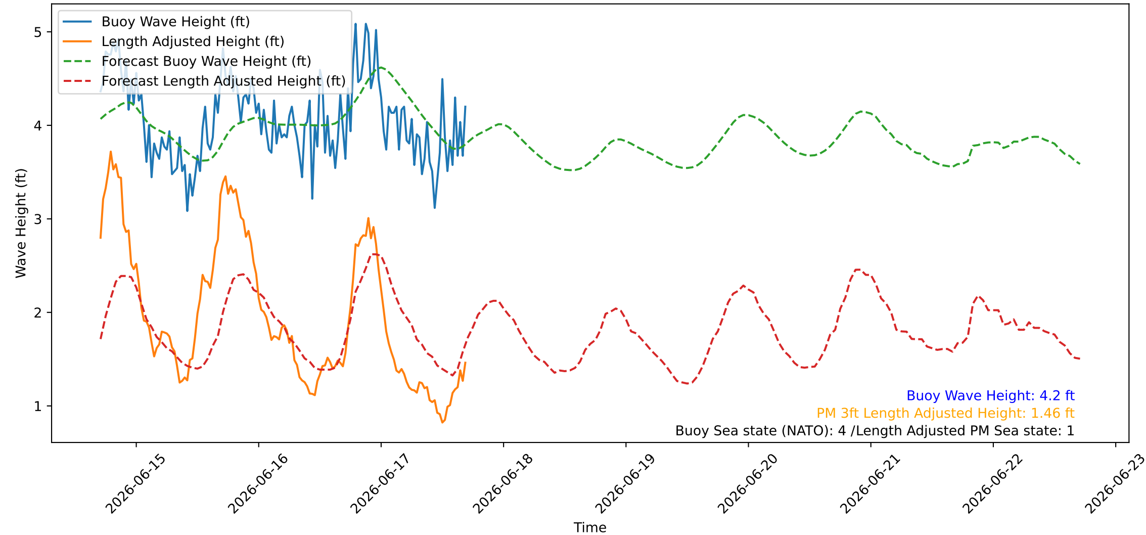
Wave Heights over Time for Green Beach at 2026-06-17 17:11:08
