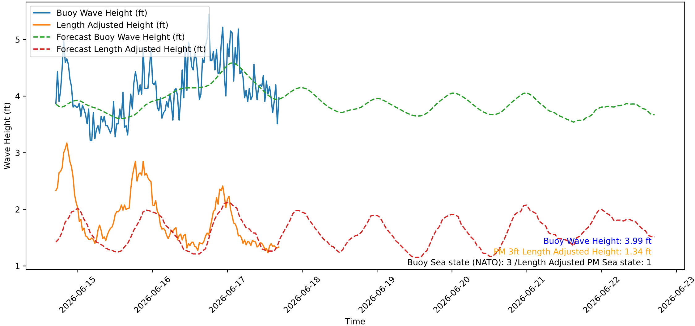
Wave Heights over Time for Oceanside Harbor at 2026-06-17 17:10:26
