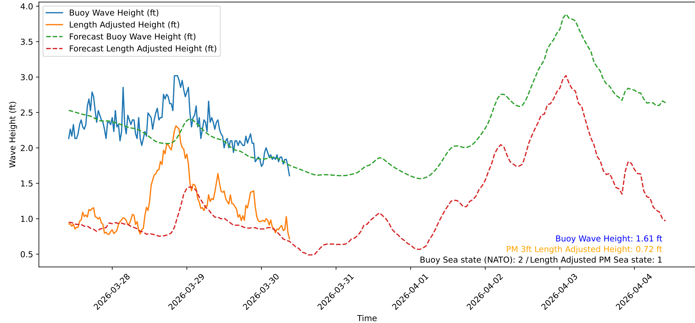
Wave Heights over Time for Red Beach at 2026-03-30 09:40:47
