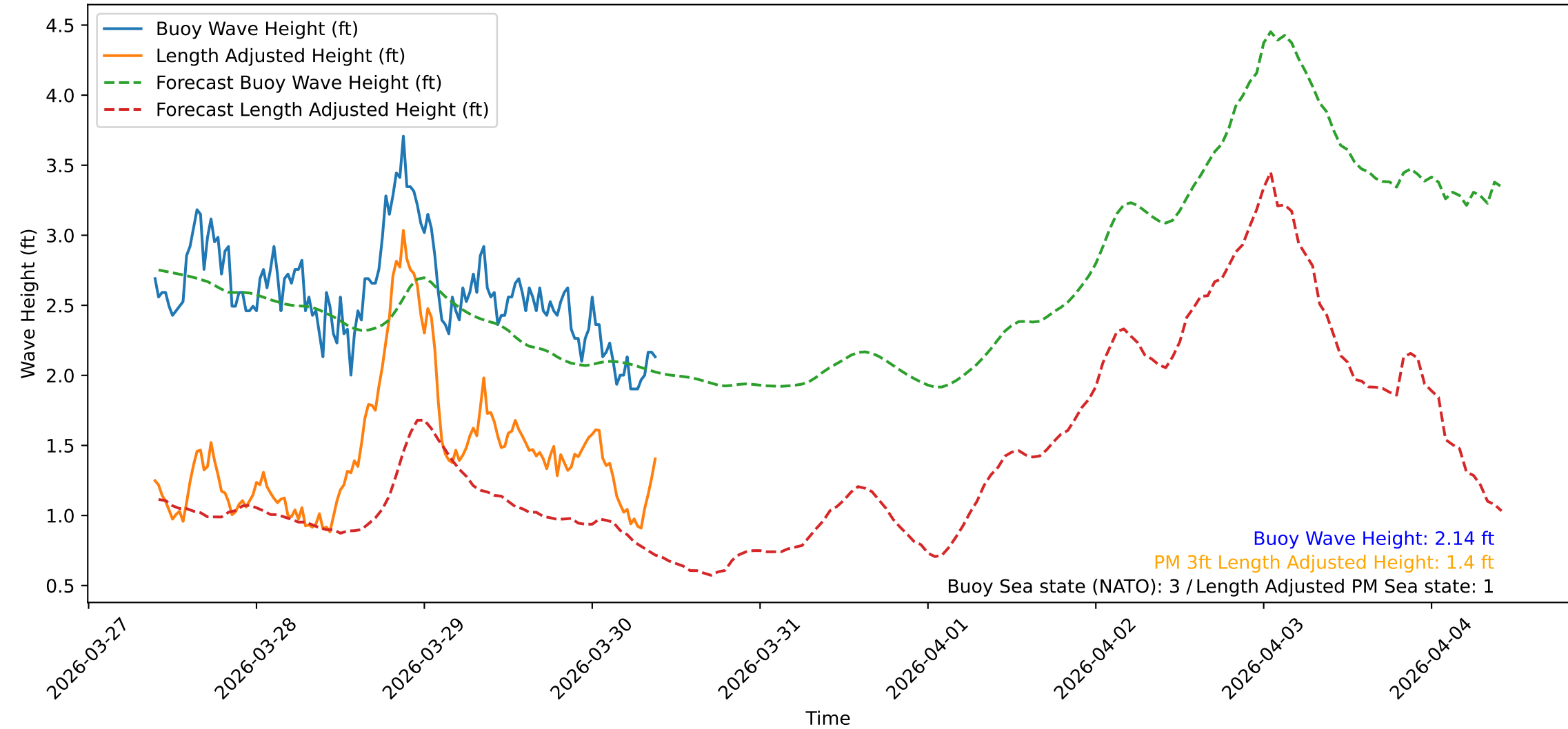
Wave Heights over Time for Green Beach at 2026-03-30 09:41:09
