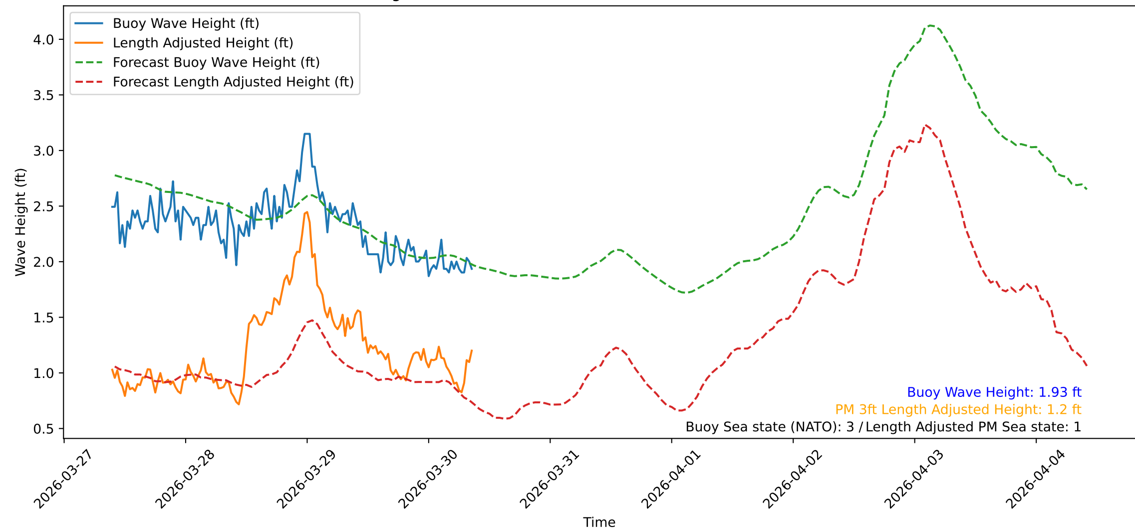
Wave Heights over Time for Oceanside Harbor at 2026-03-30 09:40:31
