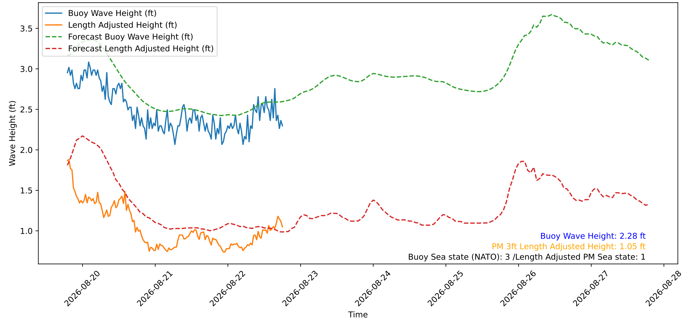
Wave Heights over Time for Red Beach at 2026-08-22 18:50:51
