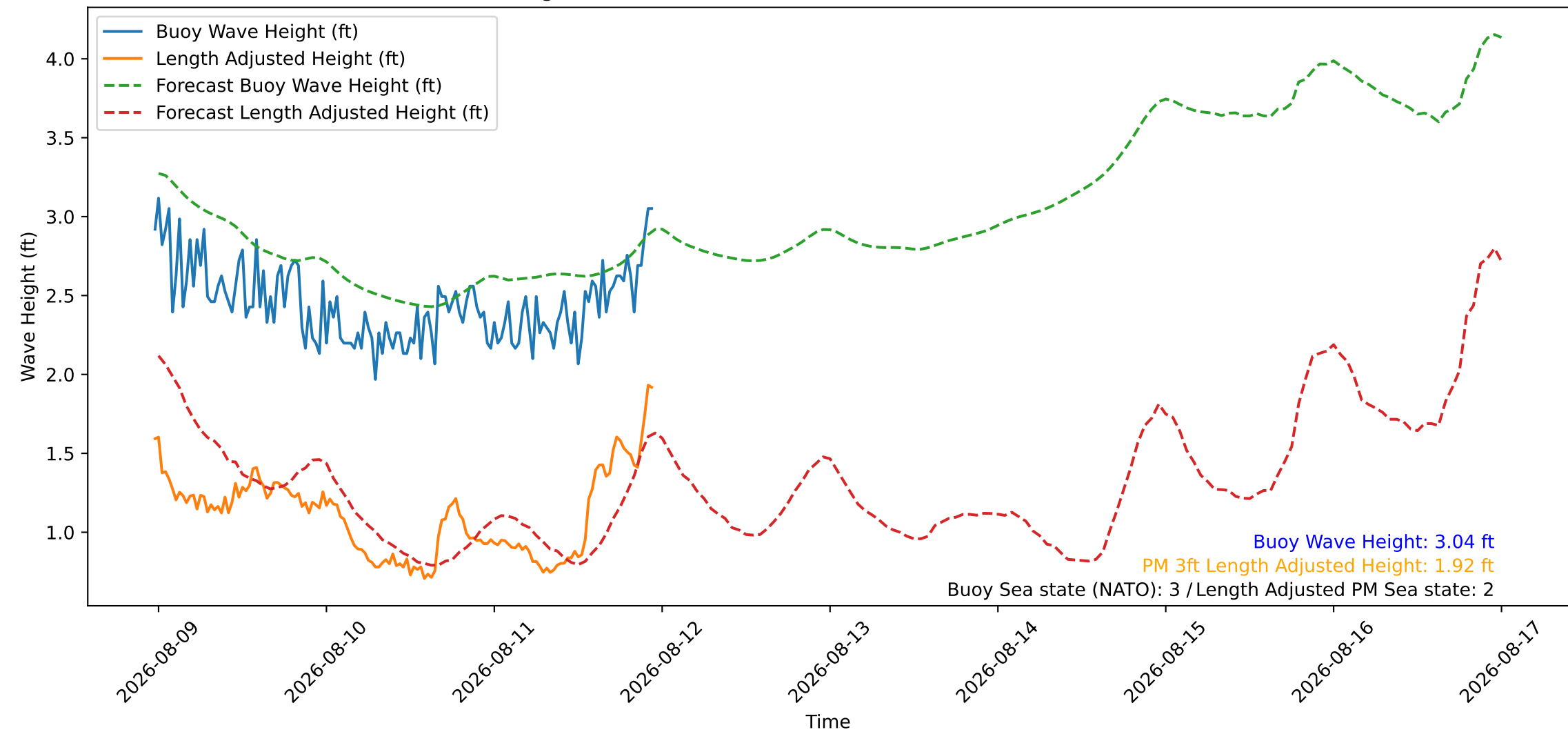
Wave Heights over Time for Oceanside Harbor at 2026-08-11 23:30:26
