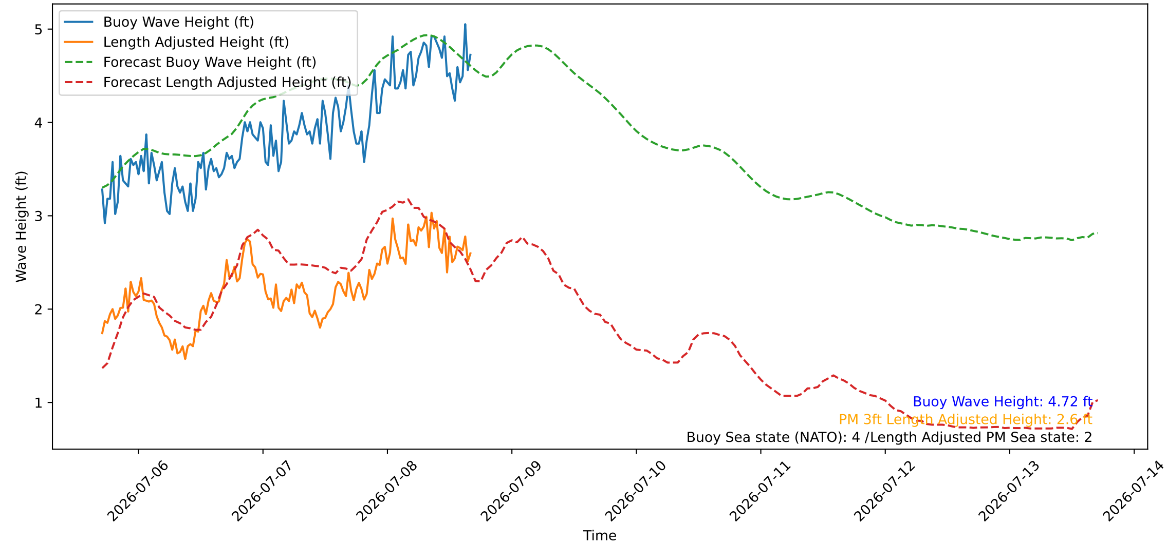
Wave Heights over Time for Oceanside Harbor at 2026-07-08 16:50:27
