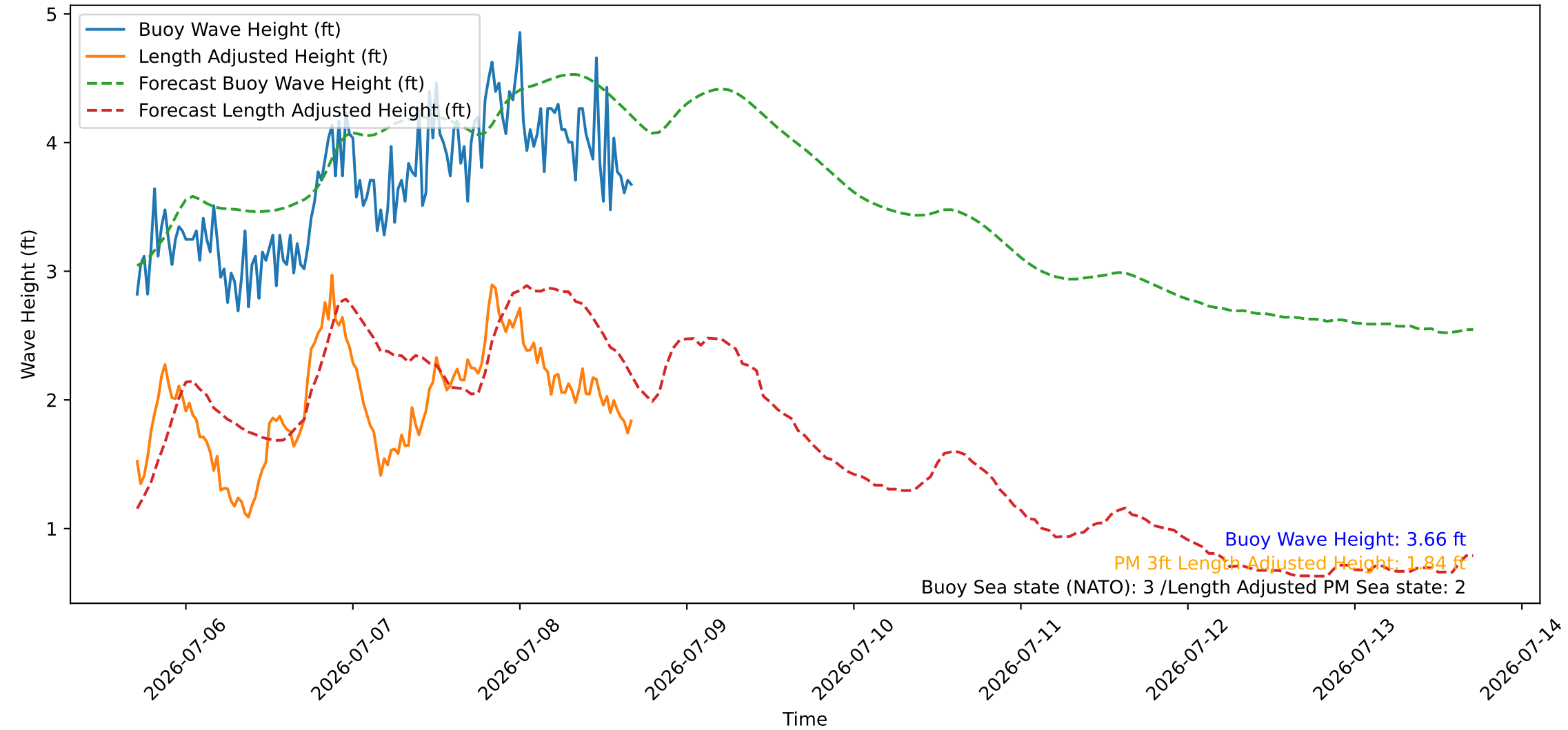
Wave Heights over Time for Red Beach at 2026-07-08 16:50:48
