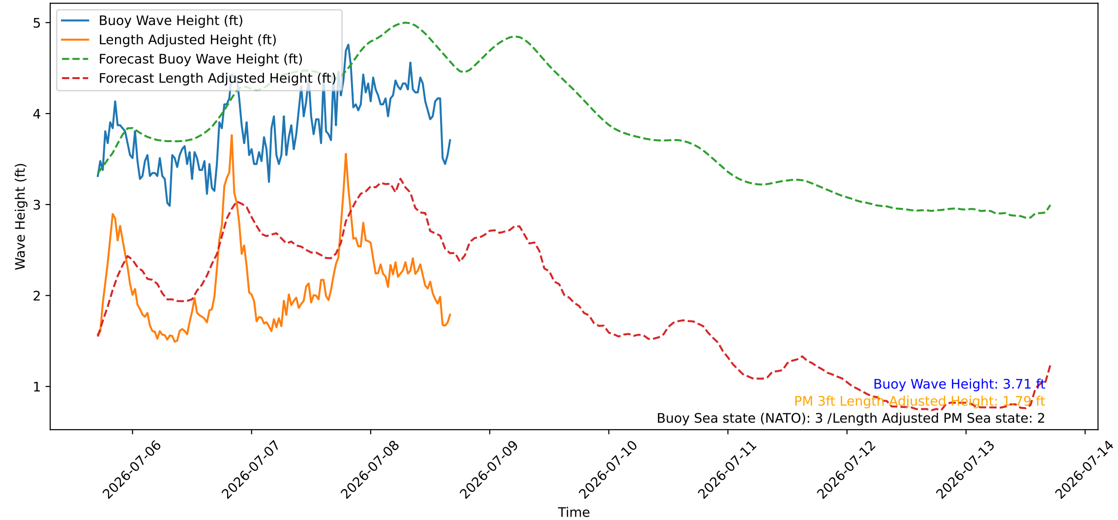
Wave Heights over Time for Green Beach at 2026-07-08 16:51:10
