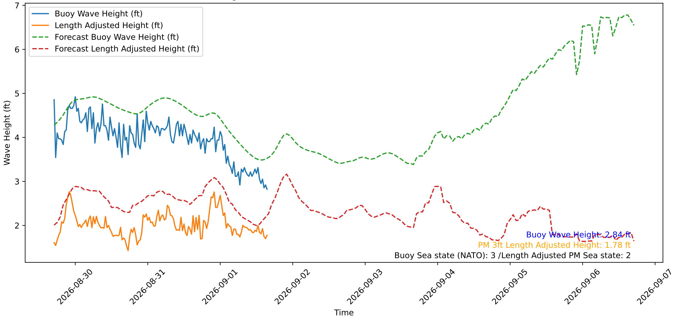
Wave Heights over Time for Green Beach at 2026-09-01 16:31:12
