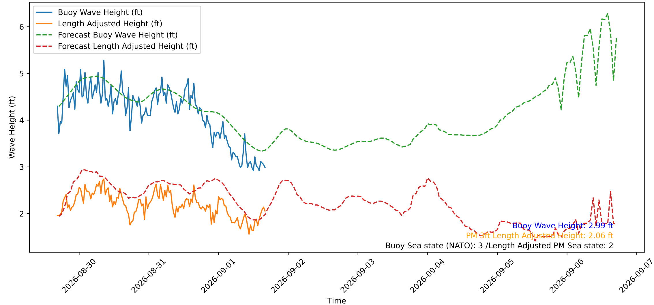
Wave Heights over Time for Oceanside Harbor at 2026-09-01 16:30:30
