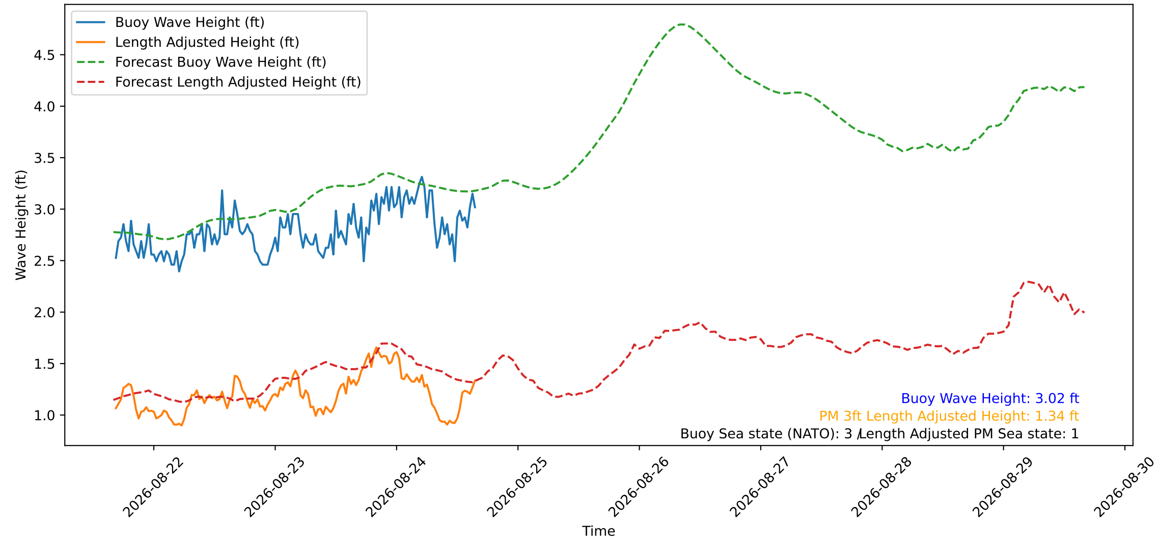
Wave Heights over Time for Green Beach at 2026-08-24 16:11:11
