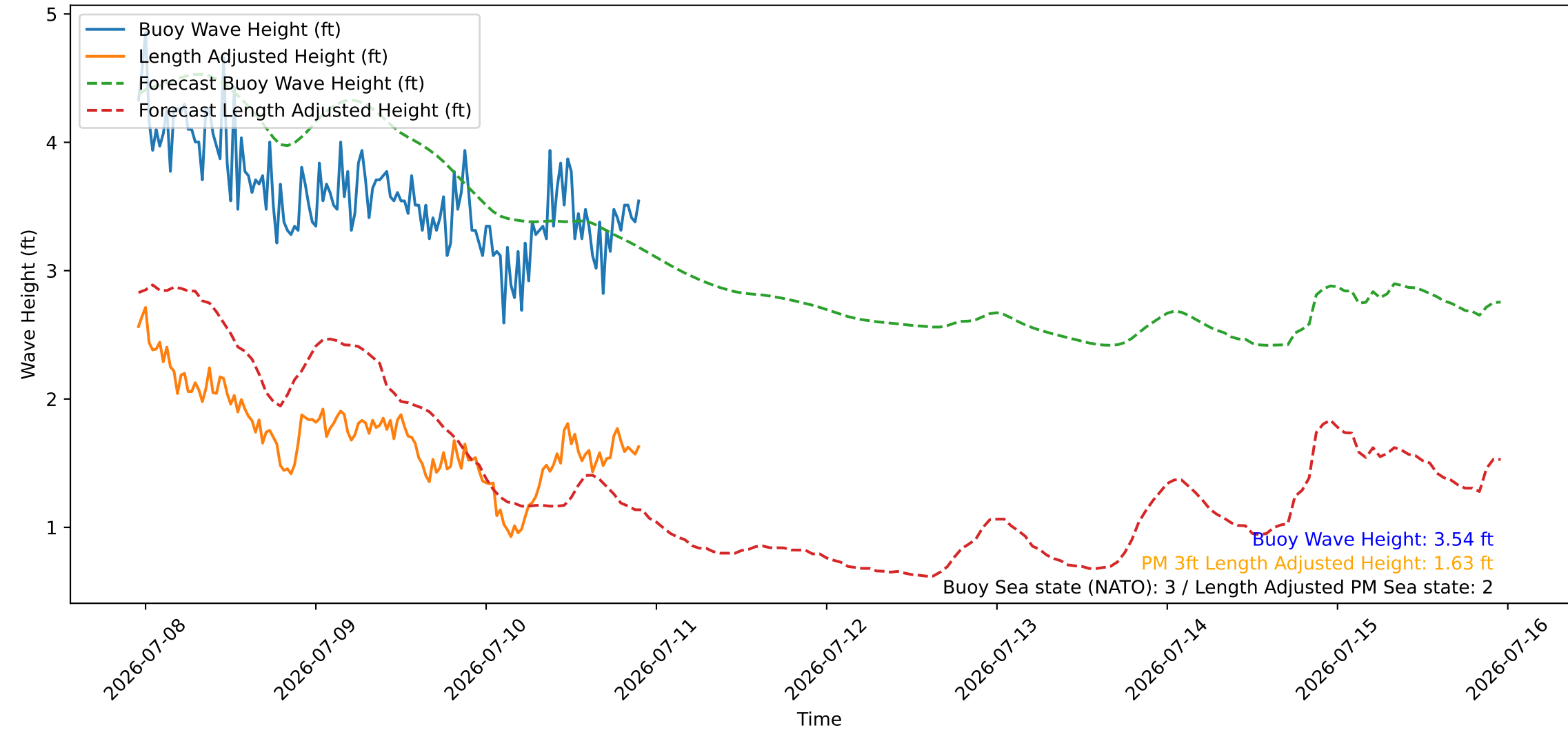
Wave Heights over Time for Red Beach at 2026-07-10 22:40:46
