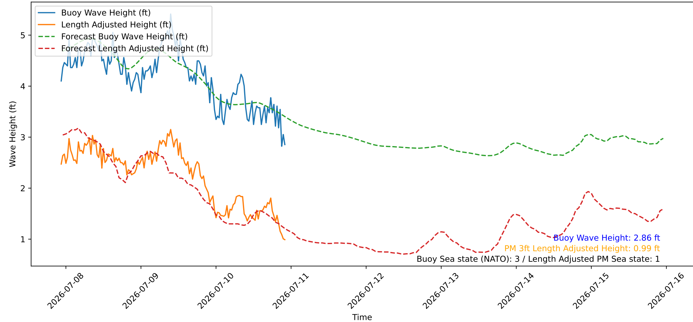
Wave Heights over Time for Oceanside Harbor at 2026-07-10 22:40:26
