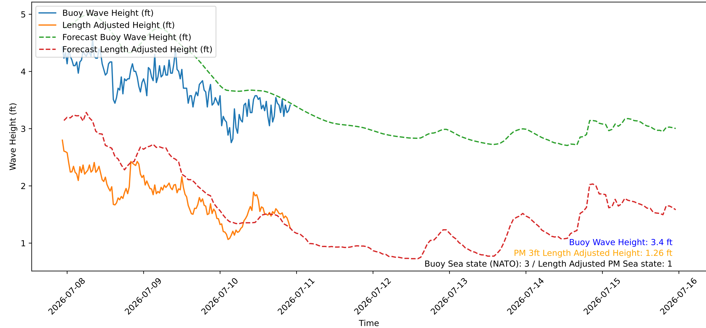
Wave Heights over Time for Green Beach at 2026-07-10 22:41:08
