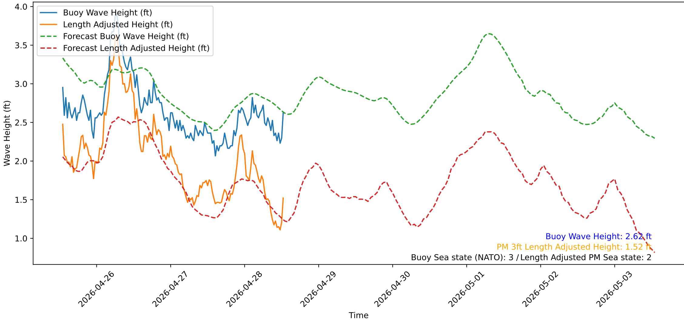
Wave Heights over Time for Oceanside Harbor at 2026-04-28 13:10:31
