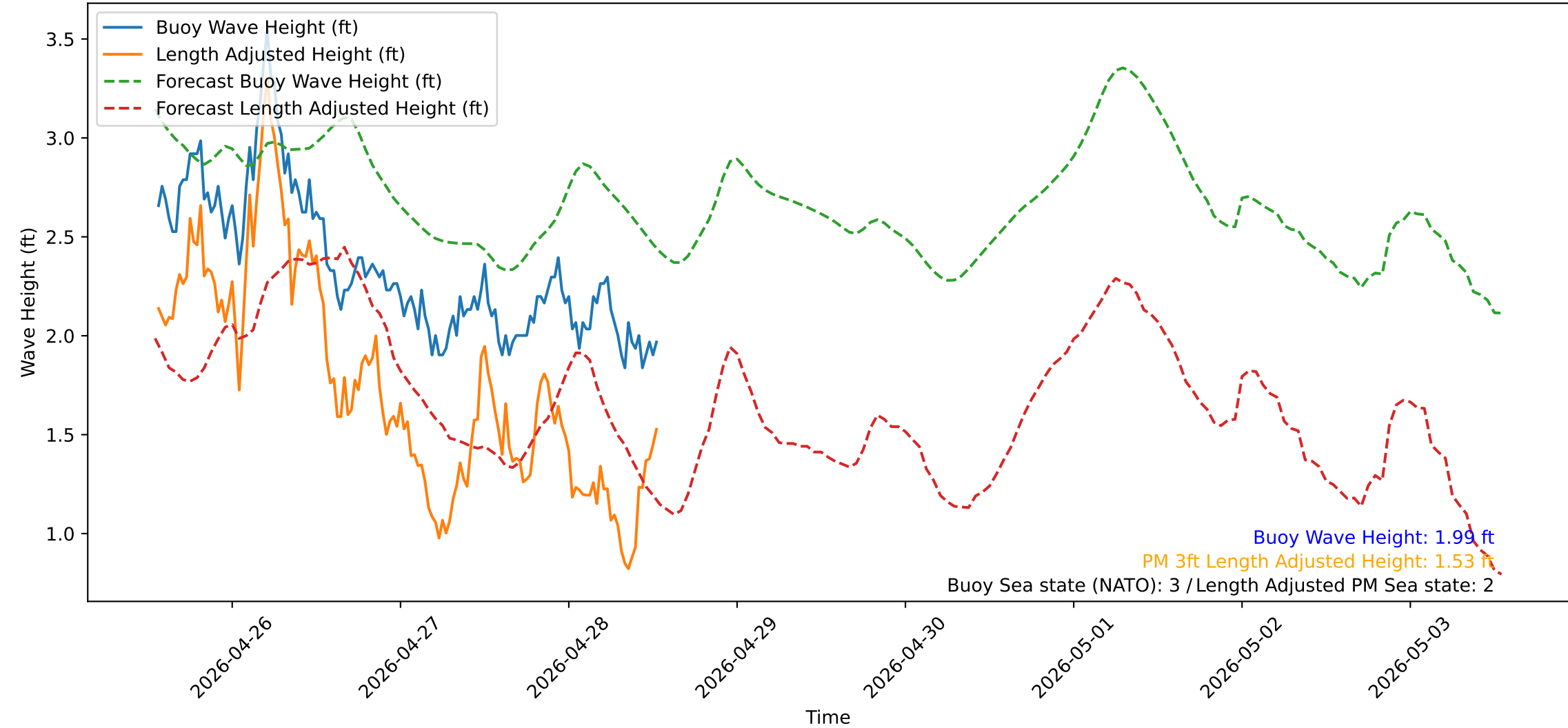
Wave Heights over Time for Red Beach at 2026-04-28 13:10:50
