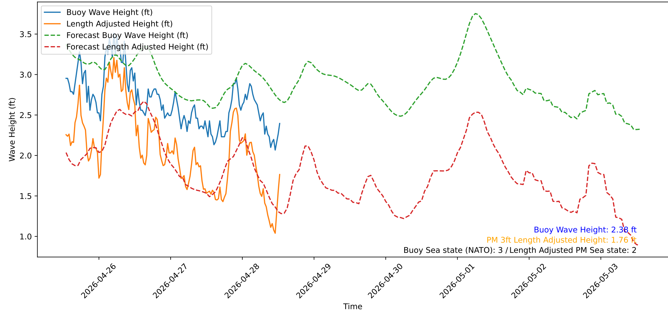
Wave Heights over Time for Green Beach at 2026-04-28 13:11:13
