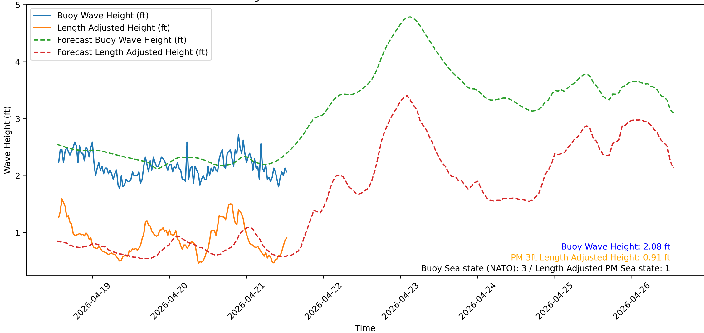
Wave Heights over Time for Red Beach at 2026-04-21 13:10:51
