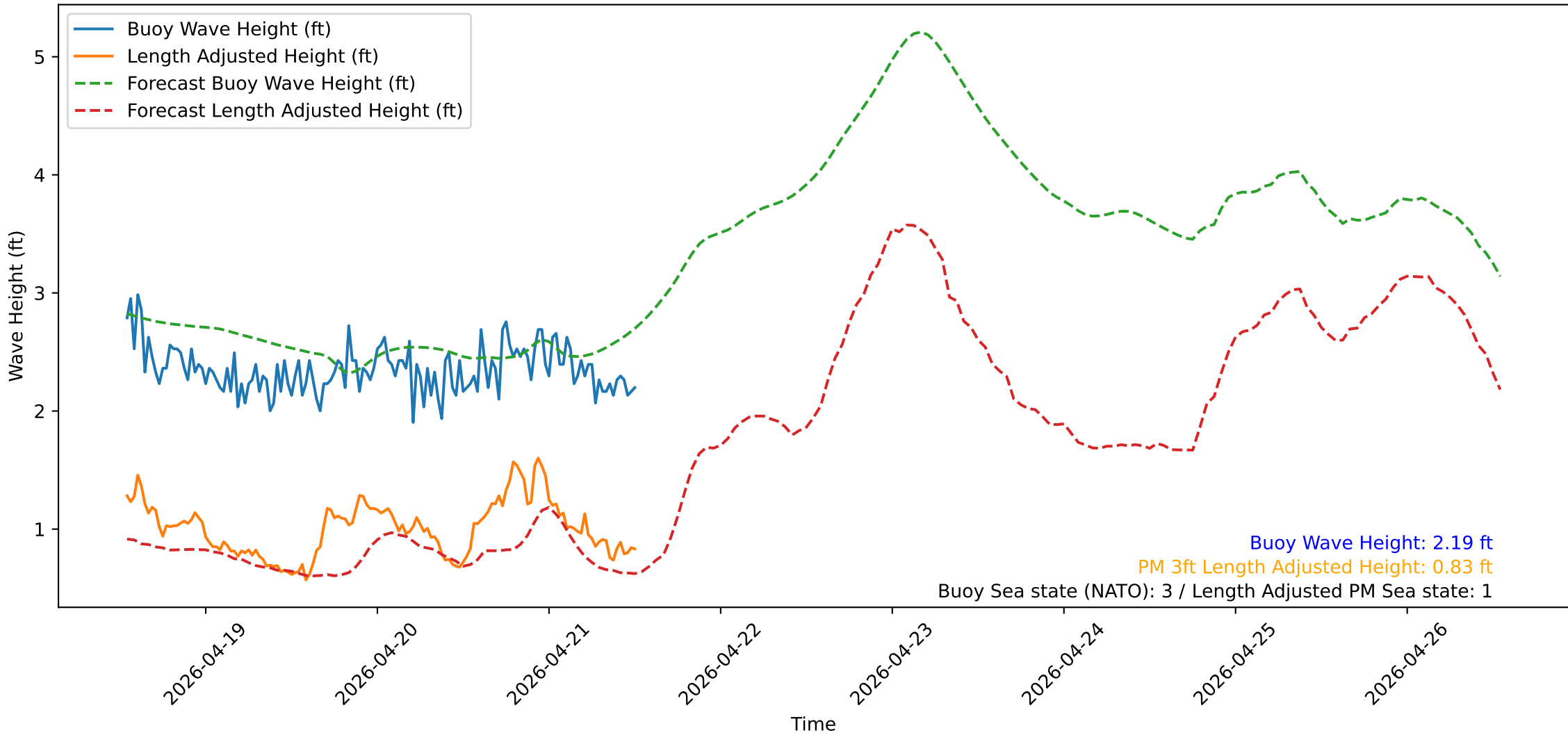
Wave Heights over Time for Oceanside Harbor at 2026-04-21 13:10:32
