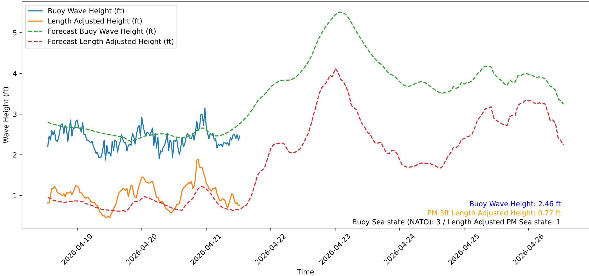
Wave Heights over Time for Green Beach at 2026-04-21 13:11:15
