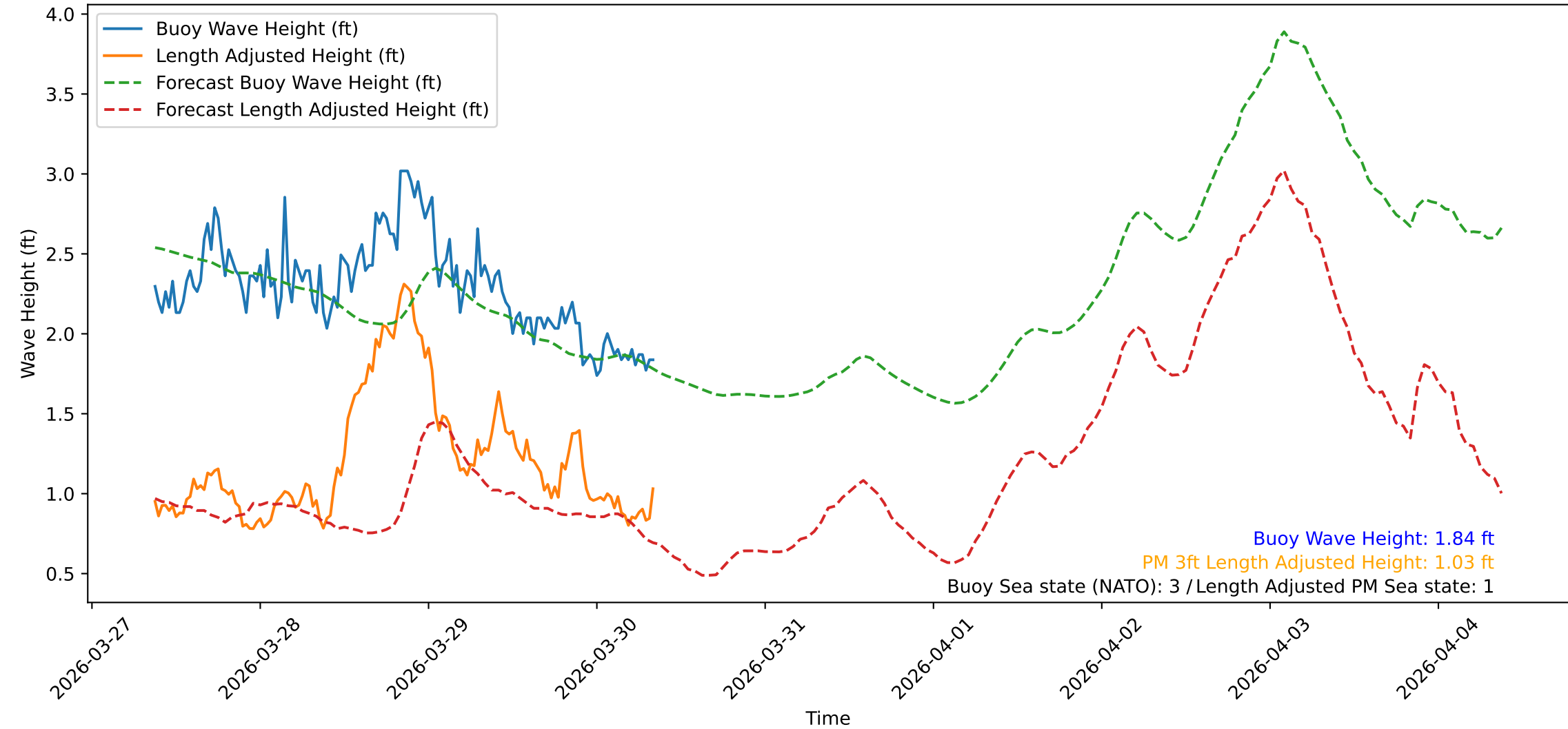
Wave Heights over Time for Red Beach at 2026-03-30 08:40:48
