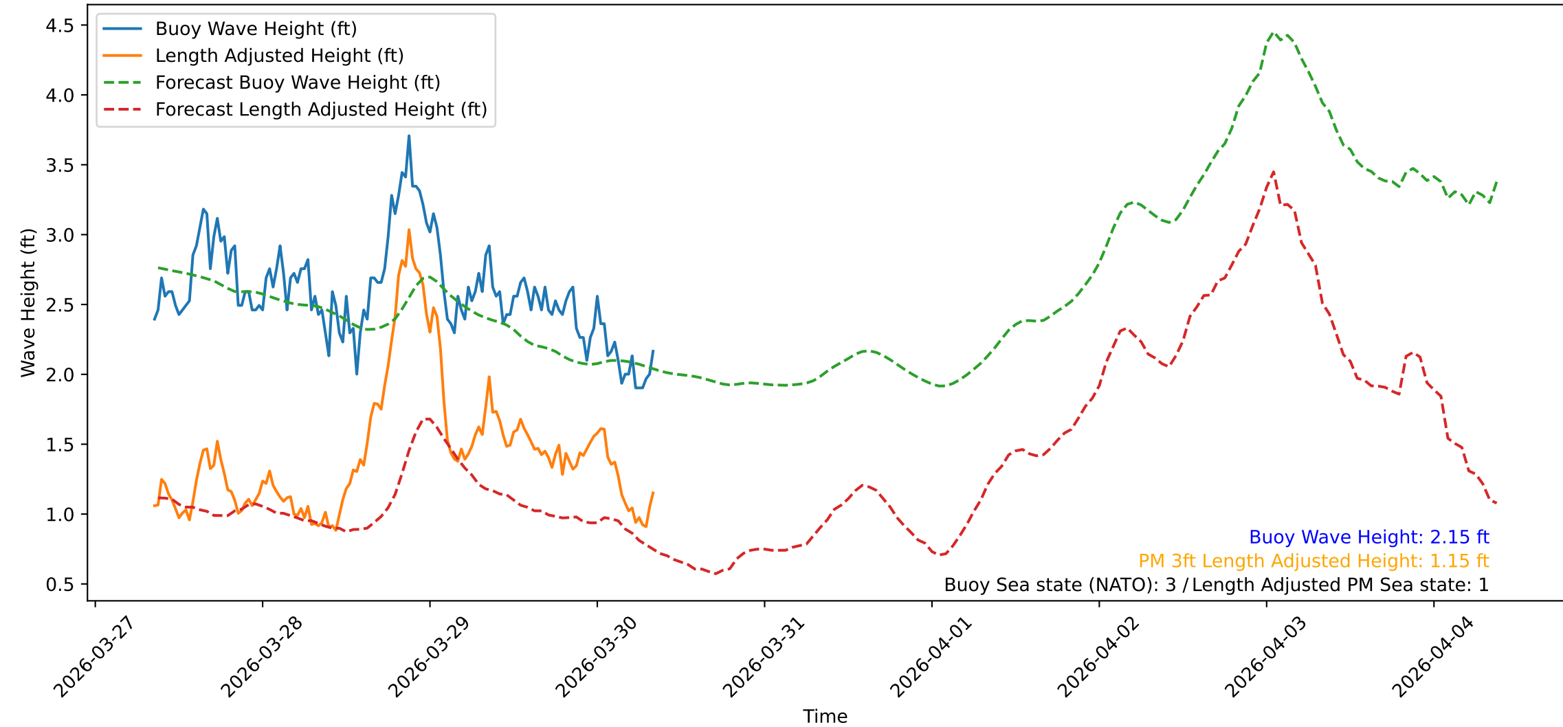
Wave Heights over Time for Green Beach at 2026-03-30 08:41:10
