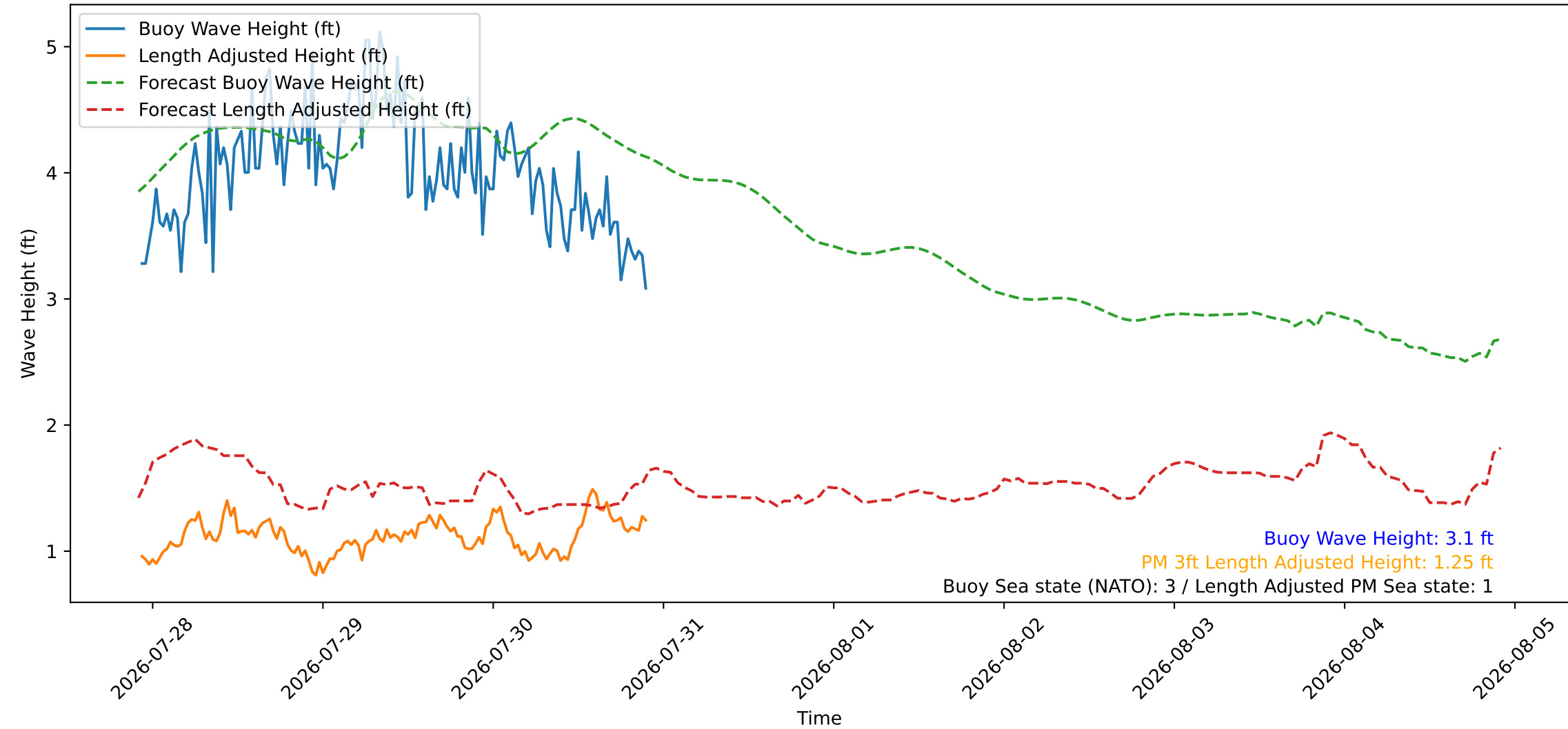
Wave Heights over Time for Red Beach at 2026-07-30 22:20:47
