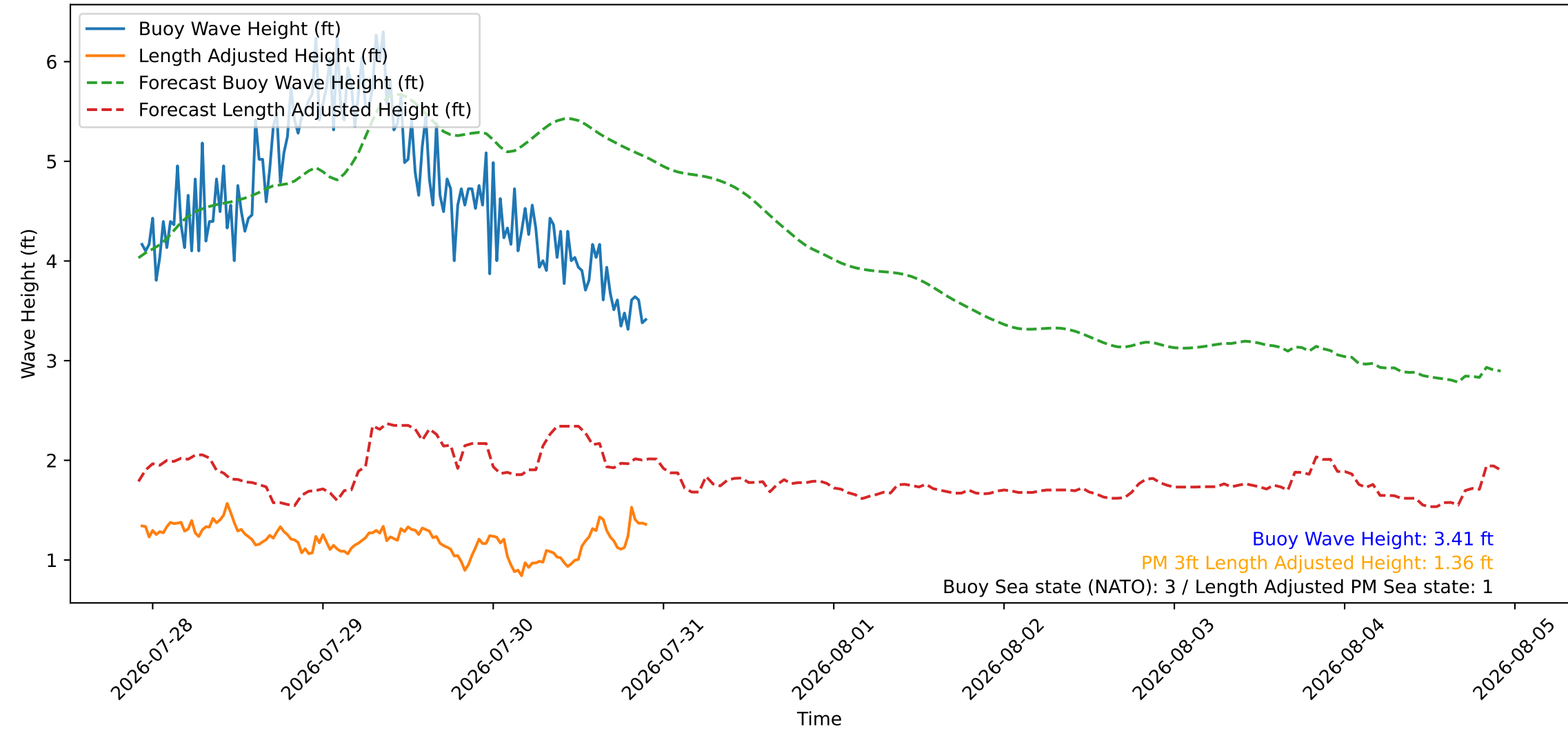
Wave Heights over Time for Green Beach at 2026-07-30 22:21:10
