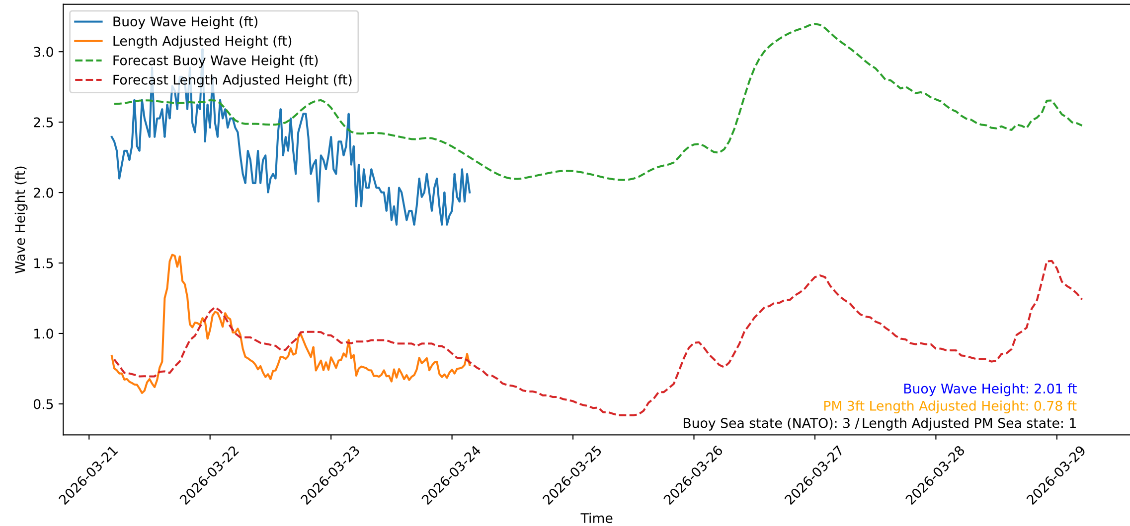
Wave Heights over Time for Oceanside Harbor at 2026-03-24 04:30:31
