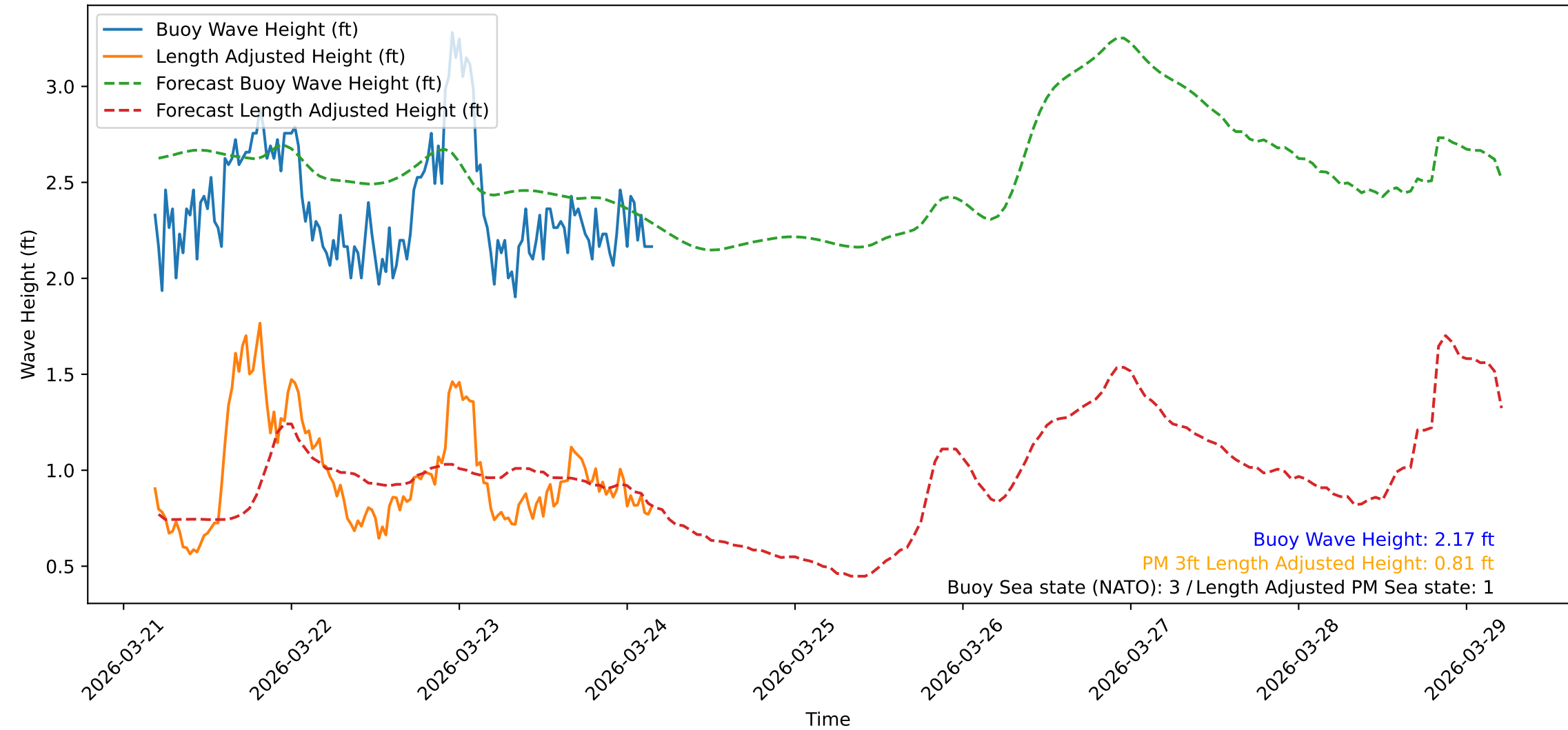
Wave Heights over Time for Green Beach at 2026-03-24 04:31:09
