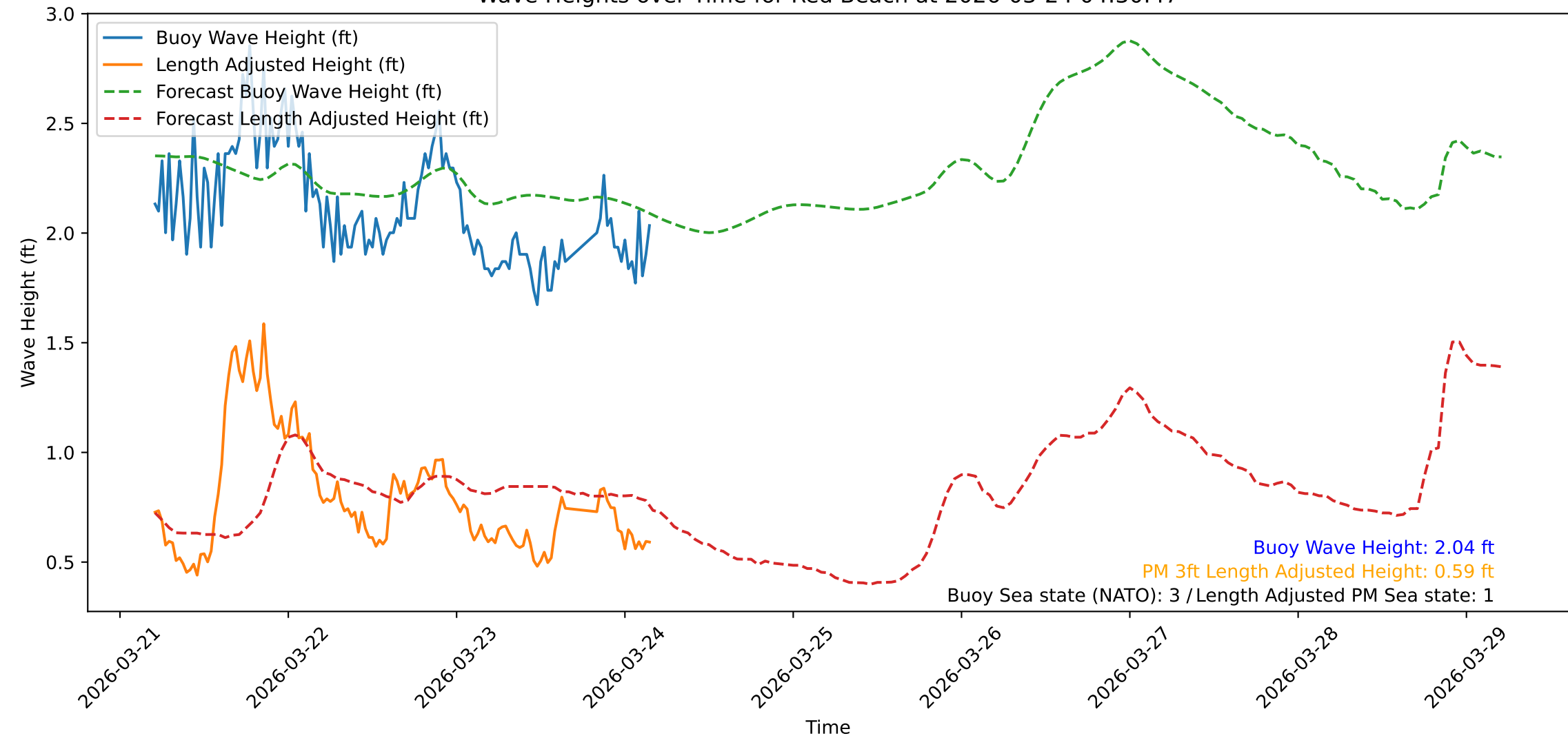
Wave Heights over Time for Red Beach at 2026-03-24 04:30:47
