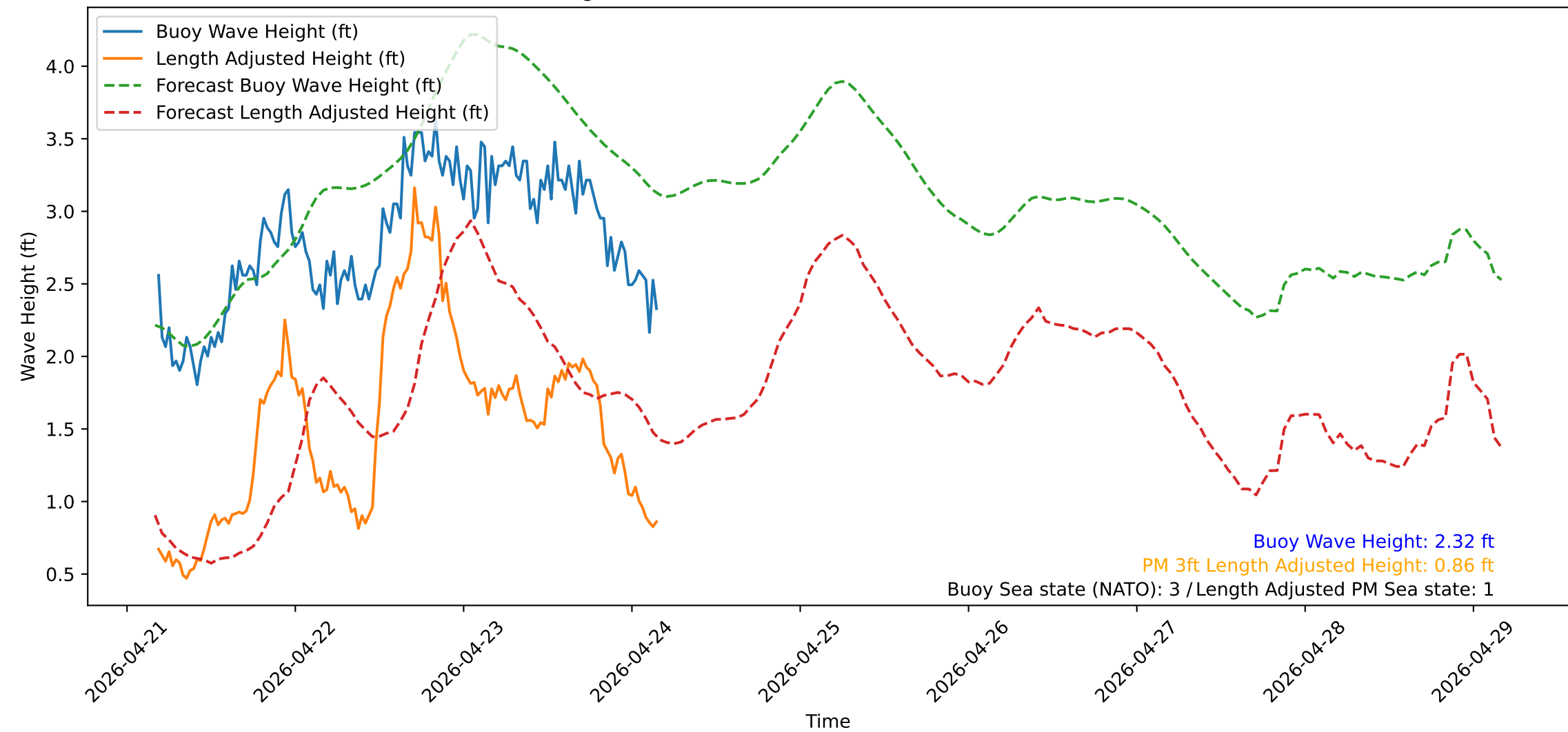
Wave Heights over Time for Red Beach at 2026-04-24 04:20:51
