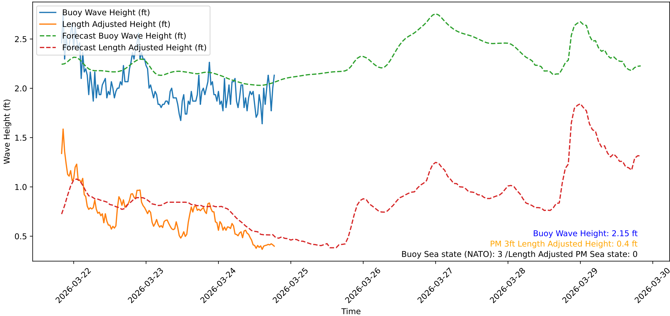
Wave Heights over Time for Red Beach at 2026-03-24 19:40:47
