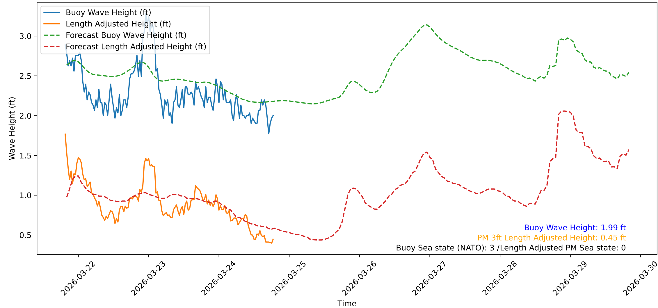
Wave Heights over Time for Green Beach at 2026-03-24 19:41:10
