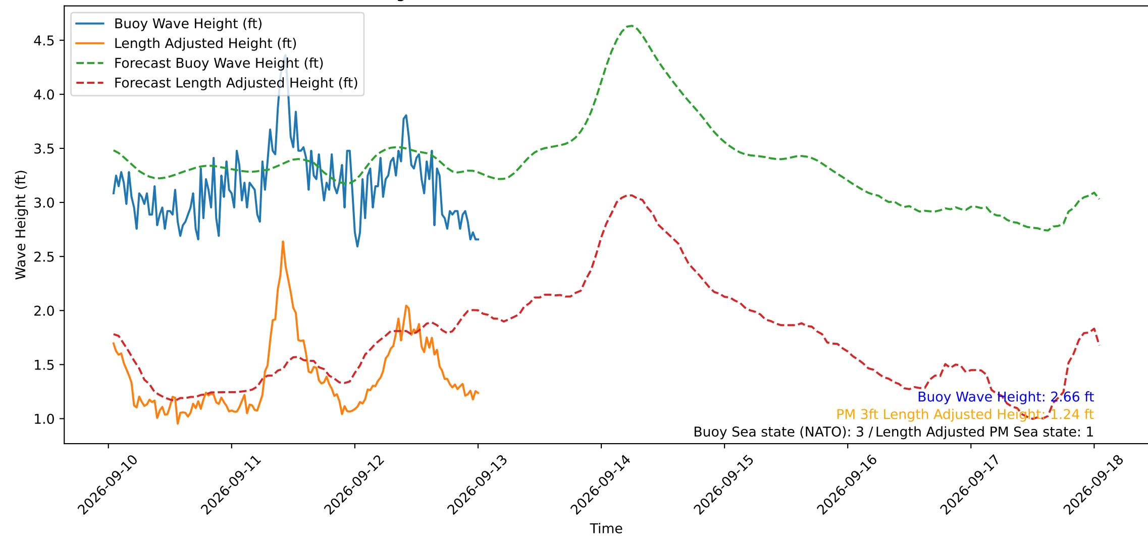
Wave Heights over Time for Oceanside Harbor at 2026-09-13 00:50:30
