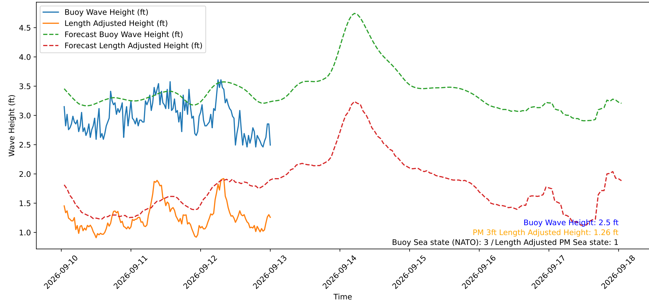
Wave Heights over Time for Green Beach at 2026-09-13 00:51:14
