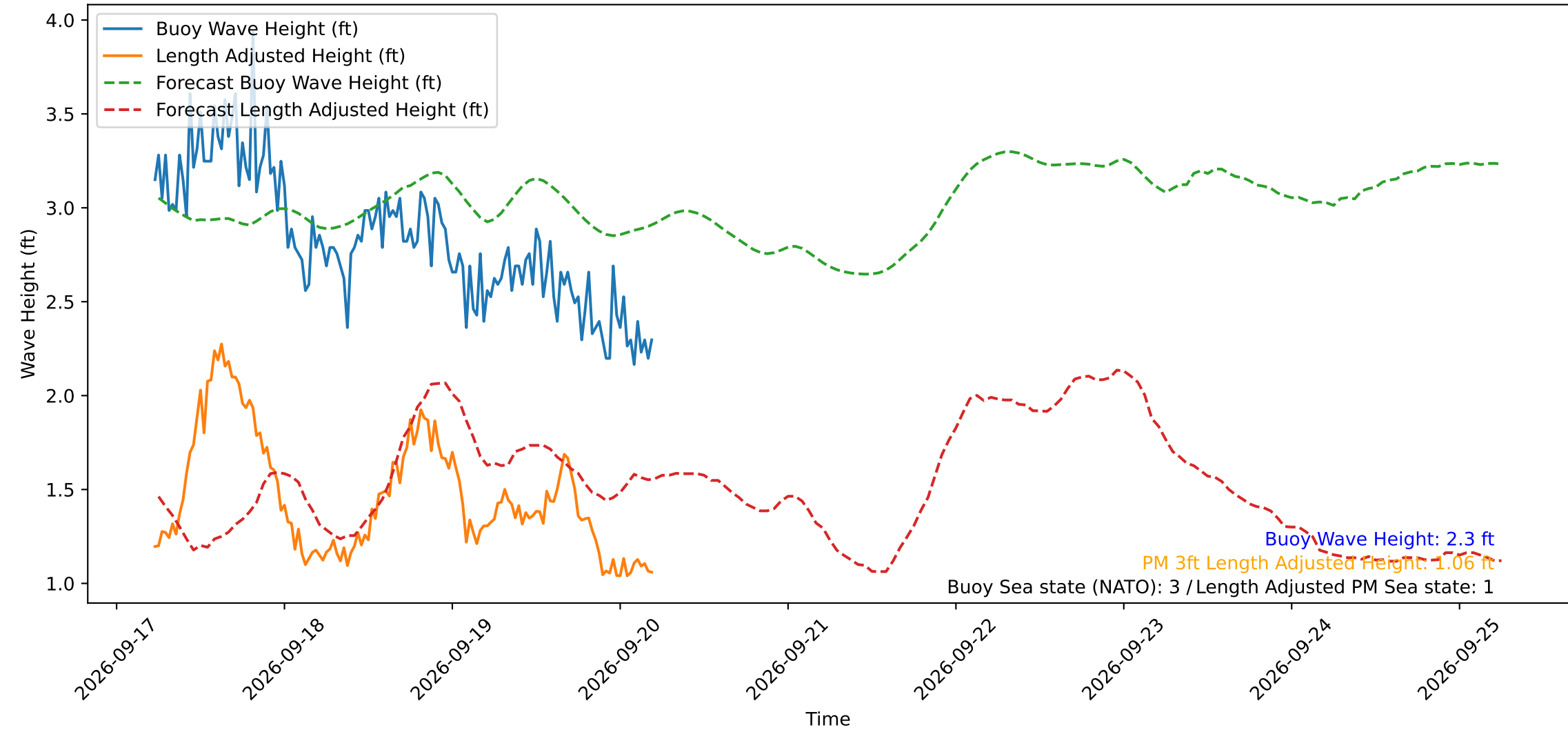
Wave Heights over Time for Oceanside Harbor at 2026-09-20 05:40:29
