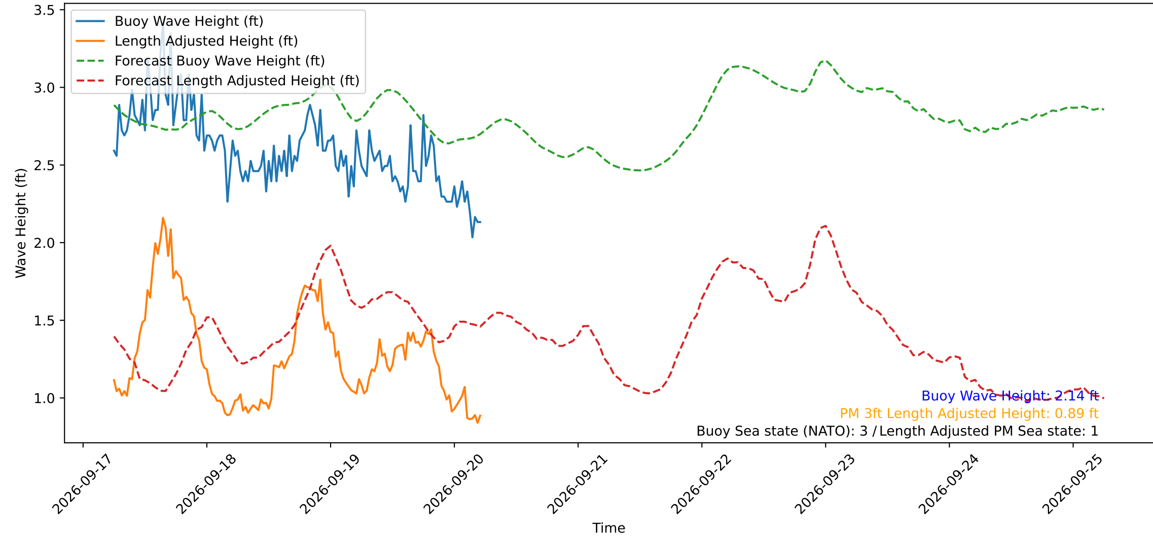
Wave Heights over Time for Red Beach at 2026-09-20 05:40:50
