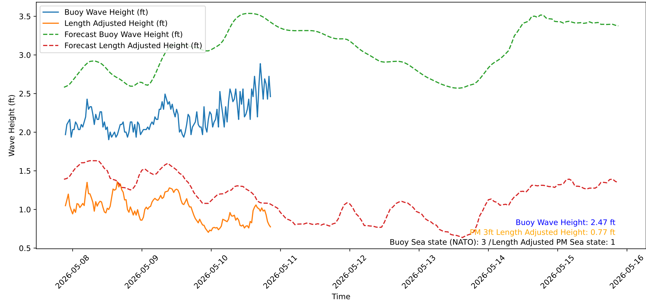
Wave Heights over Time for Red Beach at 2026-05-10 21:10:50
