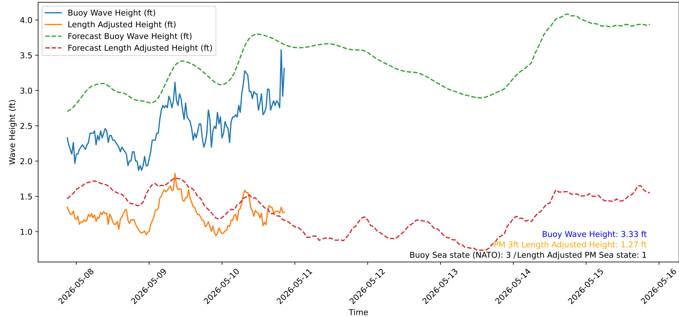
Wave Heights over Time for Oceanside Harbor at 2026-05-10 21:10:31
