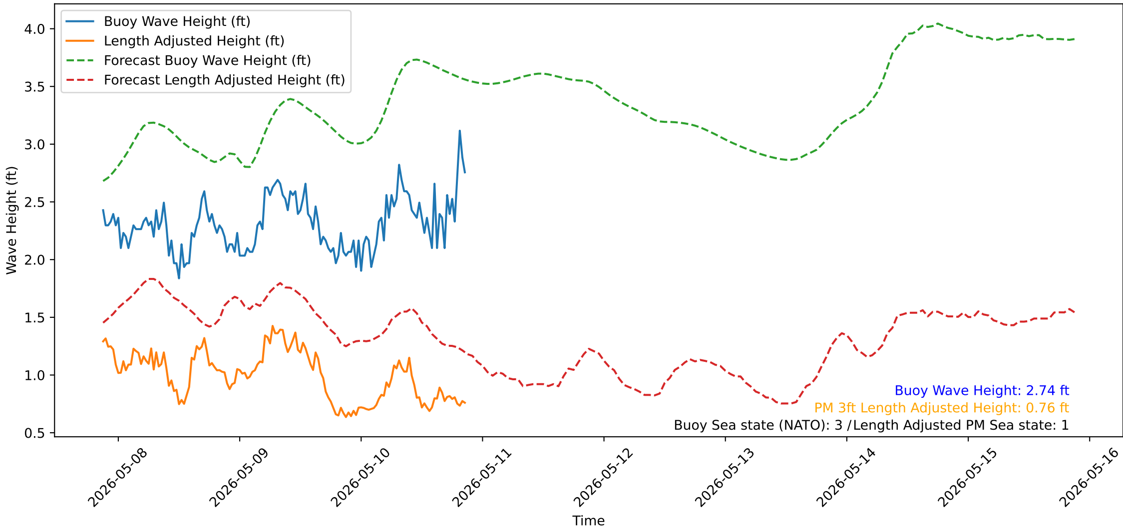
Wave Heights over Time for Green Beach at 2026-05-10 21:11:13
