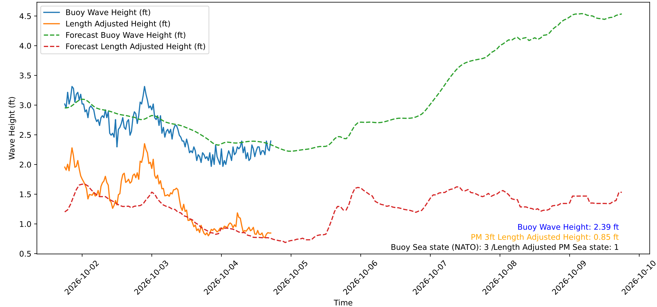
Wave Heights over Time for Oceanside Harbor at 2026-10-04 17:50:29
