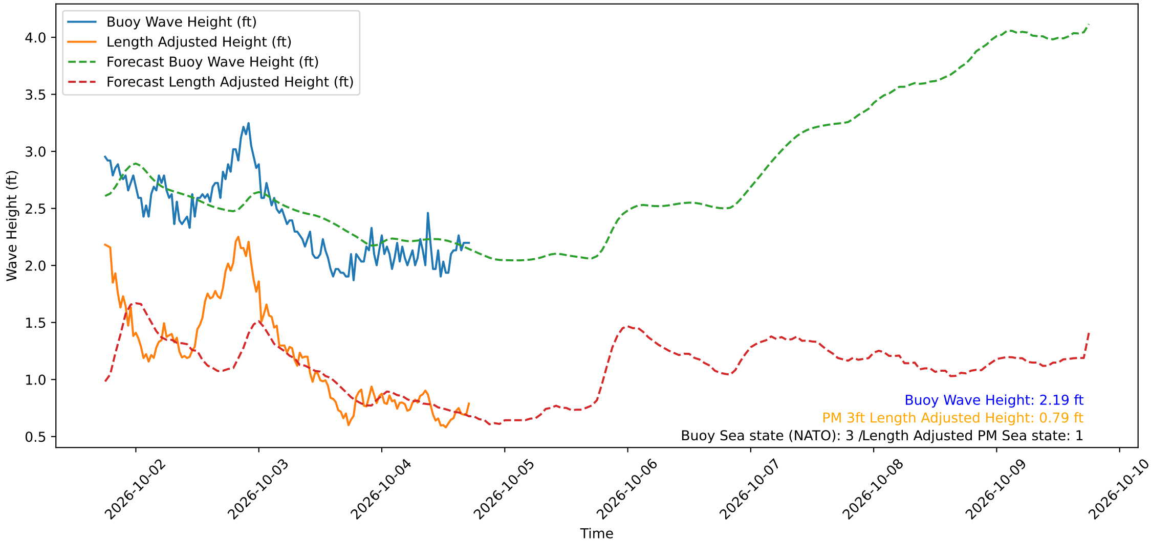
Wave Heights over Time for Red Beach at 2026-10-04 17:50:50
